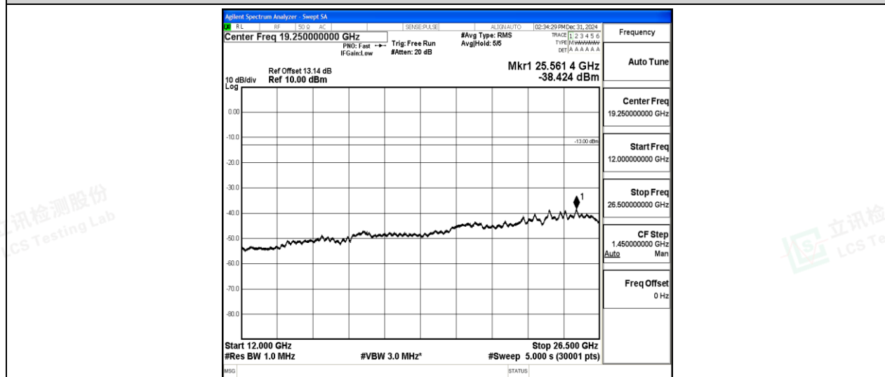
Band5-5MHz-16QAM-20625-1-0-High-12000-26500--38.42-PASS
