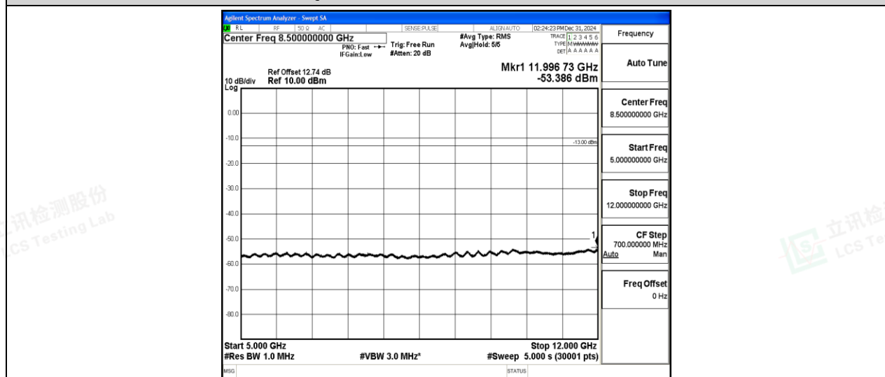
Band5-5MHz-QPSK-20425-1-0-Low-5000-12000--53.39-PASS
