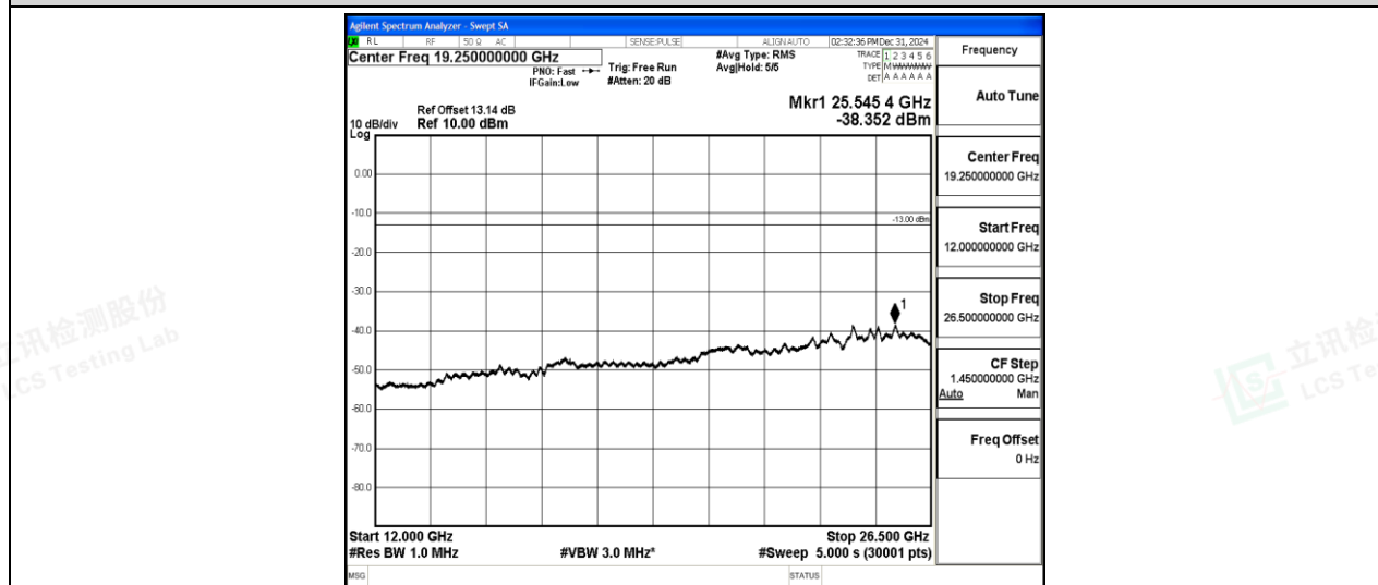
Band5-5MHz-QPSK-20625-1-0-High-12000-26500--38.35-PASS
