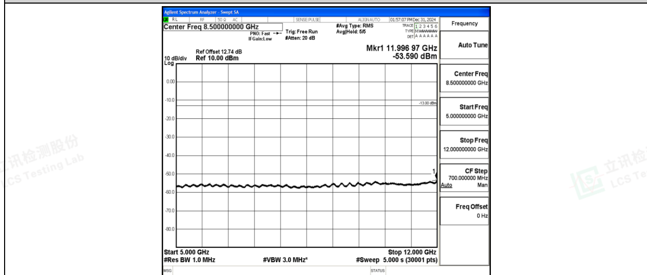
Band5-3MHz-16QAM-20415-1-0-Low-5000-12000--53.59-PASS
