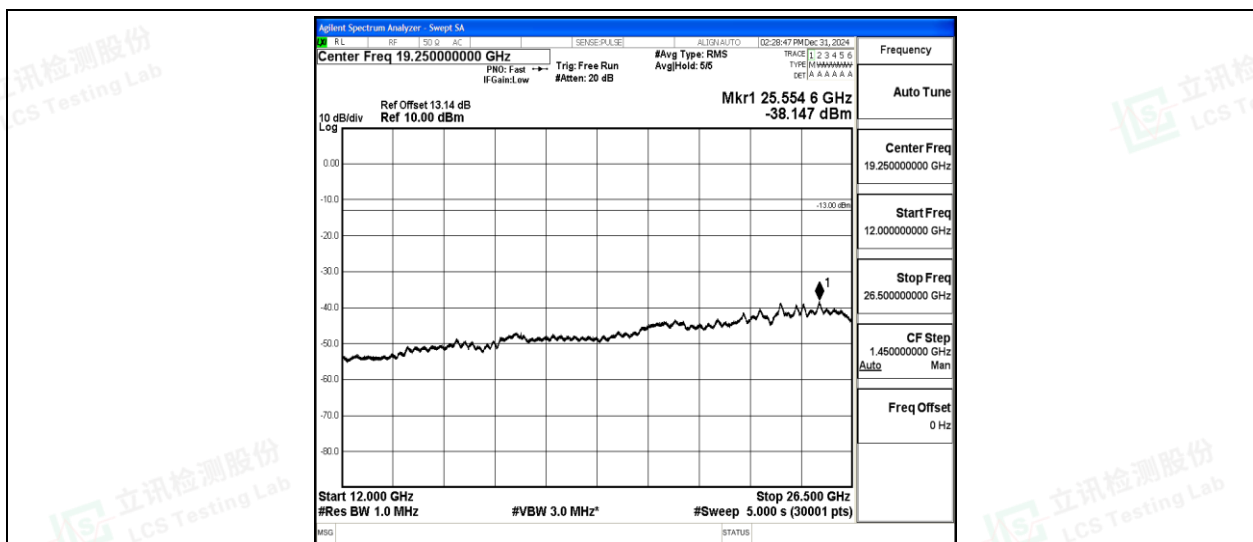
Band5-5MHz-QPSK-20525-1-0-Low-12000-26500--38.15-PASS
