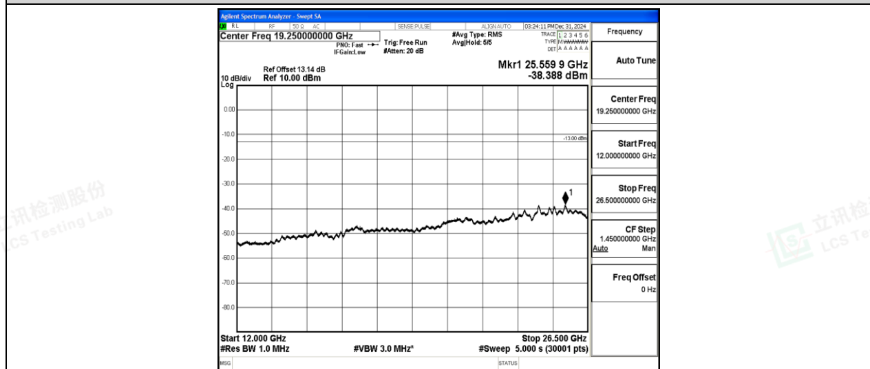
Band5-10MHz-16QAM-20600-1-0-High-12000-26500--38.39-PASS
