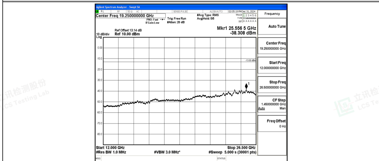
Band5-3MHz-16QAM-20635-1-0-High-12000-26500--38.31-PASS
