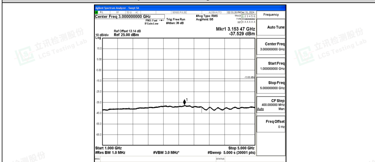
Band5-5MHz-QPSK-20625-1-0-High-1000-5000--37.53-PASS
