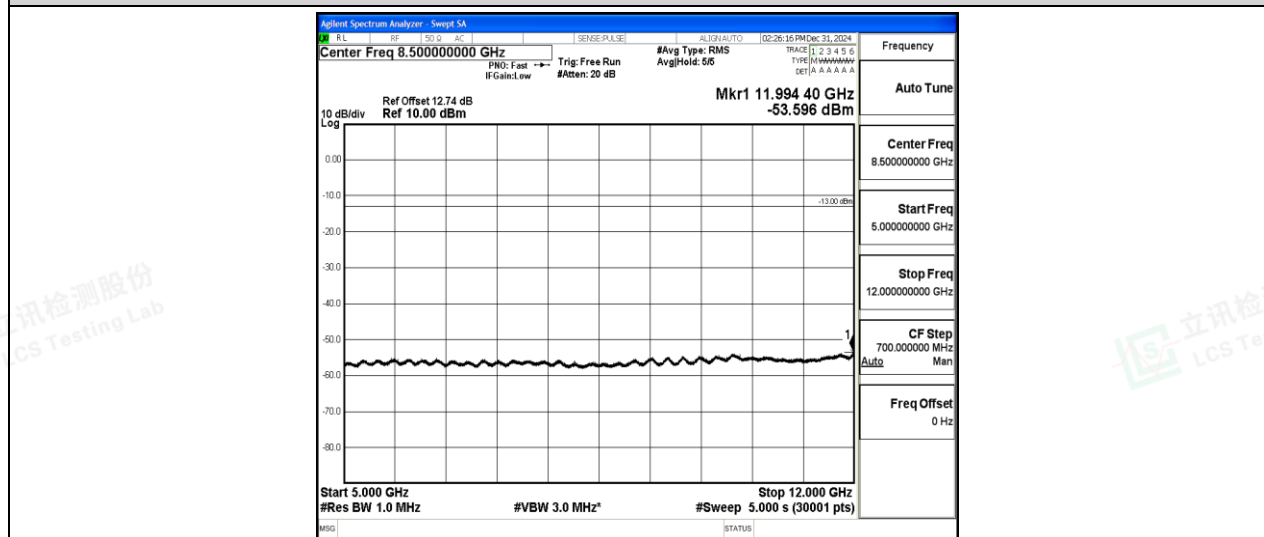
Band5-5MHz-16QAM-20425-1-0-Low-5000-12000--53.6-PASS
