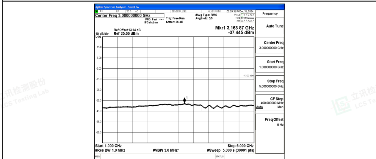
Band5-5MHz-16QAM-20525-1-0-Low-1000-5000--37.45-PASS
