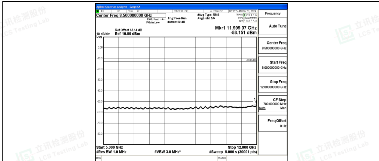
Band5-5MHz-16QAM-20625-1-0-High-5000-12000--53.15-PASS
