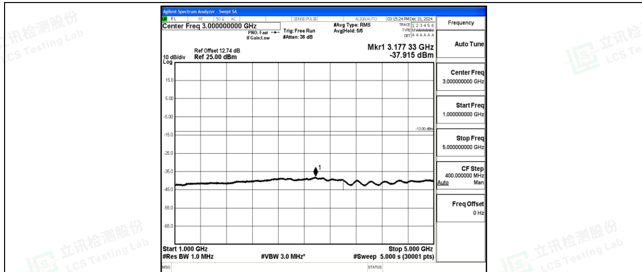
Band5-10MHz-16QAM-20450-1-0-Low-1000-5000--37.92-PASS
