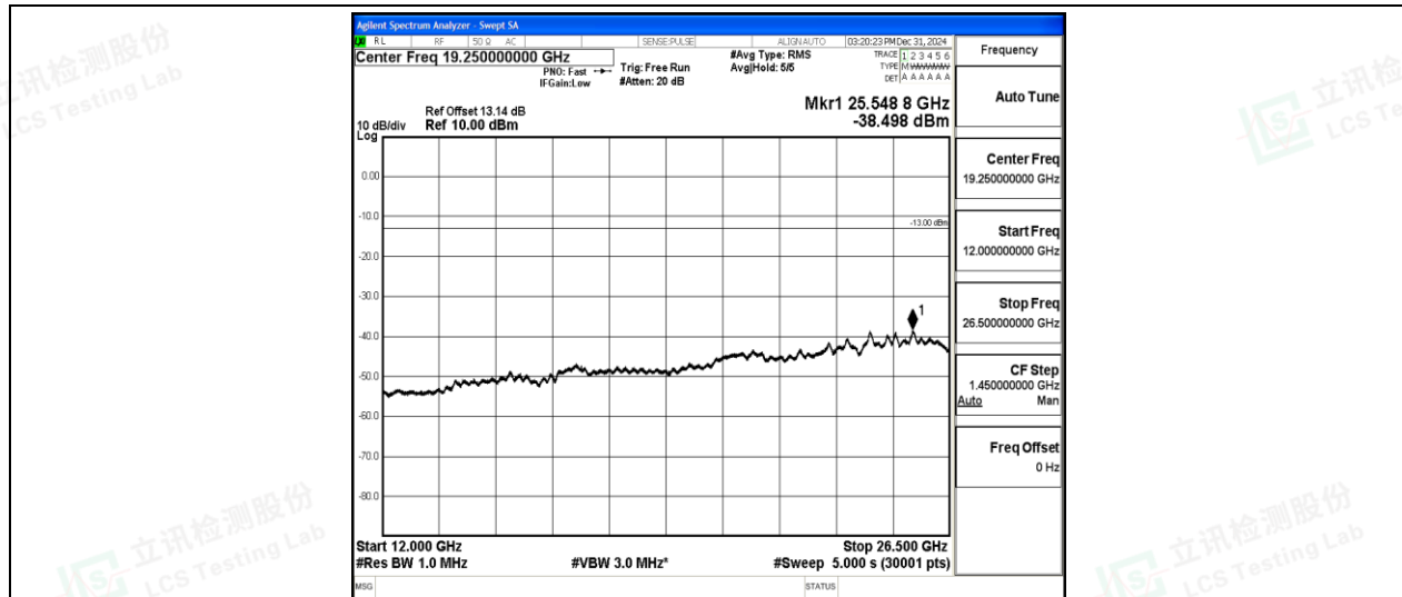
Band5-10MHz-16QAM-20525-1-0-Low-12000-26500--38.5-PASS
