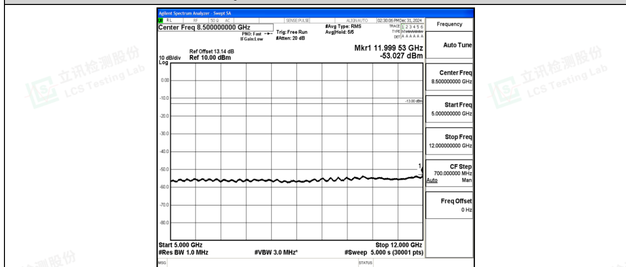
Band5-5MHz-16QAM-20525-1-0-Low-5000-12000--53.03-PASS
