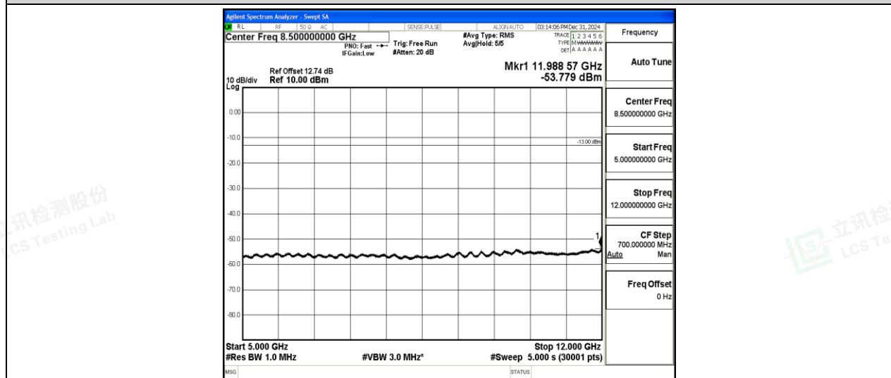
Band5-10MHz-QPSK-20450-1-0-Low-5000-12000--53.78-PASS
