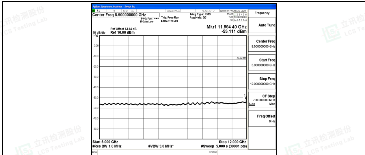
Band5-3MHz-16QAM-20635-1-0-High-5000-12000--53.11-PASS
