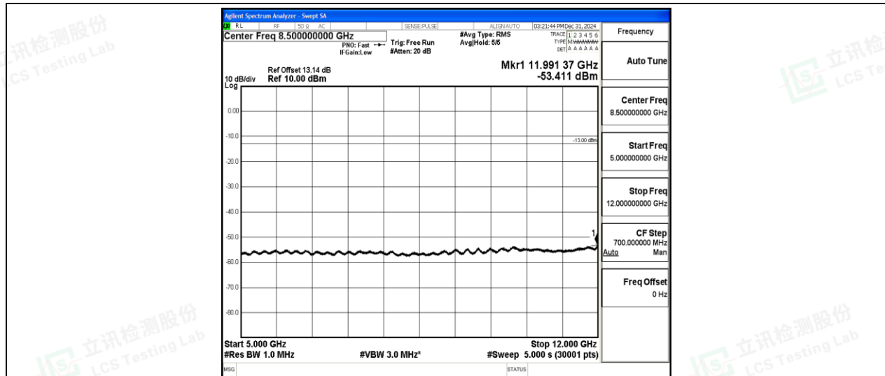
Band5-10MHz-QPSK-20600-1-0-High-5000-12000--53.41-PASS
