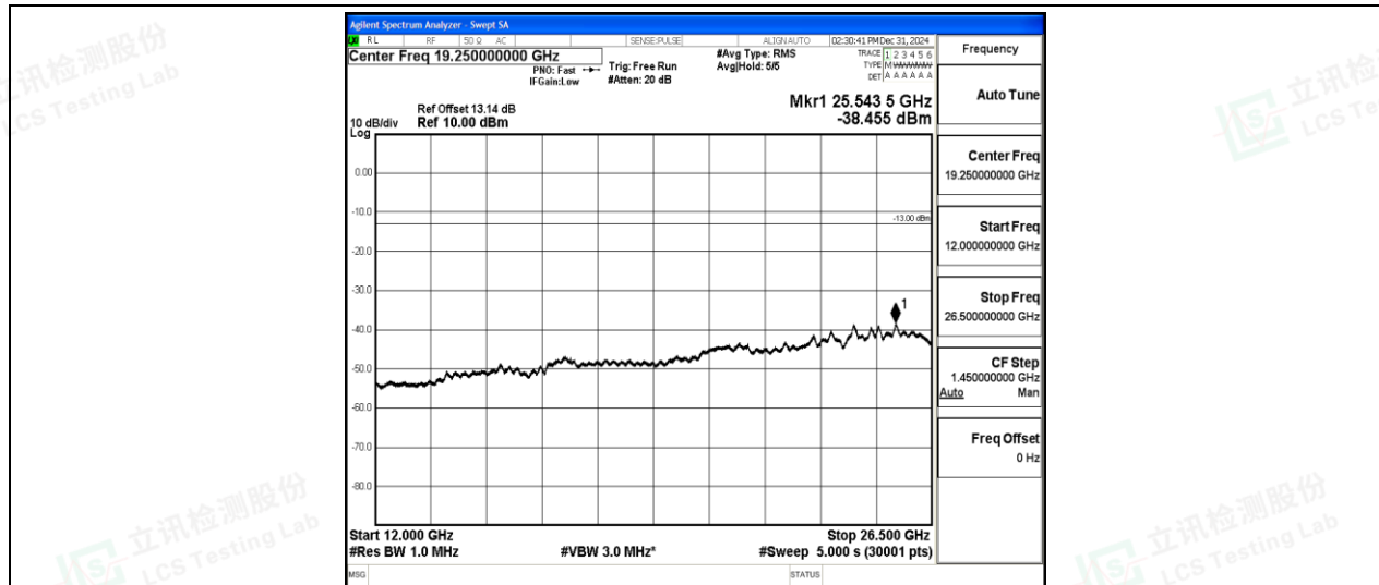
Band5-5MHz-16QAM-20525-1-0-Low-12000-26500--38.46-PASS
