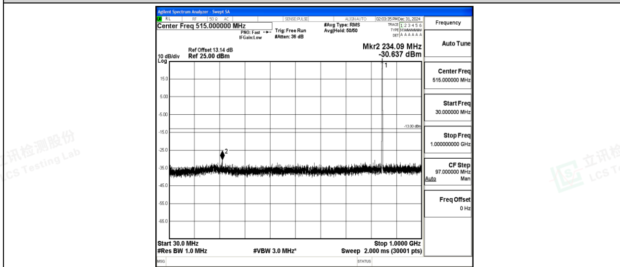
Band5-3MHz-16QAM-20635-1-0-High-30-1000--30.64-PASS
