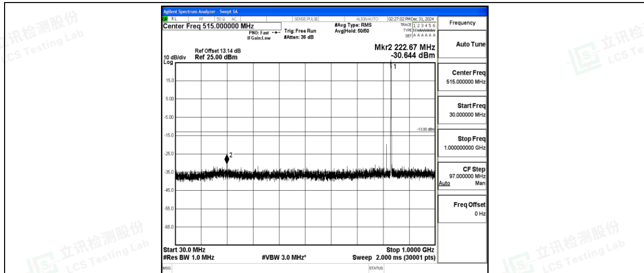
Band5-5MHz-QPSK-20525-1-0-Low-30-1000--30.64-PASS
