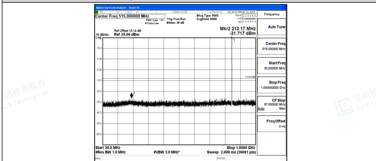
Band5-5MHz-QPSK-20625-1-0-High-30-1000--31.72-PASS
