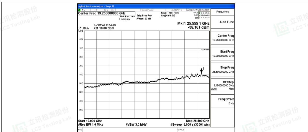
Band5-3MHz-16QAM-20525-1-0-Low-12000-26500--38.16-PASS
