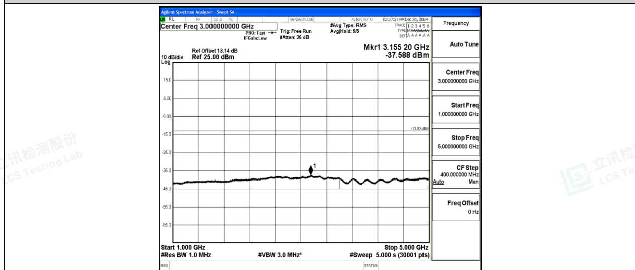
Band5-5MHz-QPSK-20525-1-0-Low-1000-5000--37.59-PASS
