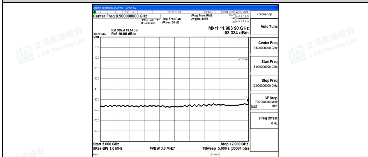
Band5-5MHz-QPSK-20525-1-0-Low-5000-12000--53.33-PASS
