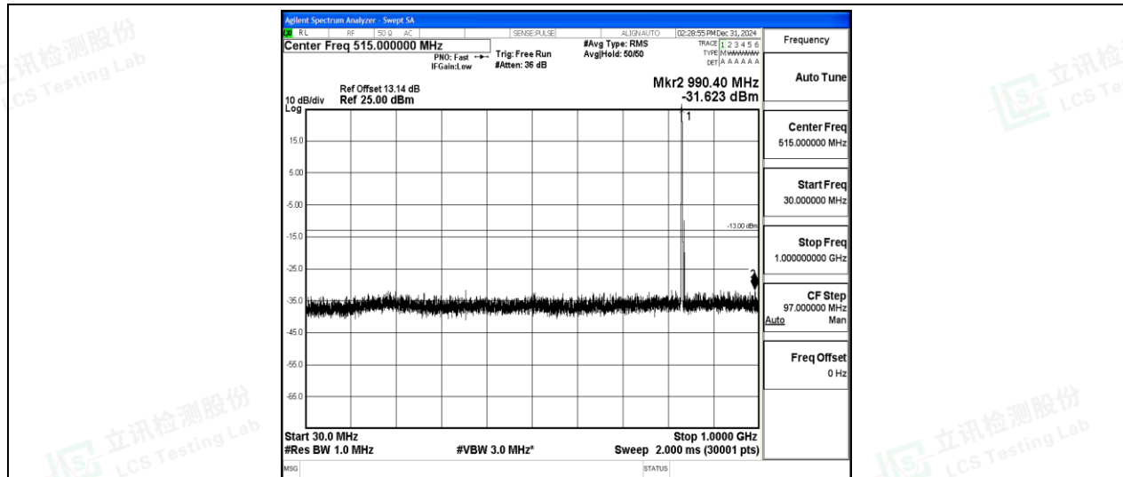
Band5-5MHz-16QAM-20525-1-0-Low-30-1000--31.62-PASS
