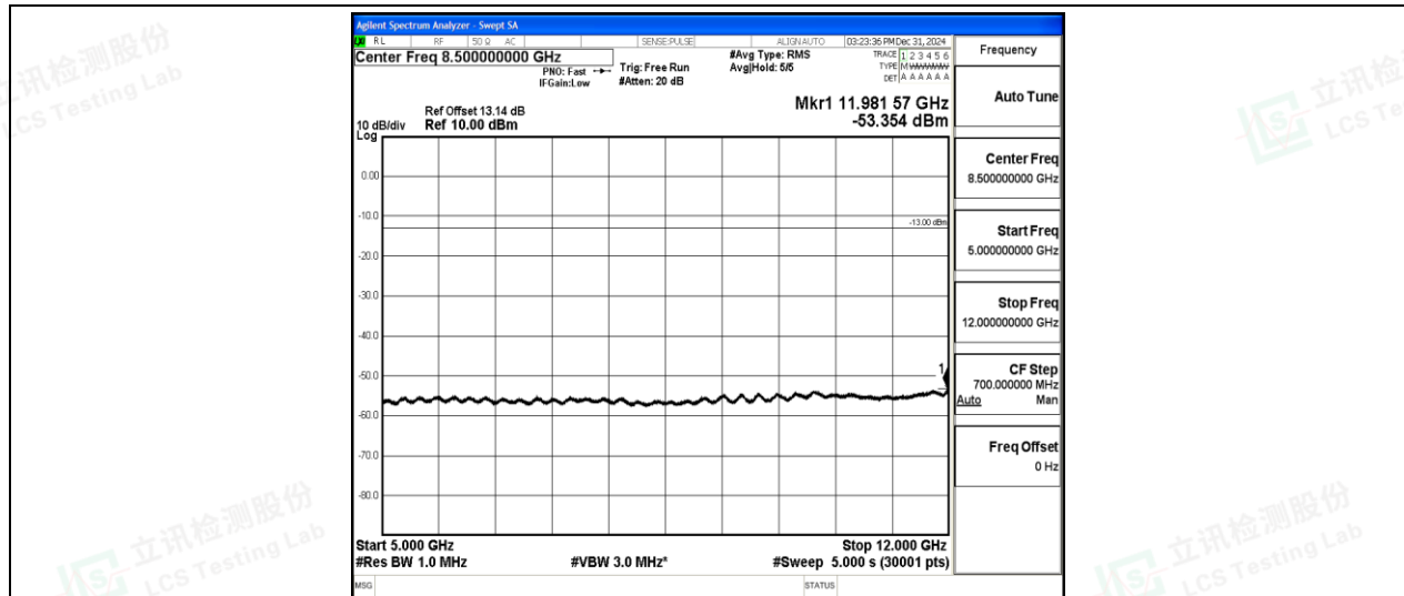
Band5-10MHz-16QAM-20600-1-0-High-5000-12000--53.35-PASS
