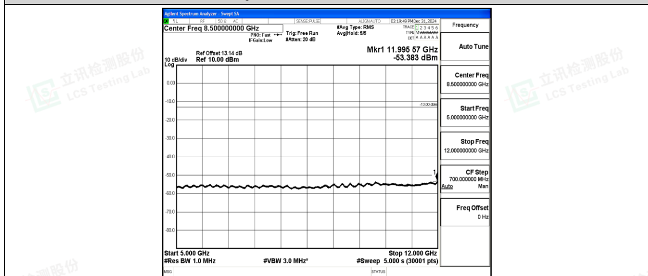
Band5-10MHz-16QAM-20525-1-0-Low-5000-12000--53.38-PASS
