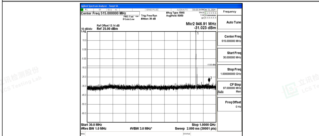
Band5-10MHz-QPSK-20600-1-0-High-30-1000--31.02-PASS
