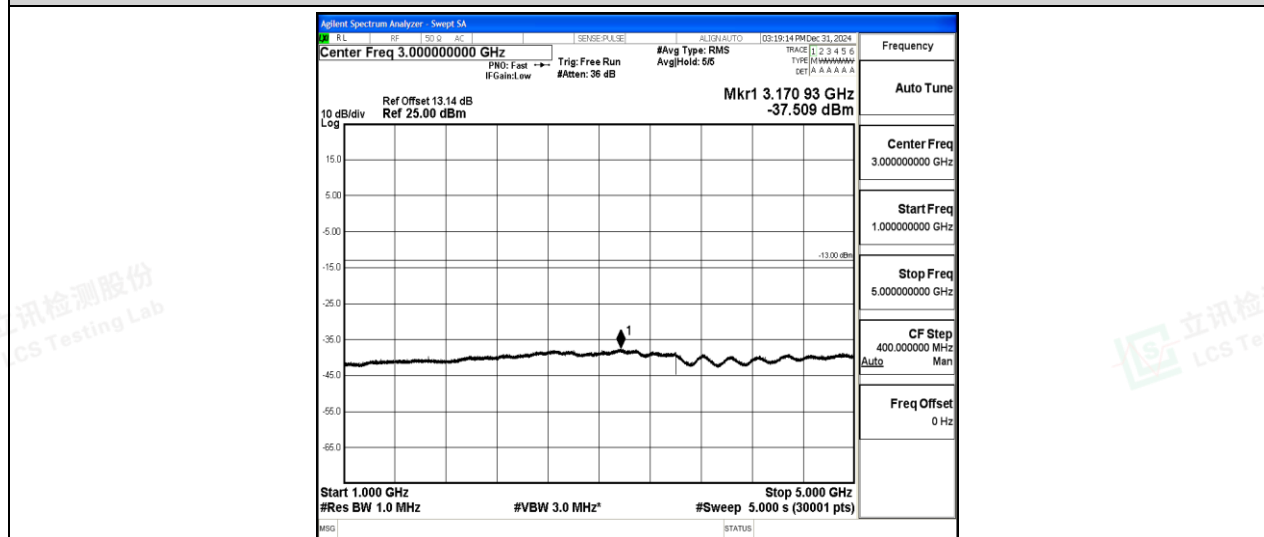
Band5-10MHz-16QAM-20525-1-0-Low-1000-5000--37.51-PASS
