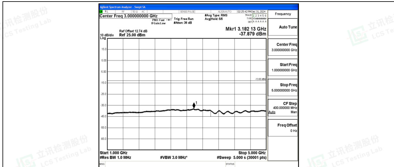
Band5-5MHz-16QAM-20425-1-0-Low-1000-5000--37.88-PASS
