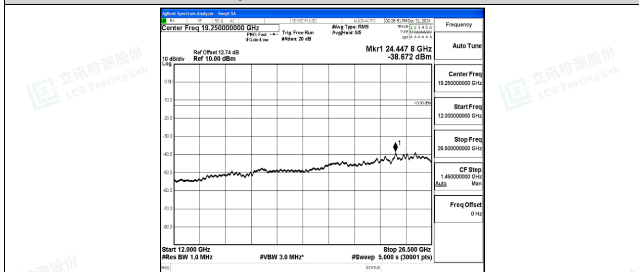
Band5-5MHz-16QAM-20425-1-0-Low-12000-26500--38.67-PASS
