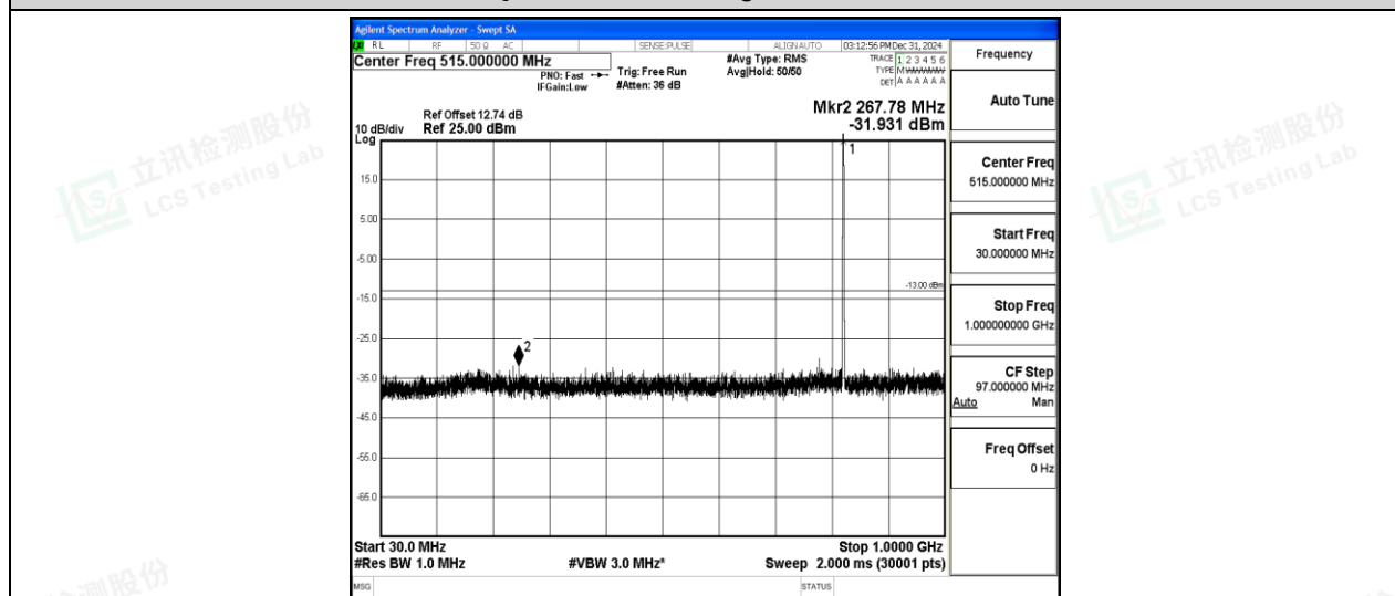
Band5-10MHz-QPSK-20450-1-0-Low-30-1000--31.93-PASS
