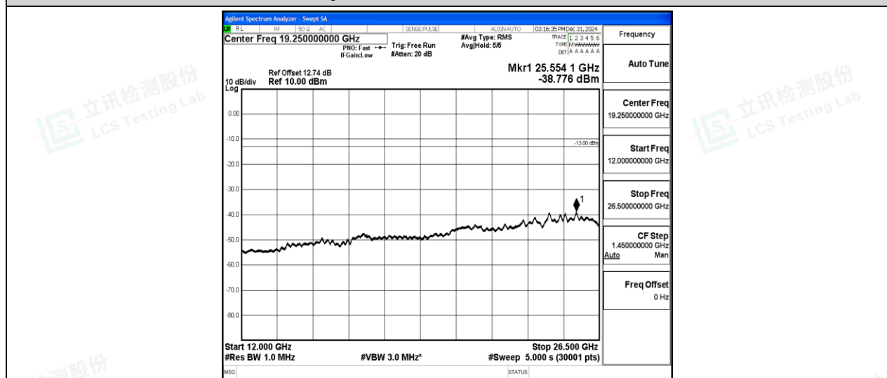
Band5-10MHz-16QAM-20450-1-0-Low-12000-26500--38.78-PASS
