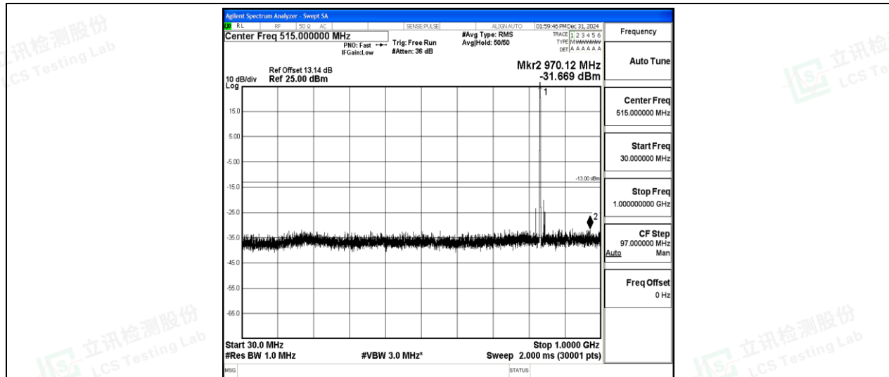
Band5-3MHz-16QAM-20525-1-0-Low-30-1000--31.67-PASS
