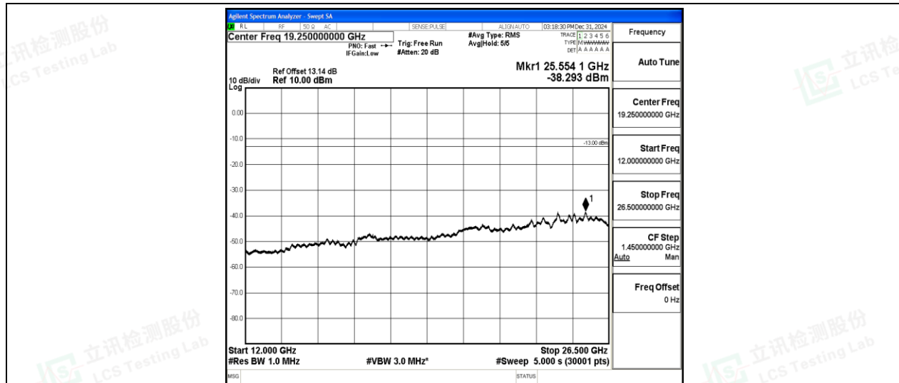
Band5-10MHz-QPSK-20525-1-0-Low-12000-26500--38.29-PASS
