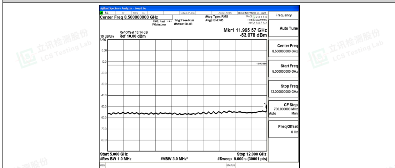
Band5-3MHz-16QAM-20525-1-0-Low-5000-12000--53.08-PASS
