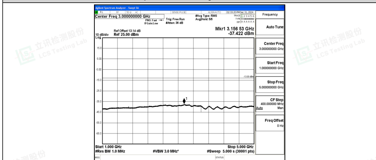
Band5-5MHz-16QAM-20625-1-0-High-1000-5000--37.42-PASS
