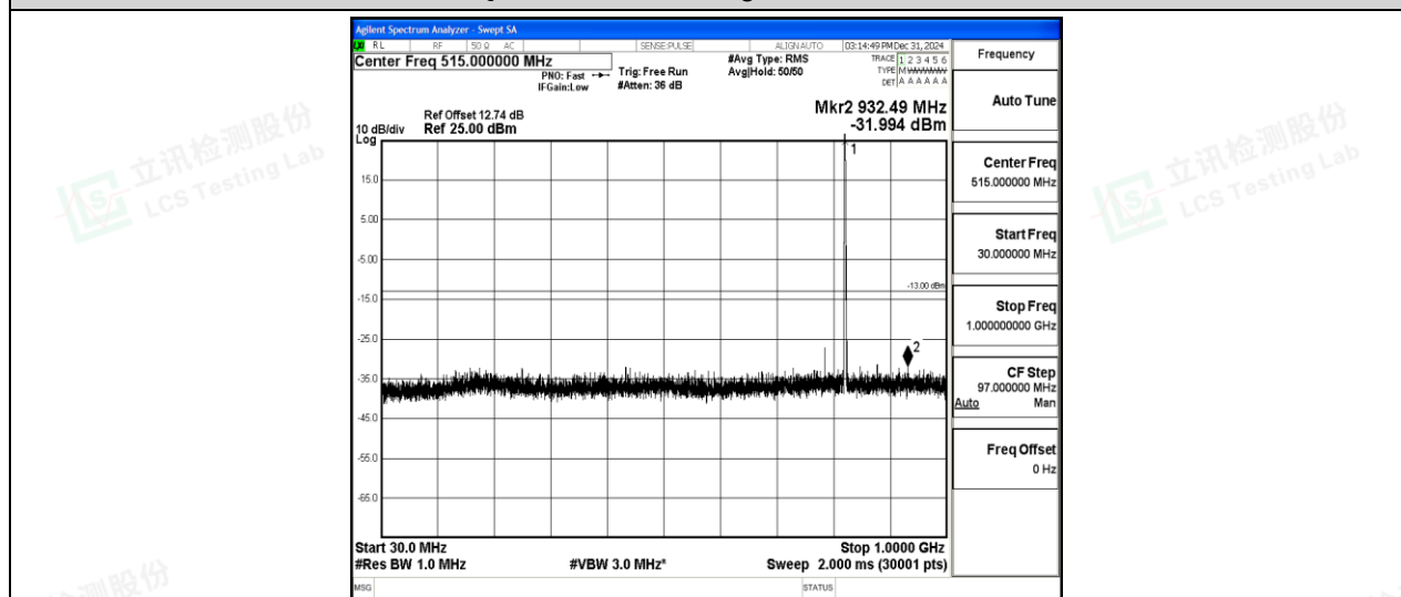
Band5-10MHz-16QAM-20450-1-0-Low-30-1000--31.99-PASS
