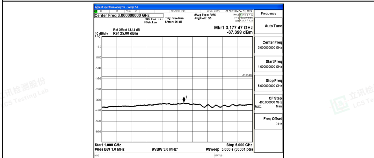
Band5-3MHz-16QAM-20525-1-0-Low-1000-5000--37.4-PASS
