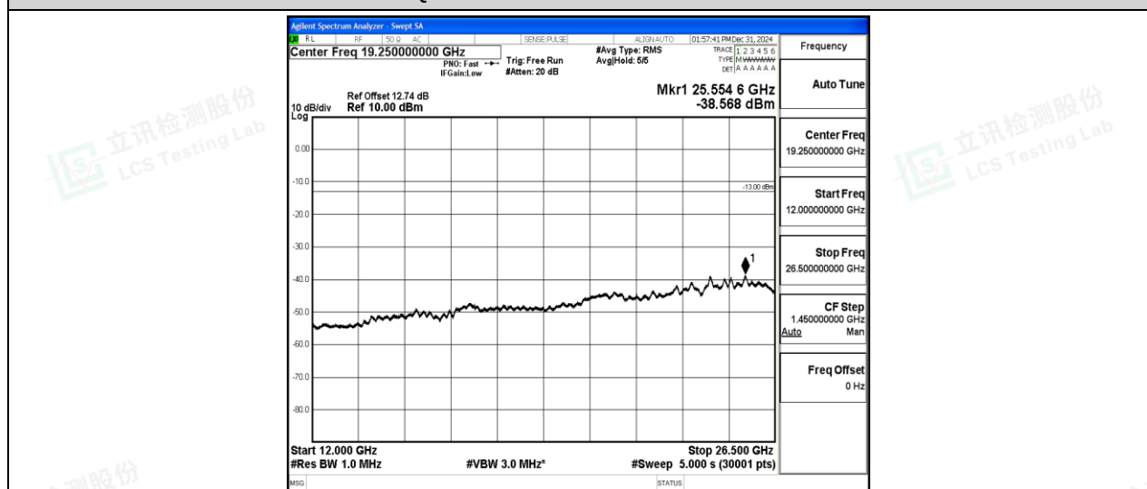
Band5-3MHz-16QAM-20415-1-0-Low-12000-26500--38.57-PASS
