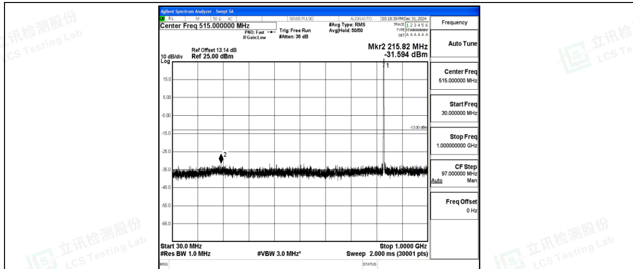
Band5-10MHz-16QAM-20525-1-0-Low-30-1000--31.59-PASS
