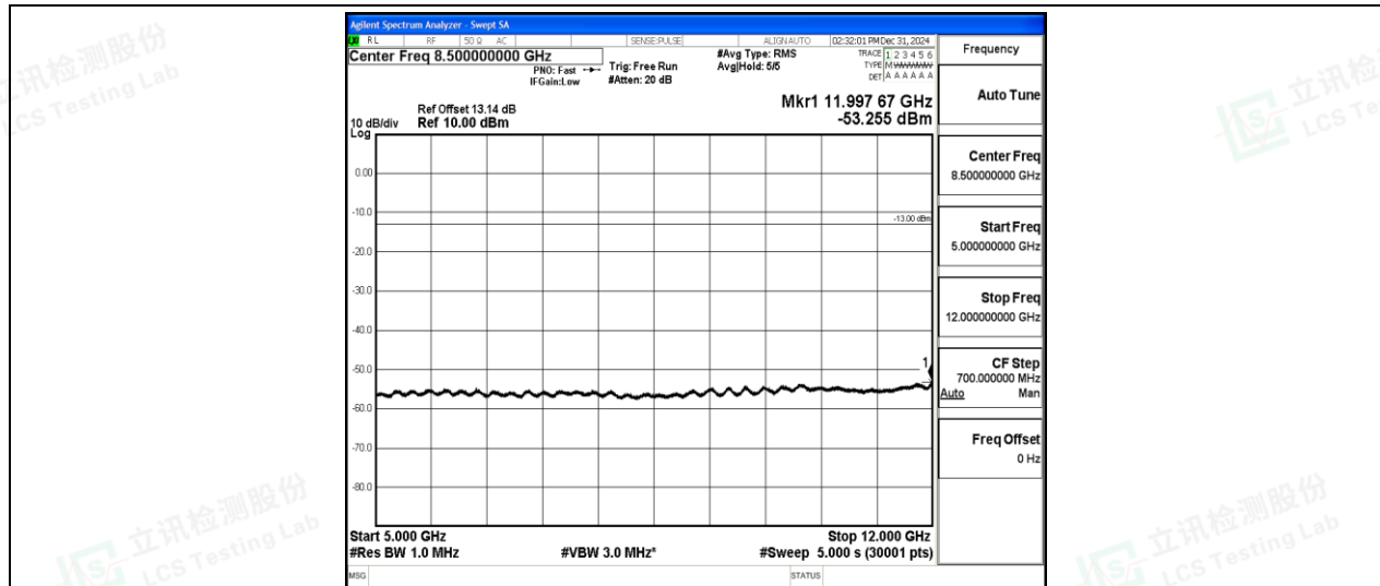
Band5-5MHz-QPSK-20625-1-0-High-5000-12000--53.26-PASS
