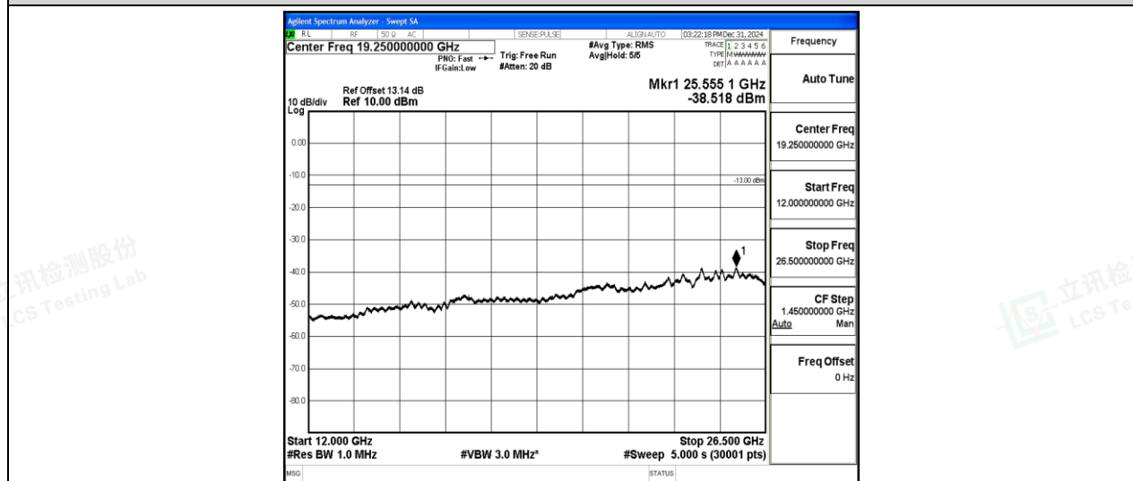
Band5-10MHz-QPSK-20600-1-0-High-12000-26500--38.52-PASS
