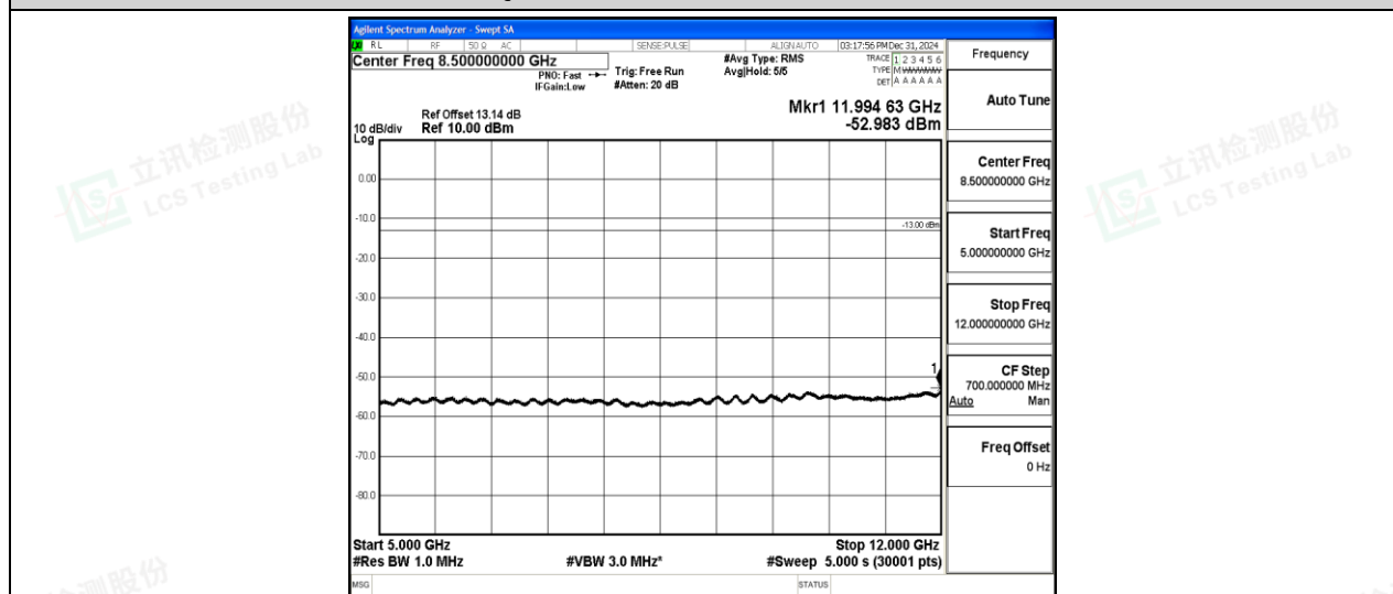
Band5-10MHz-QPSK-20525-1-0-Low-5000-12000--52.98-PASS
