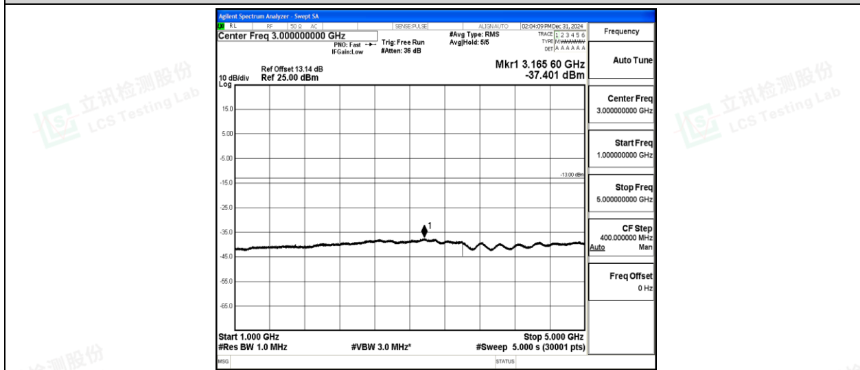
Band5-3MHz-16QAM-20635-1-0-High-1000-5000--37.4-PASS
