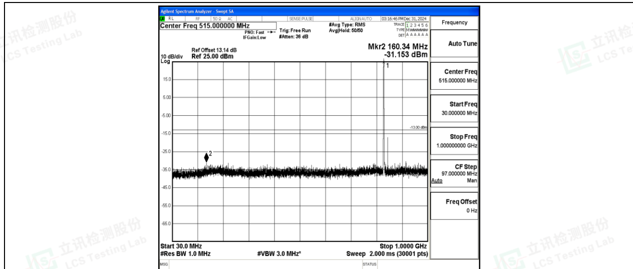
Band5-10MHz-QPSK-20525-1-0-Low-30-1000--31.15-PASS
