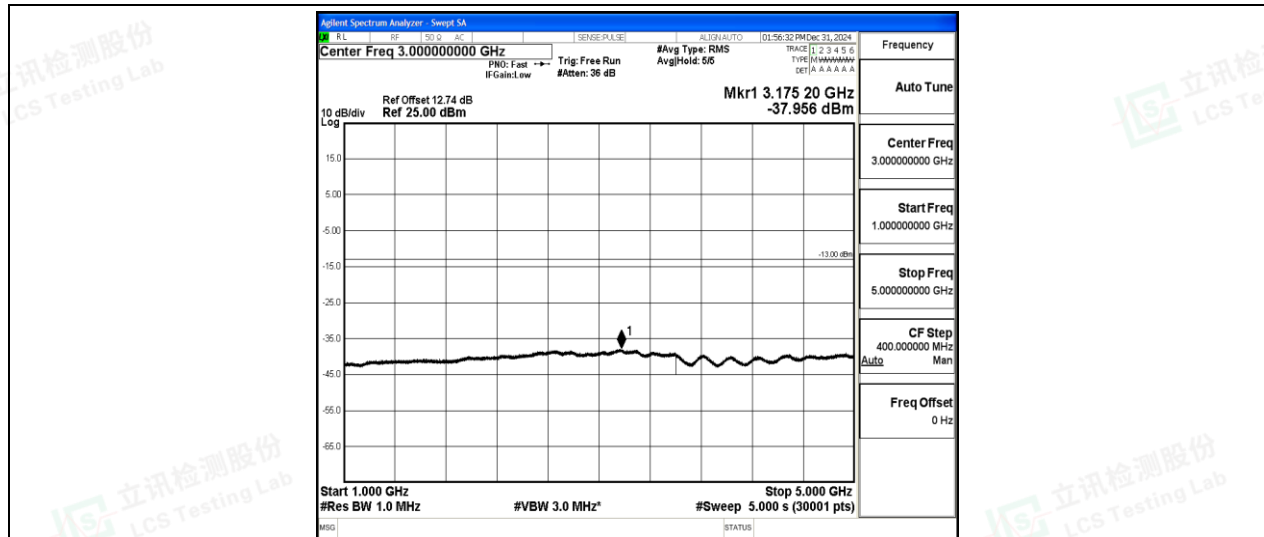
Band5-3MHz-16QAM-20415-1-0-Low-1000-5000--37.96-PASS
