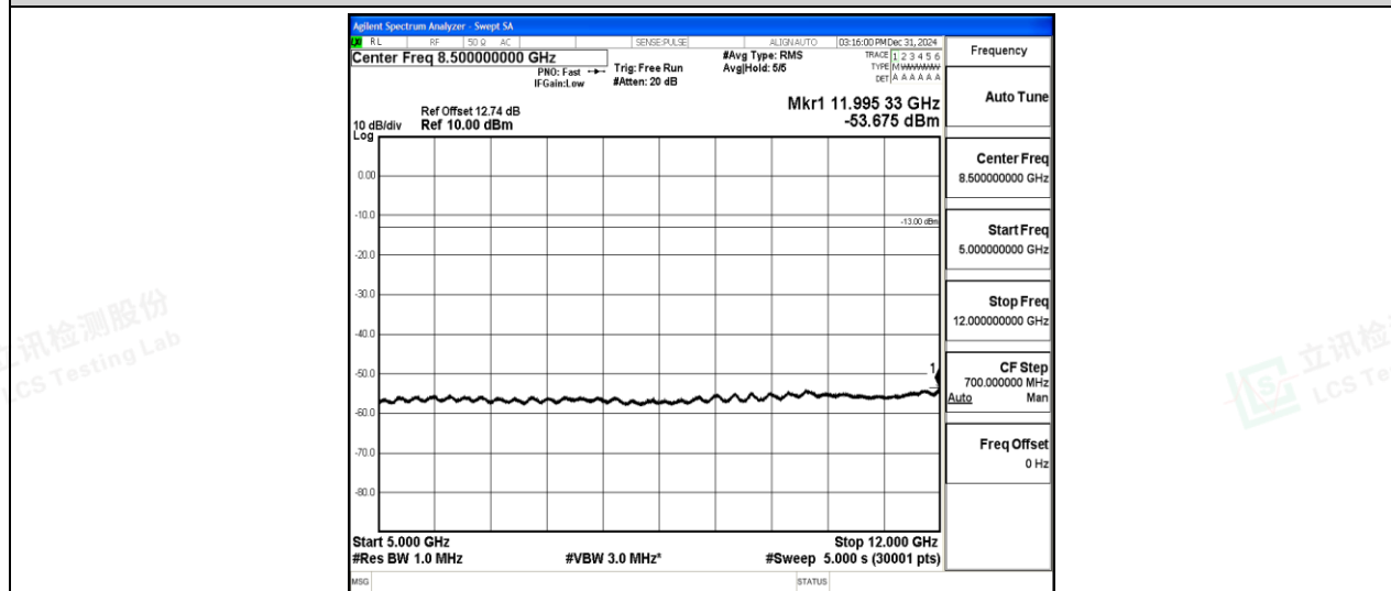
Band5-10MHz-16QAM-20450-1-0-Low-5000-12000--53.68-PASS
