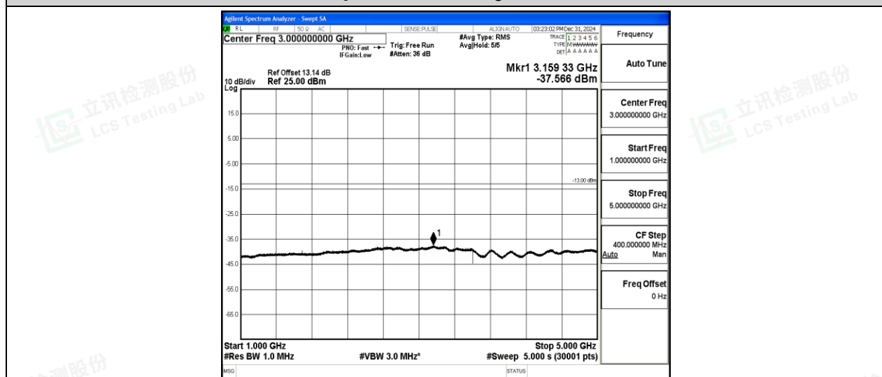
Band5-10MHz-16QAM-20600-1-0-High-1000-5000--37.57-PASS
