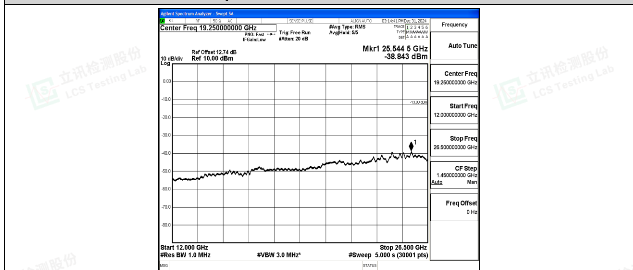
Band5-10MHz-QPSK-20450-1-0-Low-12000-26500--38.84-PASS
