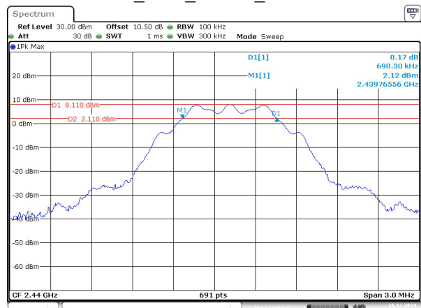
BLE_125k_Middle_Channel
