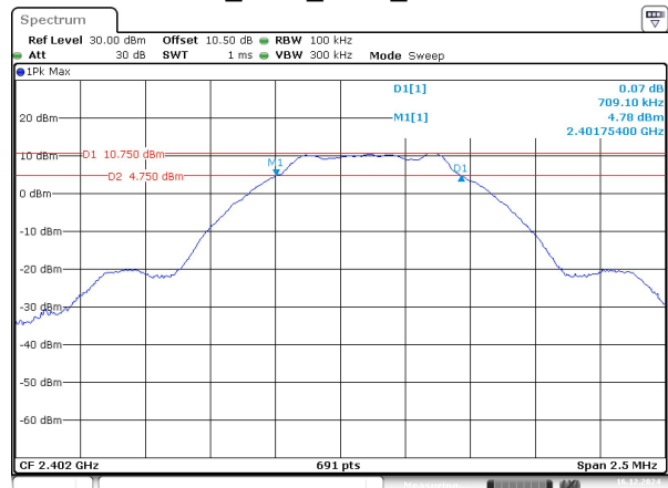
BLE_500k_Low_Channel
