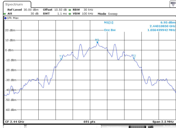
BLE_125k_Middle_Channel
