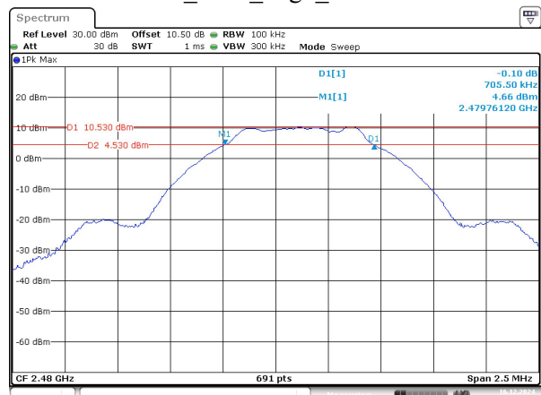
BLE_500k_High_Channel
