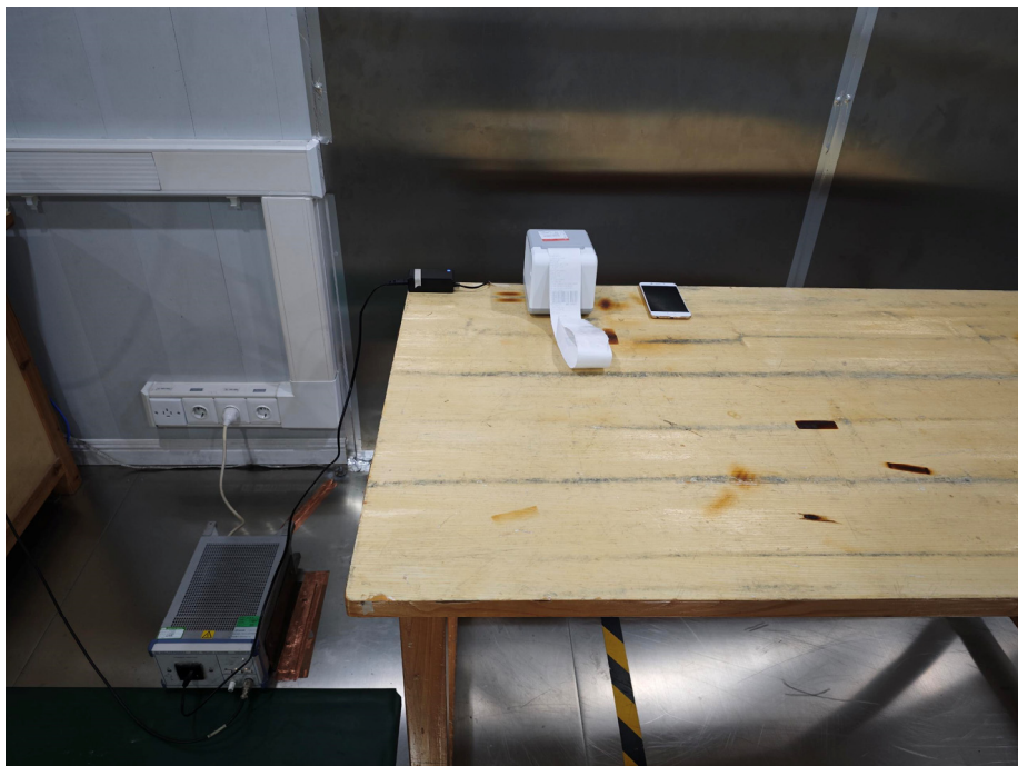
1.2 Photograph –AC Power Line Conducted Emission Test Setup
