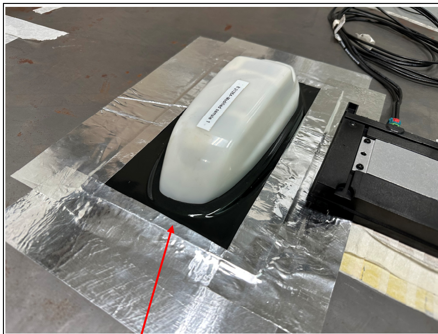
External Antenna
