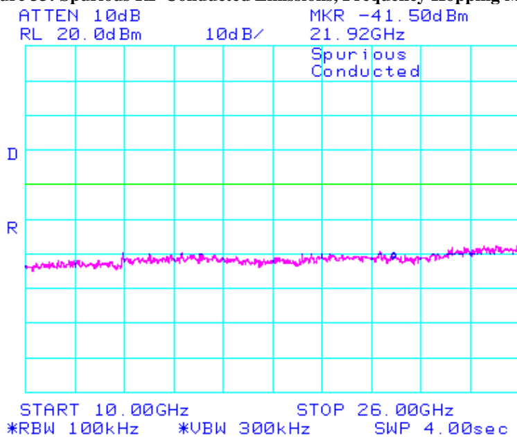
Figure 33: Spurious RF Conducted Emissions, Frequency Hopping Mode
