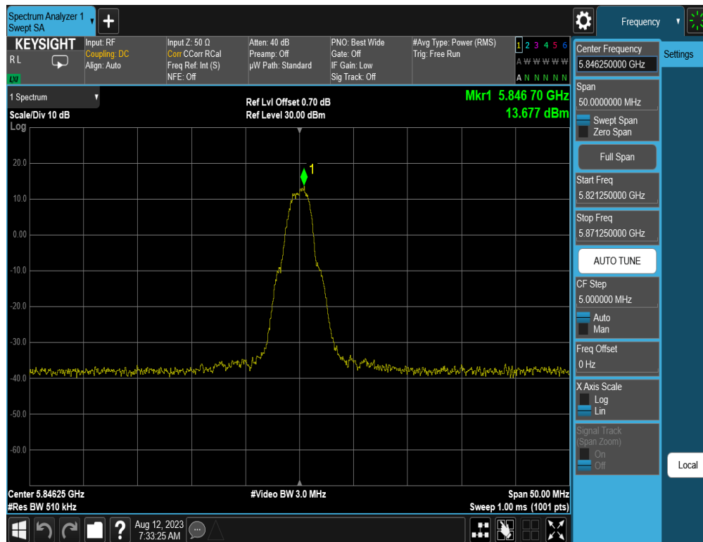
Plot 7-12. PSD (OQPSK, 5846.25MHz, 250kbps)
