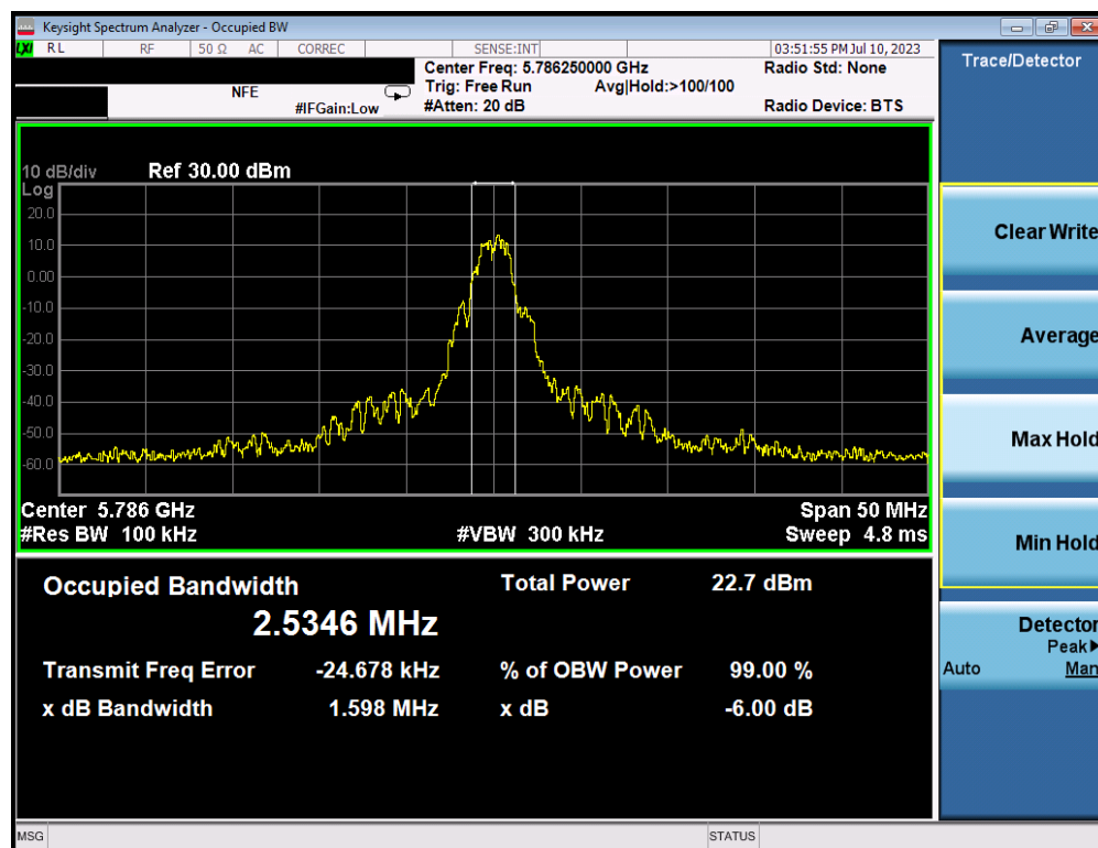
Plot 7-8. 6dB BW & 99% OBW (OQPSK, 5786.25MHz, 1000kbps)
