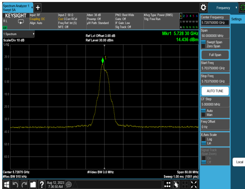
Plot 7-13. PSD (OQPSK, 5728.75MHz, 500kbps)
