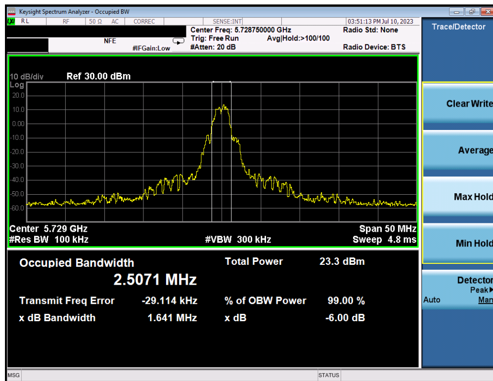
Plot 7-7. 6dB BW & 99% OBW (OQPSK, 5728.75MHz, 1000kbps)
