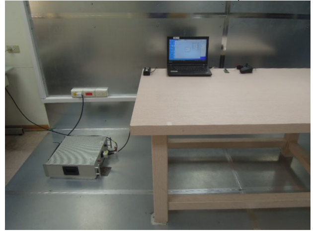
FCC_15_247_2.4G_Conduction_Setup
