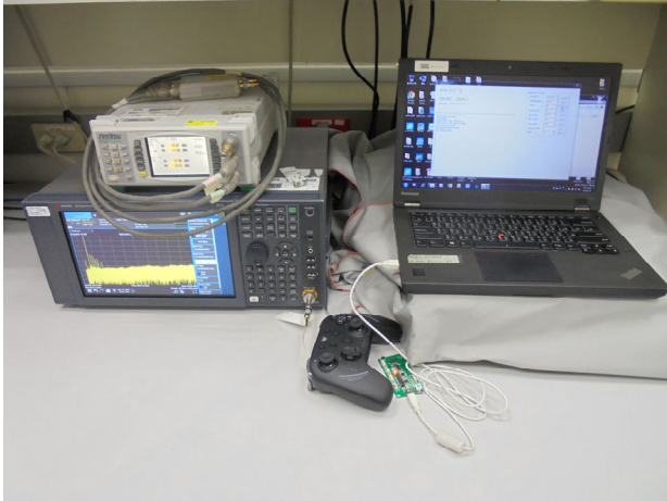
FCC_15_247_BT_conducted_setup
