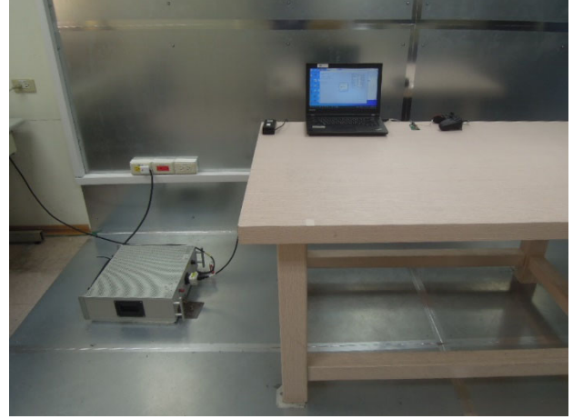
FCC_15_247_BLE_Conduction_Setup
