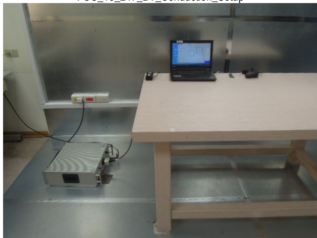
FCC_15_247_BT_Conduction_Setup
