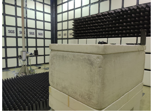
FCC_15_247_2.4G_Radiated_Setup
