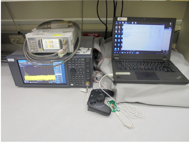
FCC_15_247_BLE_conducted_setup
