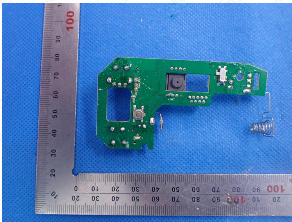
INTERNAL VIEW-5 OF EUT(D1023E)
