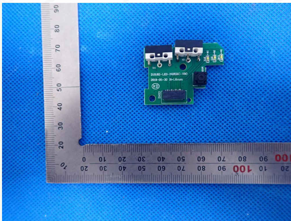
INTERNAL VIEW-3 OF EUT(D1018E)
