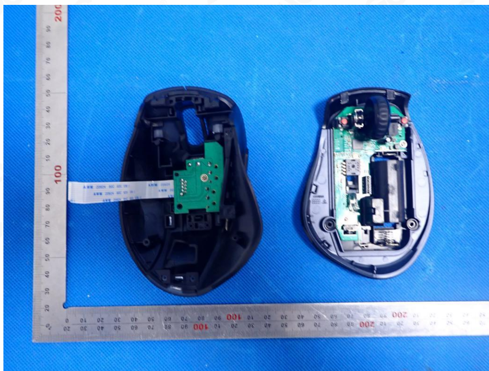
INTERNAL VIEW-1 OF EUT(D1018E)
