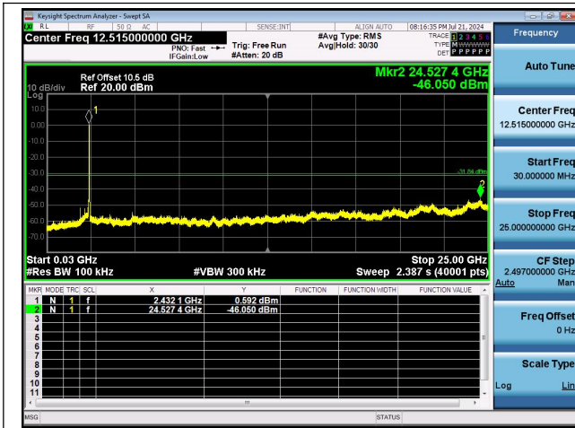
11AX40MIMO-Ant0-2437-30~25000-PASS
