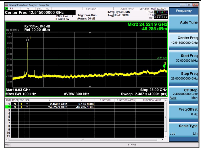
11AX40MIMO-Ant1-2452-30~25000-PASS
