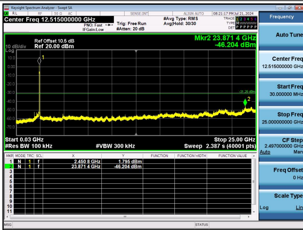
11AX40MIMO-Ant0-2452-30~25000-PASS
