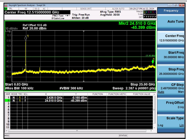
11AX40MIMO-Ant1-2437-30~25000-PASS
