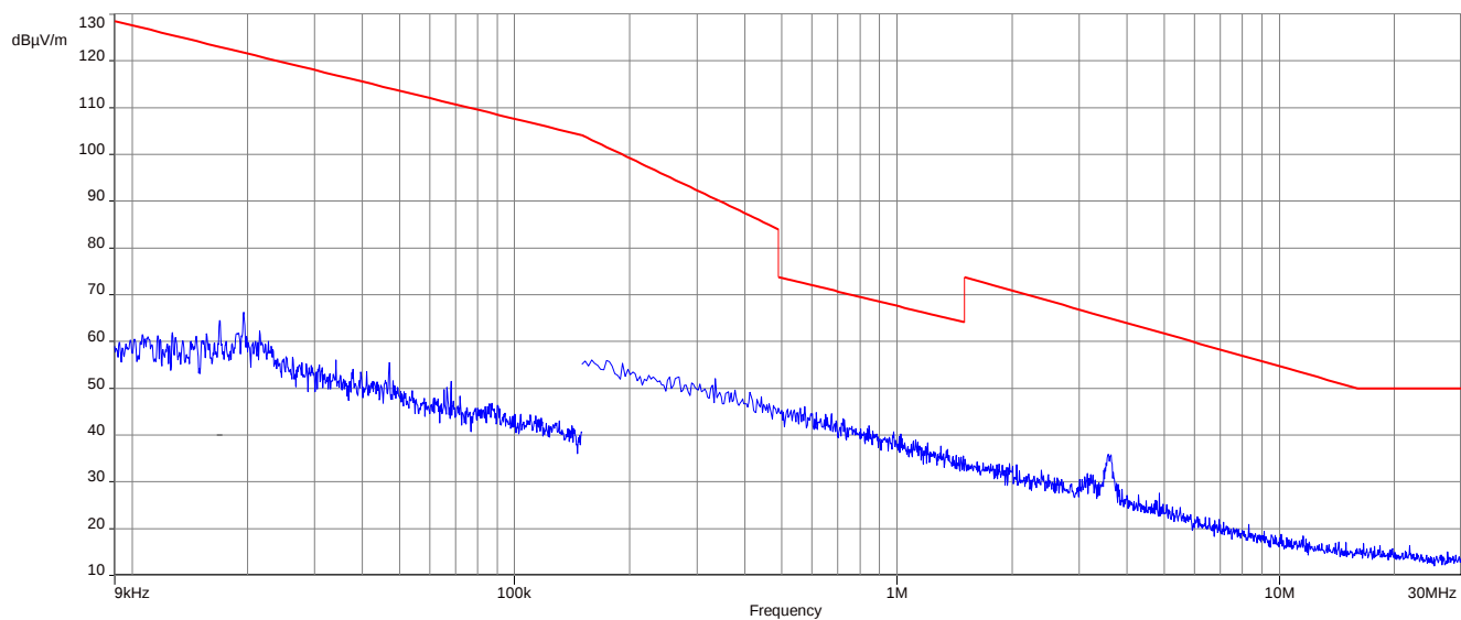
Plot 10: Channel 7, 15.209, TX Magnetic
