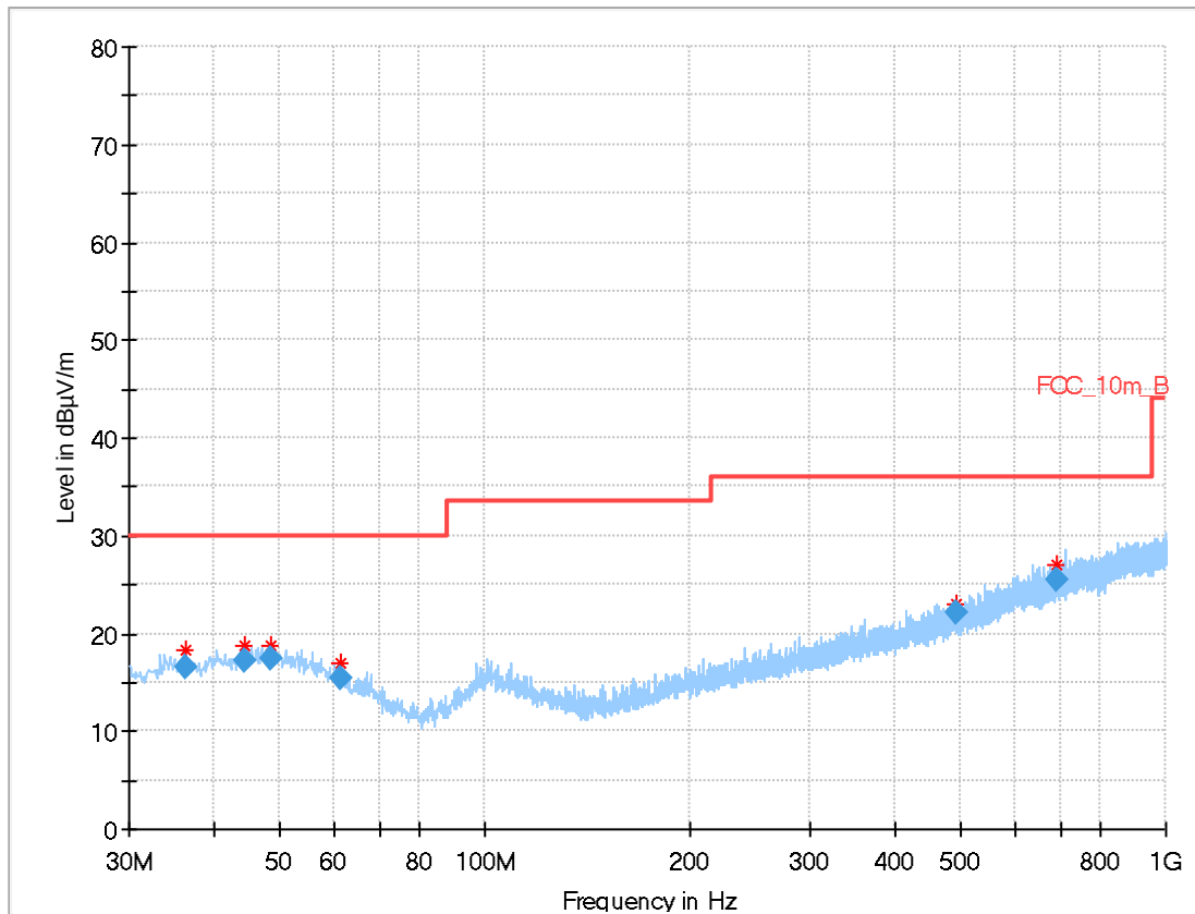
Plot 11: Channel 7, 15.209, 30 MHz – 1 GHz
