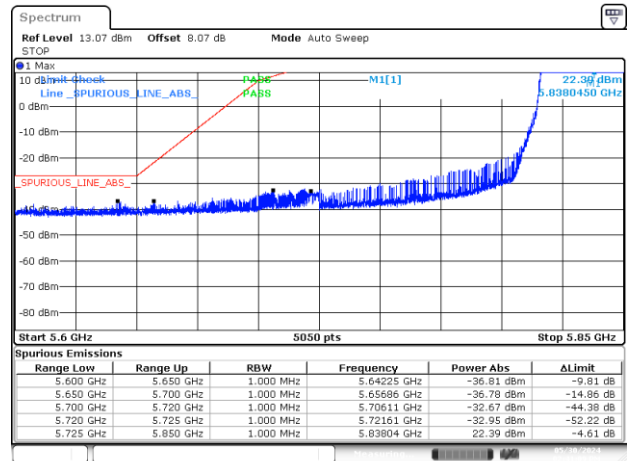
BE-NR-LOW, MIMO-B, 802.11ax/be40-MCS0, Ch167
