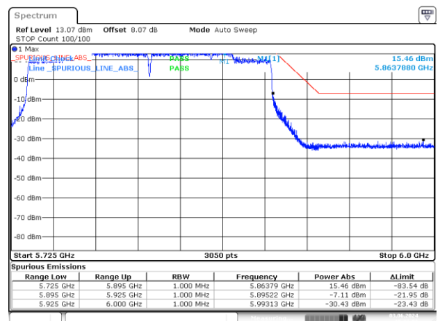
BE-NR-HIGH-PEAK, MIMO-B, 802.11ax/be160-MCS0, Ch163
