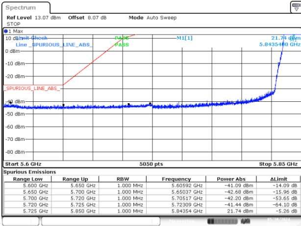
BE-NR-LOW, MIMO-B, 802.11ax/be20-MCS0, Ch169
