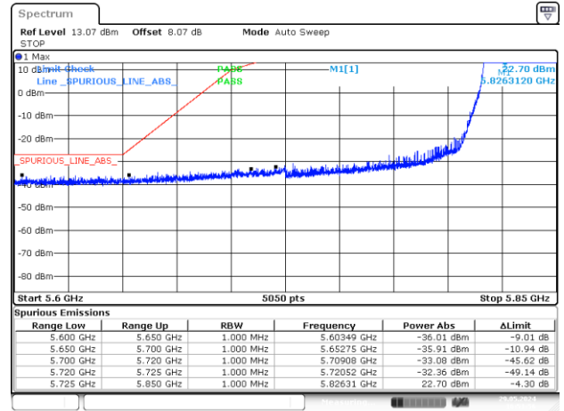
BE-NR-LOW, MIMO-A, 802.11n40-HT8, Ch167
