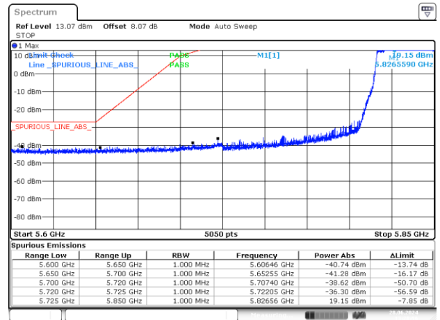
BE-NR-LOW, MIMO-A, 802.11ax/be40-MCS0, Ch167
