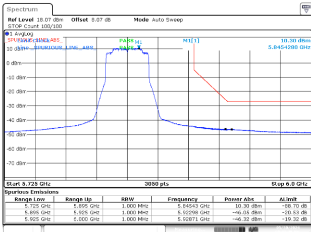
BE-NR-HIGH, MIMO-A, 802.11ax/be40-MCS0, Ch167
