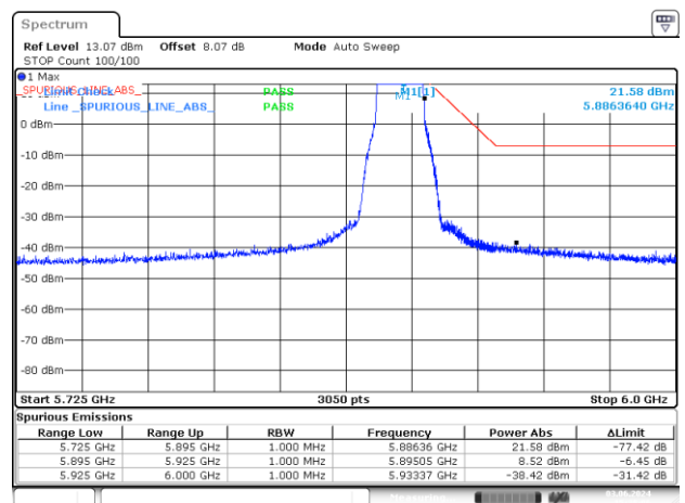
BE-NR-HIGH-PEAK, MIMO-B, 802.11ax/be20-MCS0, Ch177
