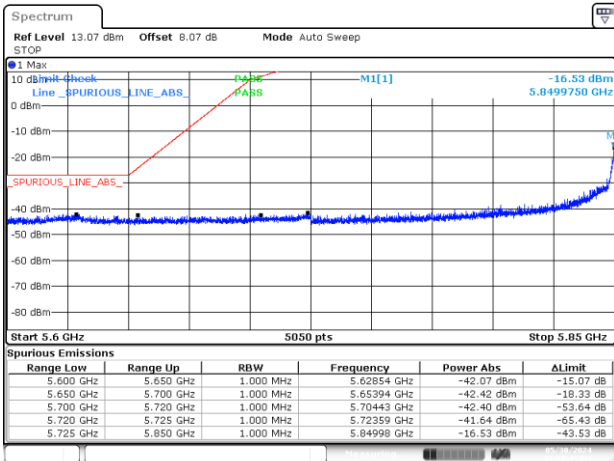
BE-NR-LOW, MIMO-B, 802.11ax/be20-MCS0, Ch173
