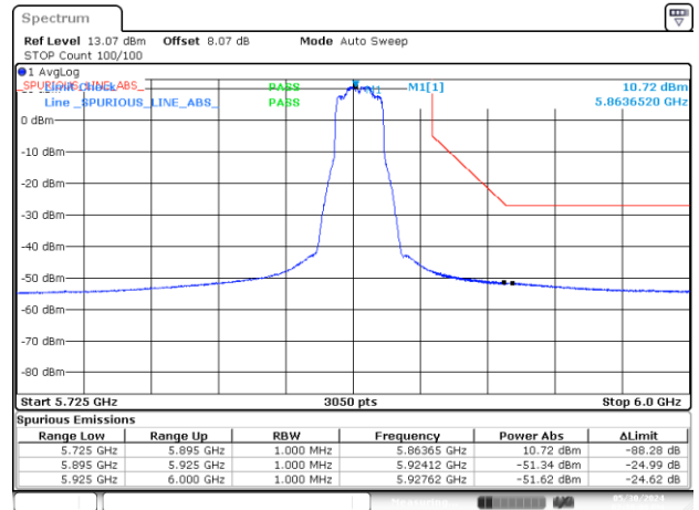
BE-NR-HIGH, MIMO-B, 802.11ax/be20-MCS0, Ch173
