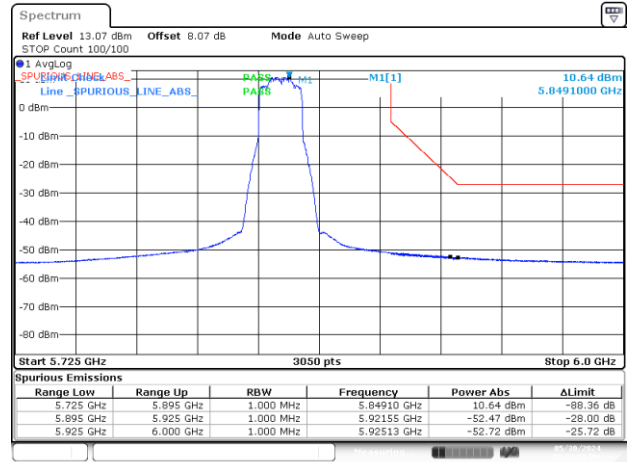
BE-NR-HIGH, MIMO-B, 802.11ax/be20-MCS0, Ch169
