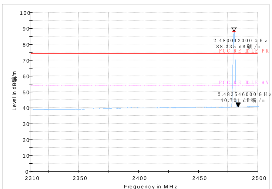
Fig.59 Radiated emission (High): GFSK, high channel
