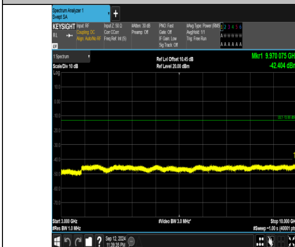
Band5_3MHz_QPSK_20635_15RB#0_3000~10000_3000~10000
