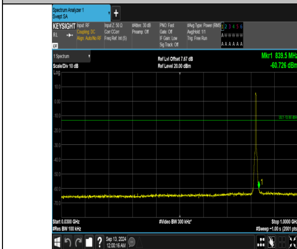
Band5_5MHz_QPSK_20425_25RB#0_30~1000_30~1000
