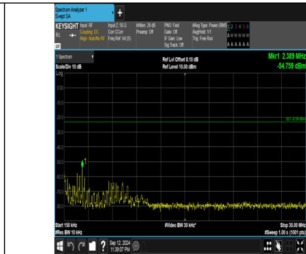
Band5_3MHz_QPSK_20635_15RB#0_0.15~30_0.15~30
