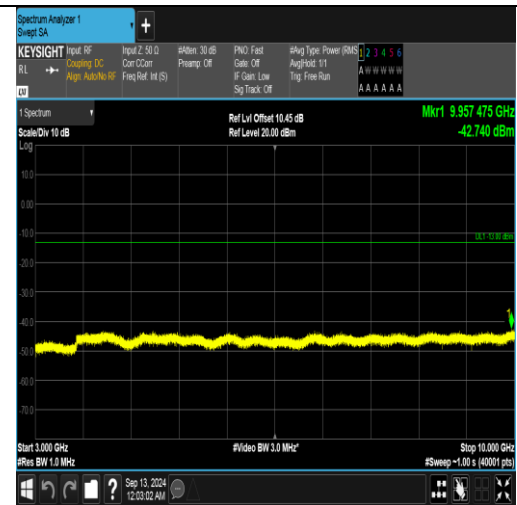
Band5_5MHz_16QAM_20525_1RB#0_3000~10000_3000~10000
