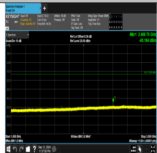
Band5_3MHz_QPSK_20635_1RB#14_1000~3000_1000~3000
