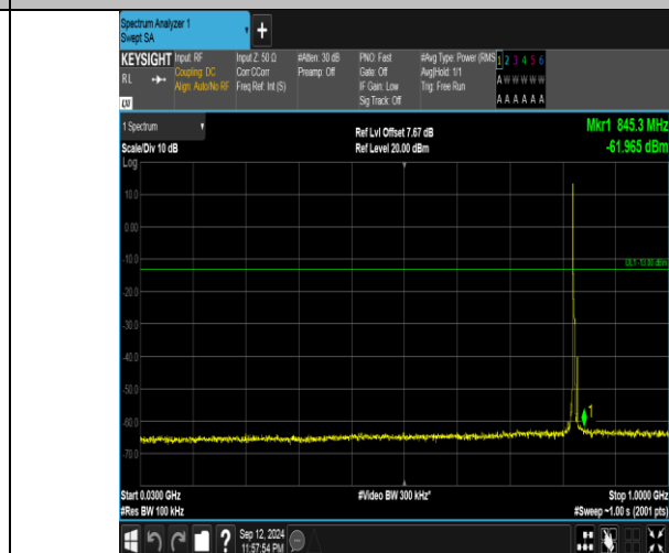
Band5_5MHz_16QAM_20425_1RB#0_30~1000_30~1000
