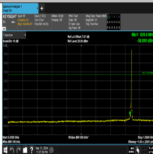
Band5_3MHz_QPSK_20635_1RB#14_30~1000_30~1000
