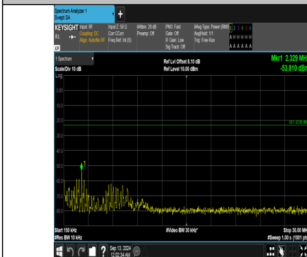
Band5_5MHz_16QAM_20525_1RB#0_0.15~30_0.15~30
