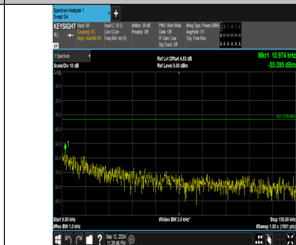
Band5_3MHz_16QAM_20635_15RB#0_0.009~0.15_0.009~0.15
