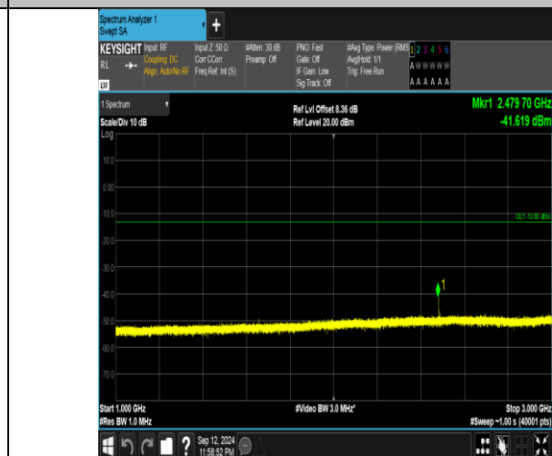
Band5_5MHz_QPSK_20425_1RB#24_1000~3000_1000~3000
