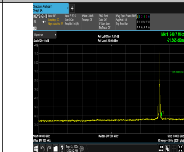
Band5_5MHz_16QAM_20525_1RB#0_30~1000_30~1000
