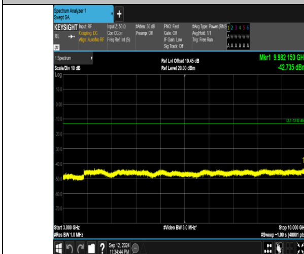
Band5_3MHz_QPSK_20525_15RB#0_3000~10000_3000~10000
