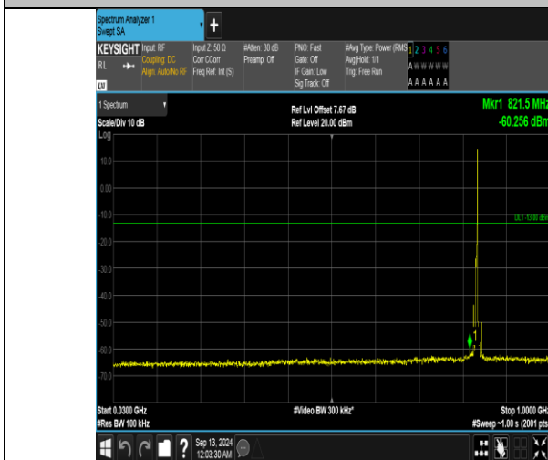
Band5_5MHz_QPSK_20525_1RB#24_30~1000_30~1000
