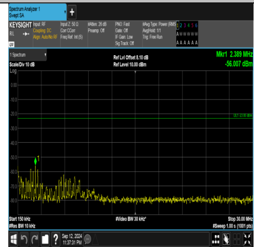
Band5_3MHz_QPSK_20635_1RB#14_0.15~30_0.15~30
