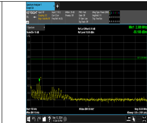
Band5_3MHz_QPSK_20525_15RB#0_0.15~30_0.15~30
