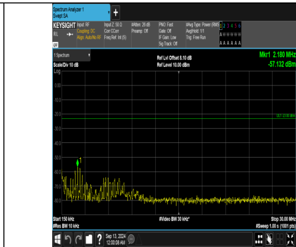
Band5_5MHz_QPSK_20425_25RB#0_0.15~30_0.15~30
