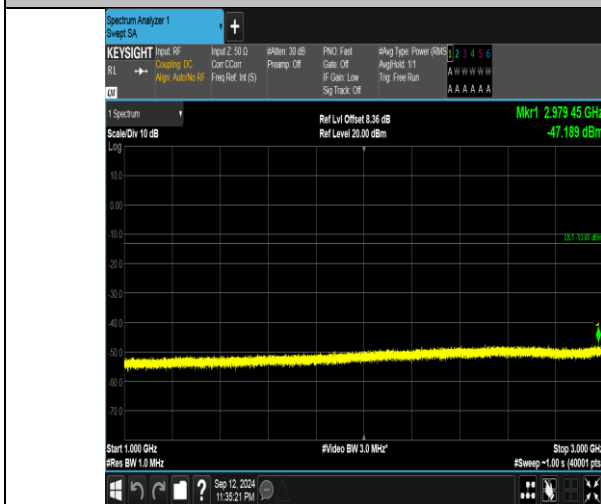
Band5_3MHz_16QAM_20525_15RB#0_1000~3000_1000~3000
