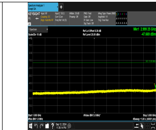
Band5_3MHz_QPSK_20635_1RB#0_1000~3000_1000~3000
