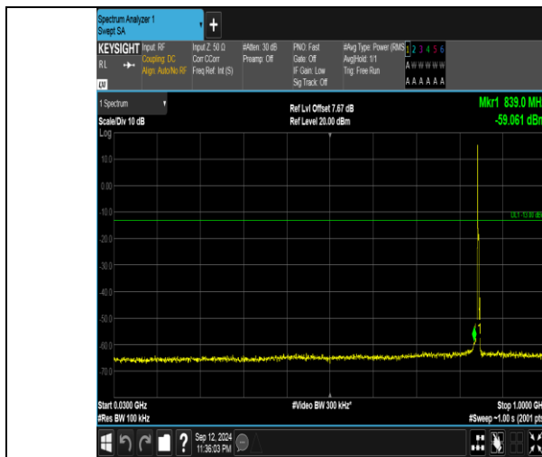
Band5_3MHz_QPSK_20635_1RB#0_30~1000_30~1000
