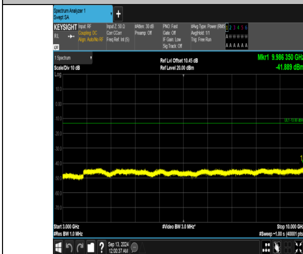
Band5_5MHz_QPSK_20425_25RB#0_3000~10000_3000~10000
