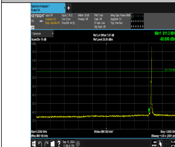
Band5_5MHz_QPSK_20425_1RB#24_30~1000_30~1000
