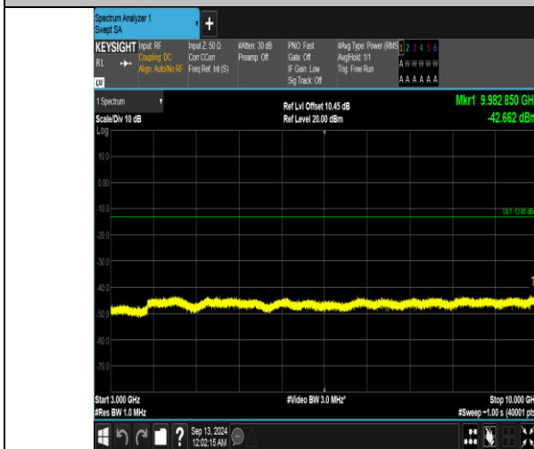
Band5_5MHz_QPSK_20525_1RB#0_3000~10000_3000~10000
