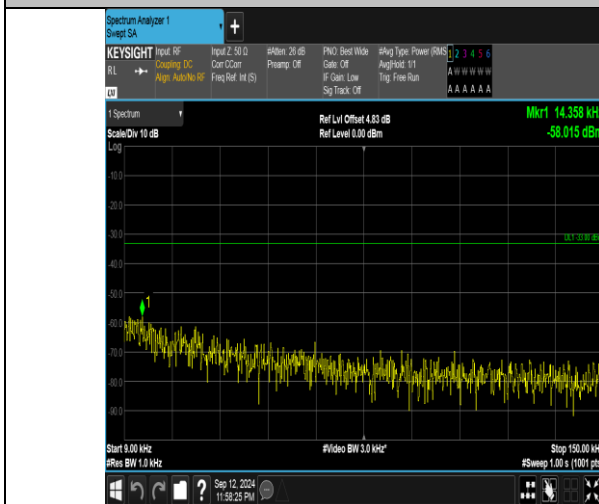
Band5_5MHz_QPSK_20425_1RB#24_0.009~0.15_0.009~0.15
