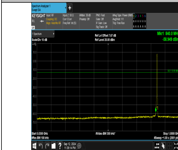
Band5_3MHz_QPSK_20635_15RB#0_30~1000_30~1000
