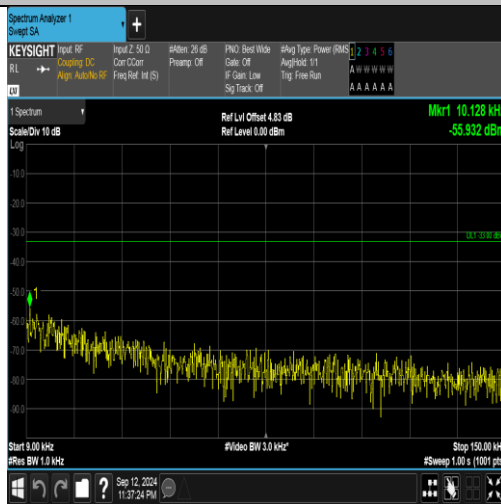
Band5_3MHz_QPSK_20635_1RB#14_0.009~0.15_0.009~0.15
