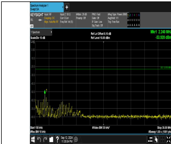
Band5_3MHz_16QAM_20525_15RB#0_0.15~30_0.15~30
