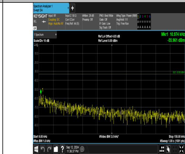
Band5_3MHz_16QAM_20635_1RB#0_0.009~0.15_0.009~0.15
