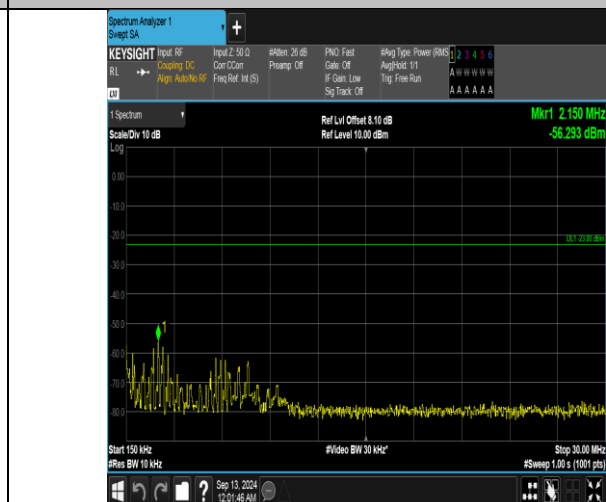
Band5_5MHz_QPSK_20525_1RB#0_0.15~30_0.15~30
