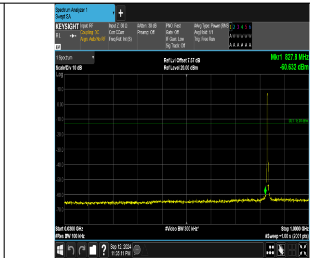
Band5_3MHz_16QAM_20525_15RB#0_30~1000_30~1000
