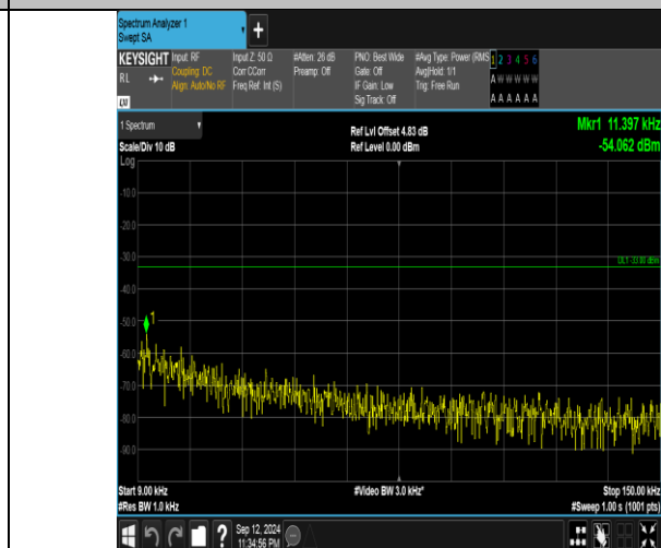
Band5_3MHz_16QAM_20525_15RB#0_0.009~0.15_0.009~0.15
