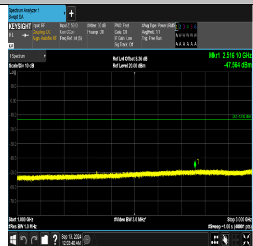
Band5_5MHz_QPSK_20525_1RB#24_1000~3000_1000~3000
