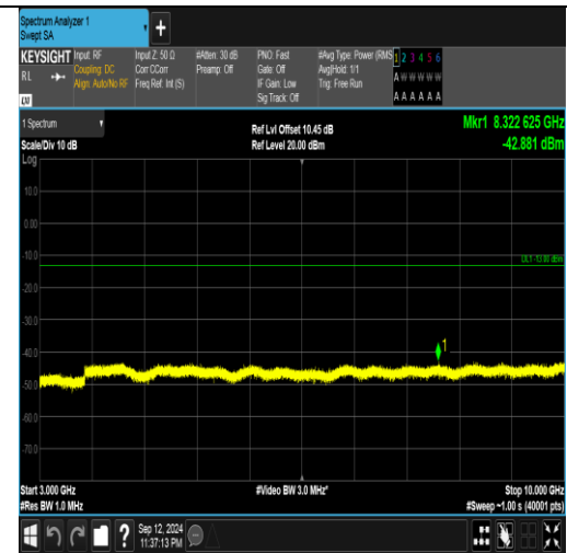
Band5_3MHz_16QAM_20635_1RB#0_3000~10000_3000~10000
