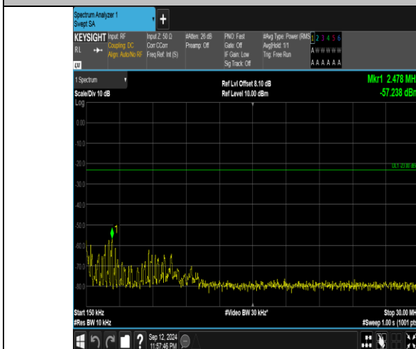
Band5_5MHz_16QAM_20425_1RB#0_0.15~30_0.15~30
