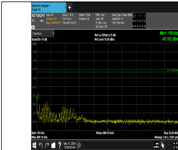
Band5_5MHz_16QAM_20425_25RB#0_0.15~30_0.15~30
