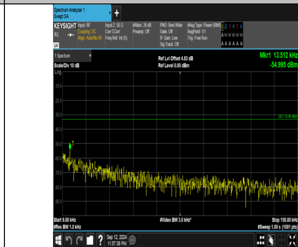
Band5_5MHz_16QAM_20425_1RB#0_0.009~0.15_0.009~0.15
