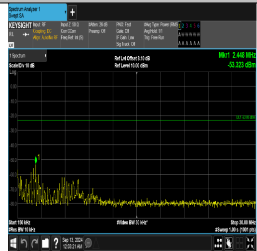
Band5_5MHz_QPSK_20525_1RB#24_0.15~30_0.15~30
