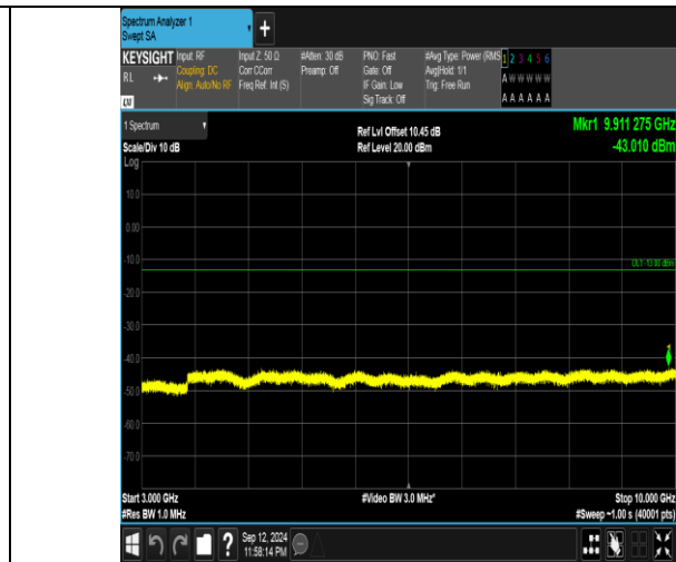
Band5_5MHz_16QAM_20425_1RB#0_3000~10000_3000~10000
