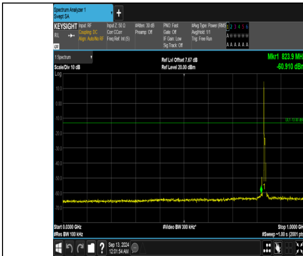
Band5_5MHz_QPSK_20525_1RB#0_30~1000_30~1000
