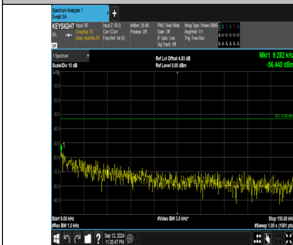
Band5_3MHz_QPSK_20635_1RB#0_0.009~0.15_0.009~0.15
