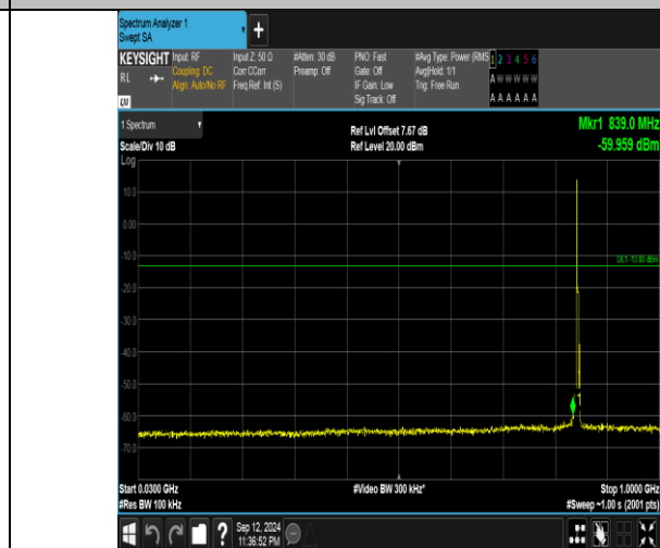
Band5_3MHz_16QAM_20635_1RB#0_30~1000_30~1000
