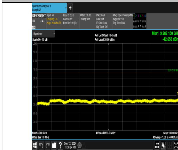
Band5_3MHz_QPSK_20635_1RB#0_3000~10000_3000~10000
