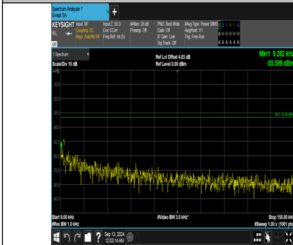
Band5_5MHz_QPSK_20525_1RB#24_0.009~0.15_0.009~0.15
