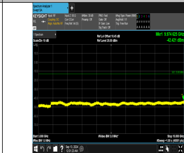
Band5_5MHz_16QAM_20425_25RB#0_3000~10000_3000~10000
