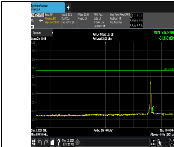
Band5_5MHz_QPSK_20425_1RB#0_30~1000_30~1000
