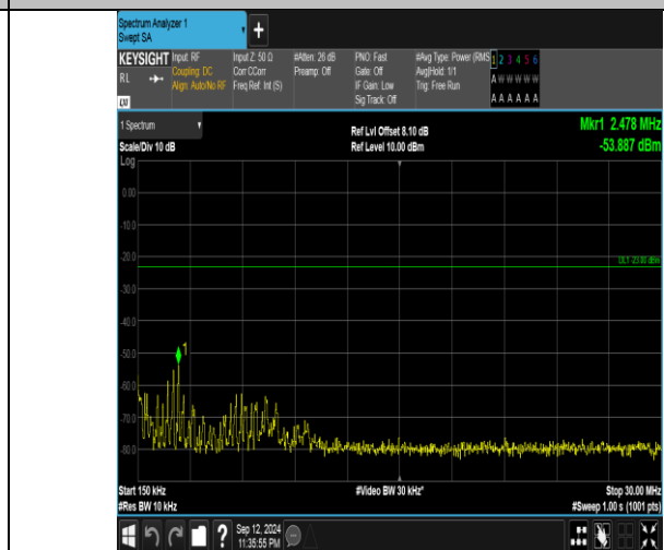
Band5_3MHz_QPSK_20635_1RB#0_0.15~30_0.15~30
