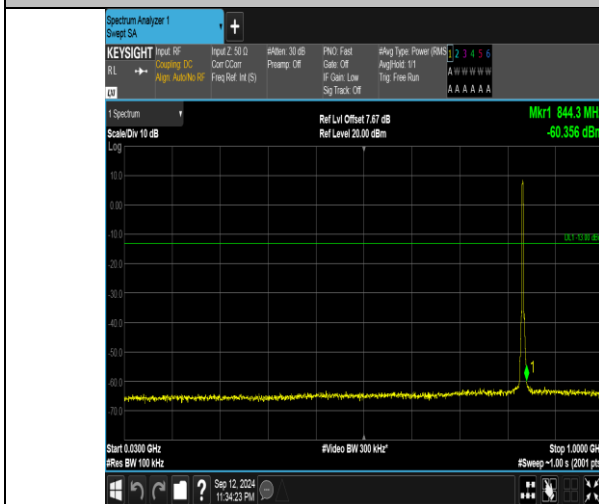
Band5_3MHz_QPSK_20525_15RB#0_30~1000_30~1000
