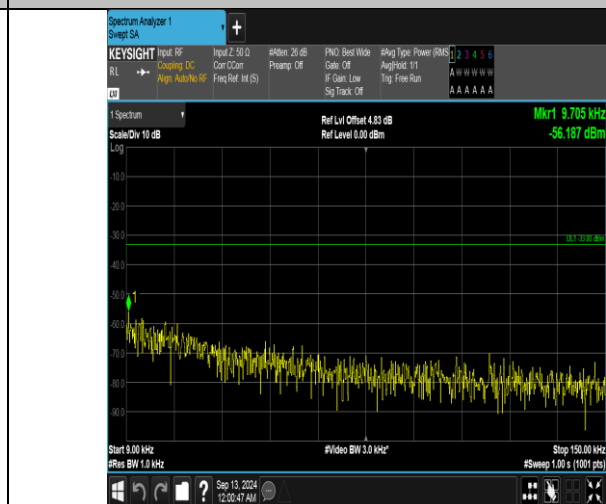
Band5_5MHz_16QAM_20425_25RB#0_0.009~0.15_0.009~0.15
