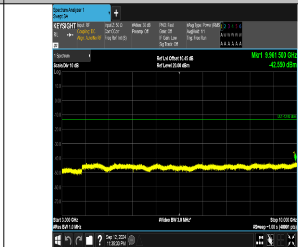
Band5_3MHz_16QAM_20525_15RB#0_3000~10000_3000~10000
