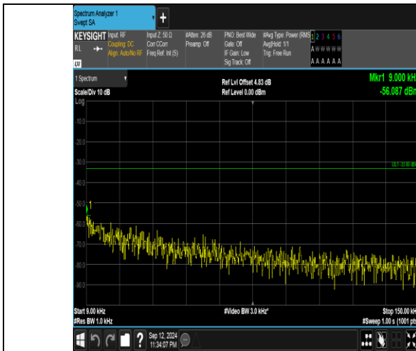
Band5_3MHz_QPSK_20525_15RB#0_0.009~0.15_0.009~0.15
