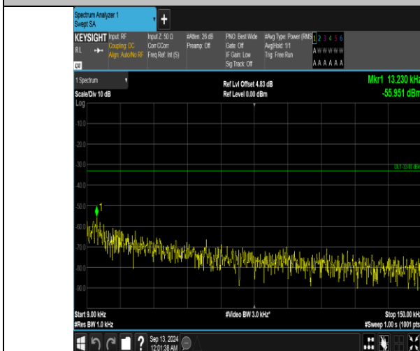
Band5_5MHz_QPSK_20525_1RB#0_0.009~0.15_0.009~0.15
