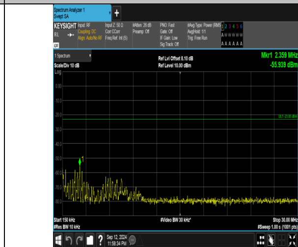
Band5_5MHz_QPSK_20425_1RB#24_0.15~30_0.15~30
