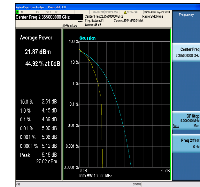
Band40(2350-2360)-10MHz-QPSK-39200-1RB#0-PASS
