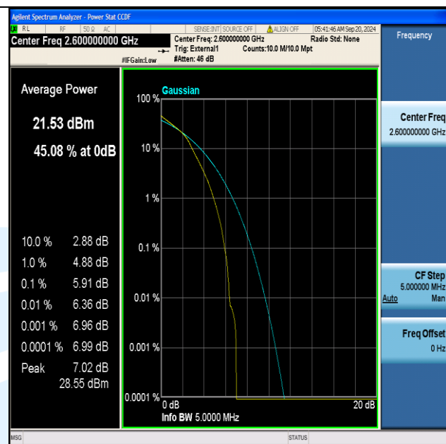
Band41(2555-2655)-5MHz-16QAM-40690-25RB#0-PASS
