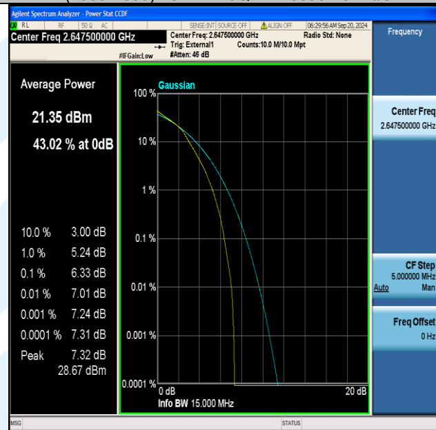
Band41(2555-2655)-15MHz-16QAM-41165-75RB#0-PASS
