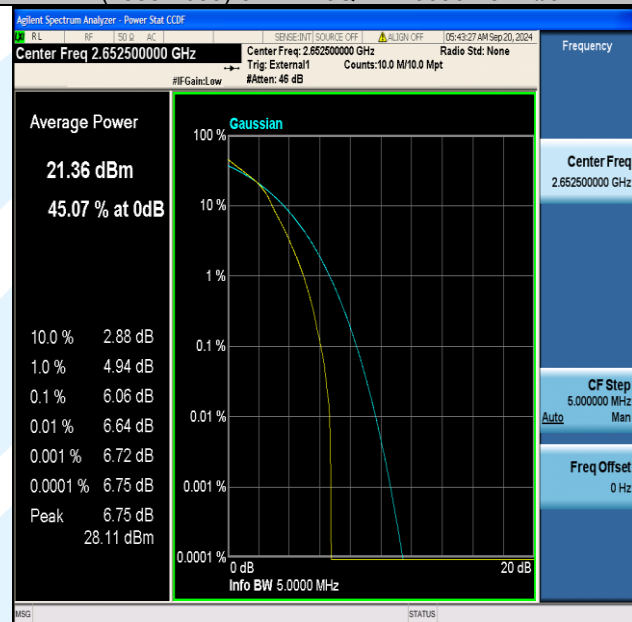
Band41(2555-2655)-5MHz-16QAM-41215-25RB#0-PASS
