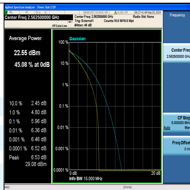
Band41(2555-2655)-15MHz-QPSK-40315-75RB#0-PASS
