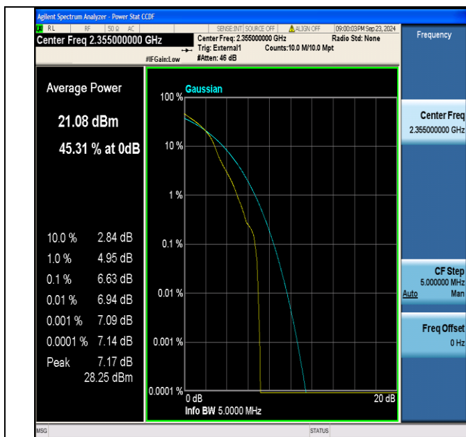
Band40(2350-2360)-5MHz-16QAM-39200-1RB#0-PASS
