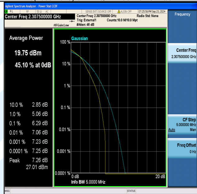
Band40(2305-2315)-5MHz-16QAM-38725-25RB#0-PASS
