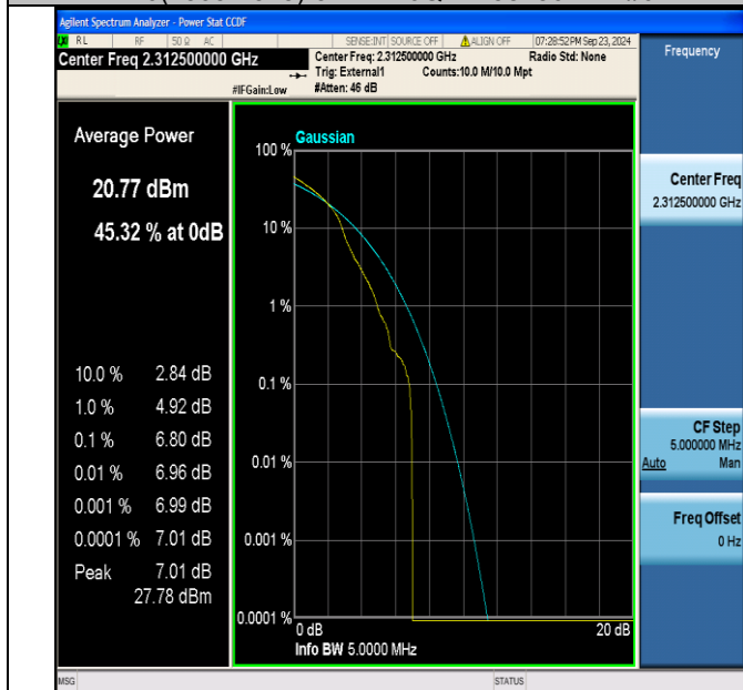
Band40(2305-2315)-5MHz-16QAM-38775-1RB#0-PASS
