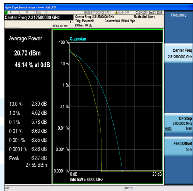
Band40(2305-2315)-5MHz-QPSK-38775-25RB#0-PASS
