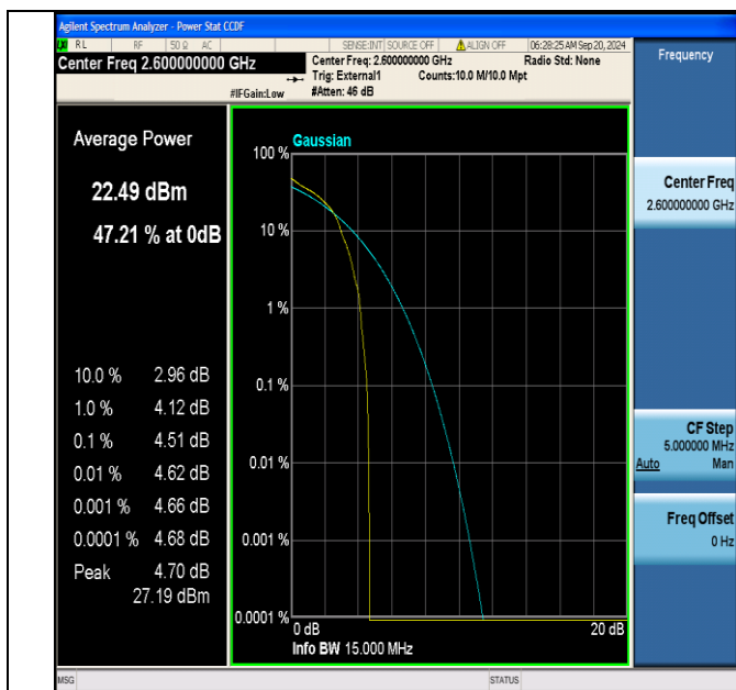
Band41(2555-2655)-15MHz-16QAM-40690-1RB#0-PASS
