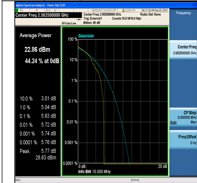
Band41(2555-2655)-15MHz-16QAM-40315-1RB#0-PASS
