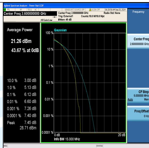
Band41(2555-2655)-15MHz-16QAM-40690-75RB#0-PASS
