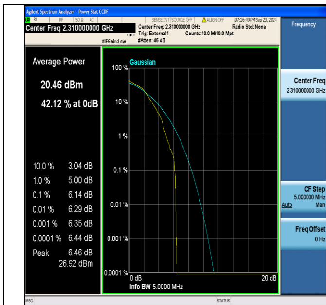
Band40(2305-2315)-5MHz-16QAM-38750-1RB#0-PASS
