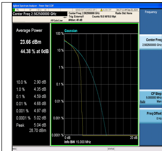
Band41(2555-2655)-15MHz-QPSK-40315-1RB#0-PASS
