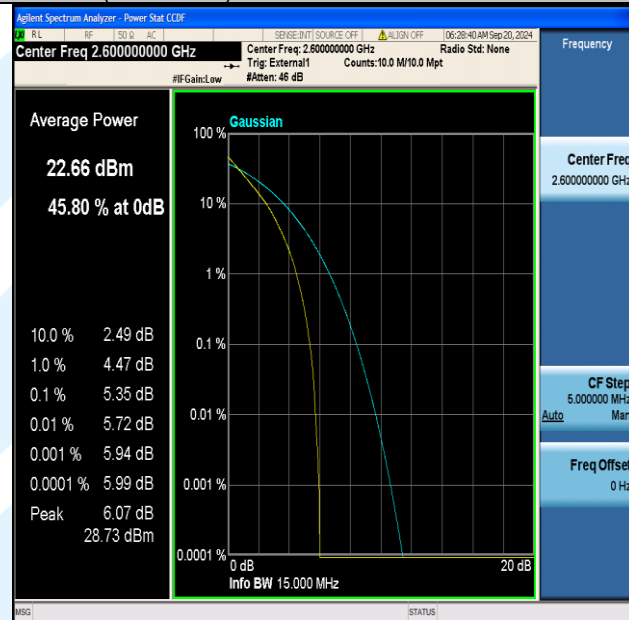
Band41(2555-2655)-15MHz-QPSK-40690-75RB#0-PASS
