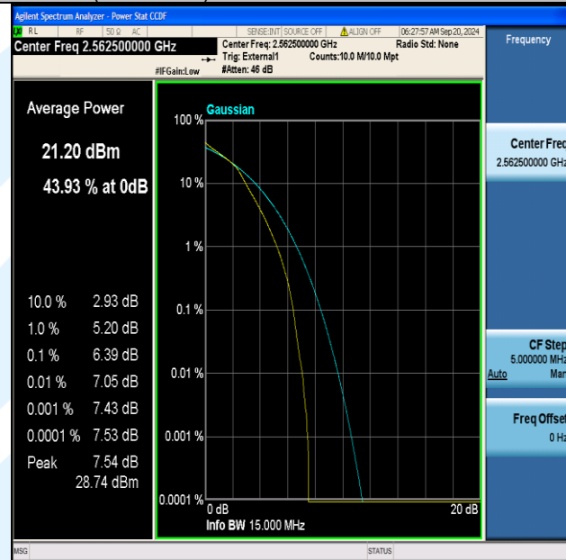
Band41(2555-2655)-15MHz-16QAM-40315-75RB#0-PASS
