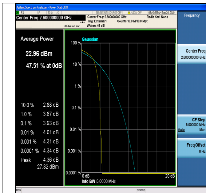
Band41(2555-2655)-5MHz-16QAM-40690-1RB#0-PASS
