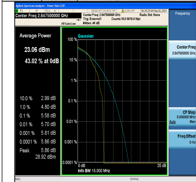
Band41(2555-2655)-15MHz-16QAM-41165-1RB#0-PASS
