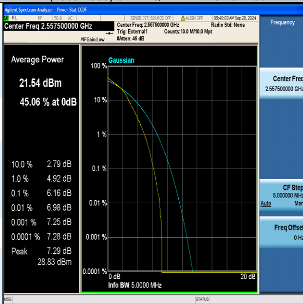
Band41(2555-2655)-5MHz-16QAM-40265-25RB#0-PASS
