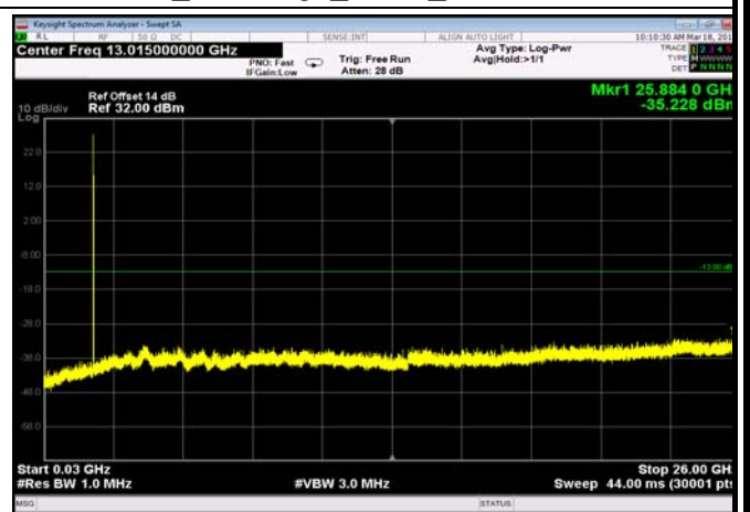
FDD04_HighRange_10MHz_30MHz~26GHz
