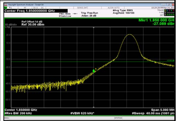
LowRange_FDD02_20MHz_1860_OneRB _low_Q16
