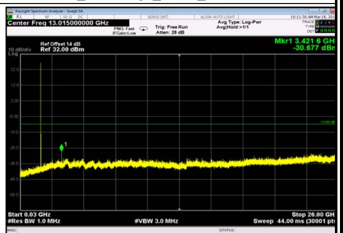
FDD04_MidRange_10MHz_30MHz~26GHz
