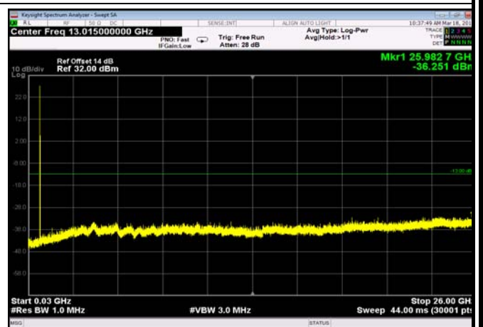
FDD12_MidRange_5MHz_30MHz~26GHz
