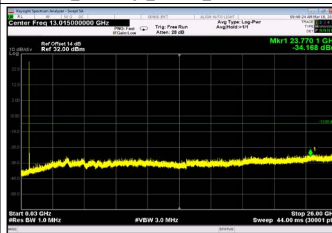
FDD12_LowRange_3MHz_30MHz~26GHz
