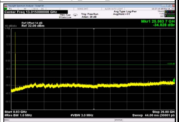
FDD12_LowRange_5MHz_30MHz~26GHz
