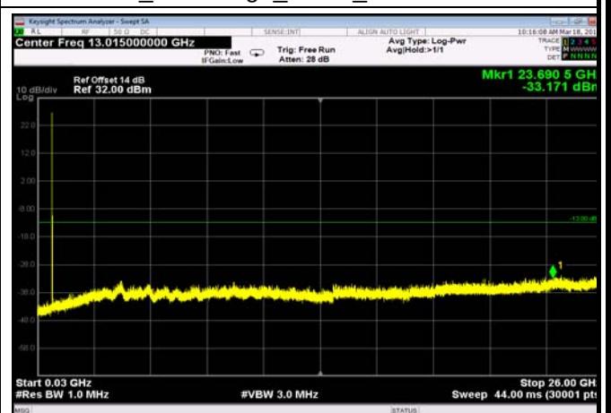
FDD12_LowRange_5MHz_30MHz~26GHz
