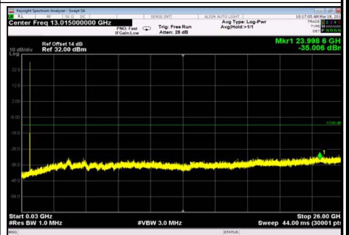
FDD12_LowRange_10MHz_30MHz~26GHz
