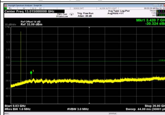
FDD04_MidRange_1.4MHz_30MHz~26GHz
