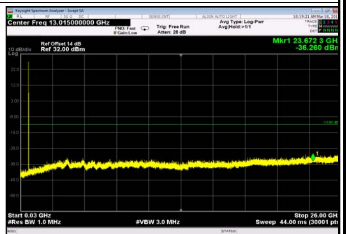
FDD17_MidRange_5MHz_30MHz~26GHz
