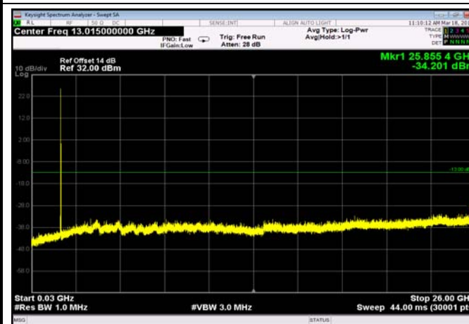
FDD04_HighRange_3MHz_30MHz~26GHz
