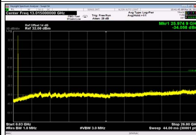
FDD17_MidRange_10MHz_30MHz~26GHz
