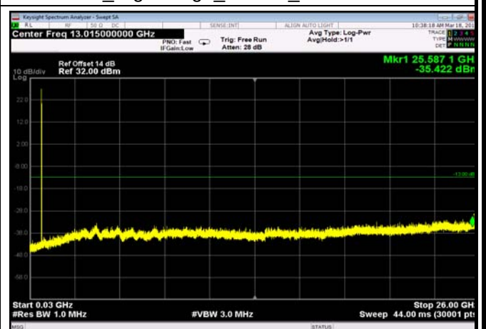
FDD12_HighRange_10MHz_30MHz~26GHz
