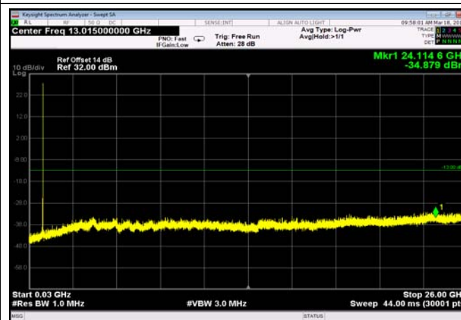
FDD05_LowRange_1.4MHz_30MHz~26GHz
