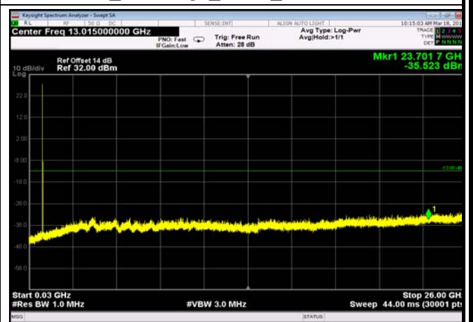
FDD12_HighRange_10MHz_30MHz~26GHz
