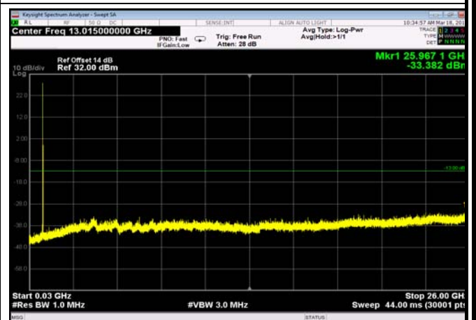
FDD05_MidRange_5MHz_30MHz~26GHz
