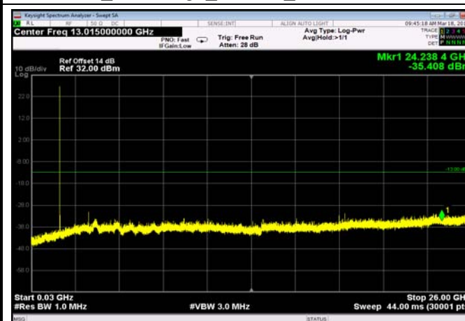
FDD04_LowRange_1.4MHz_30MHz~26GHz
