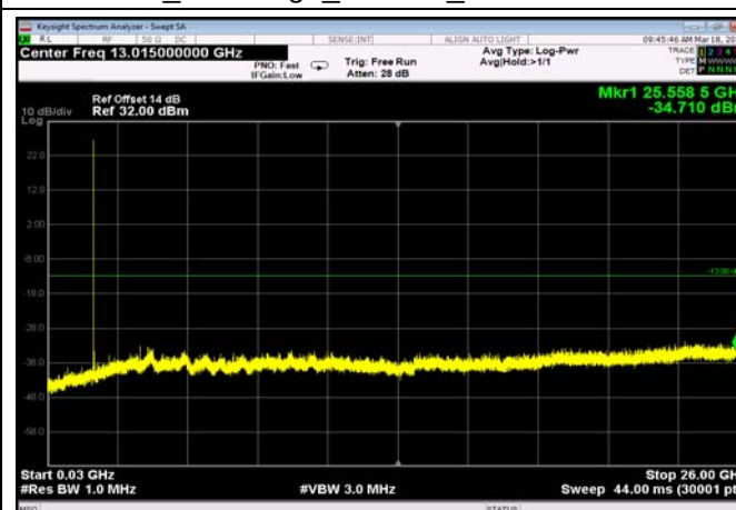
FDD04_MidRange_1.4MHz_30MHz~26GHz
