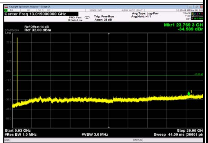
FDD17_MidRange_5MHz_30MHz~26GHz
