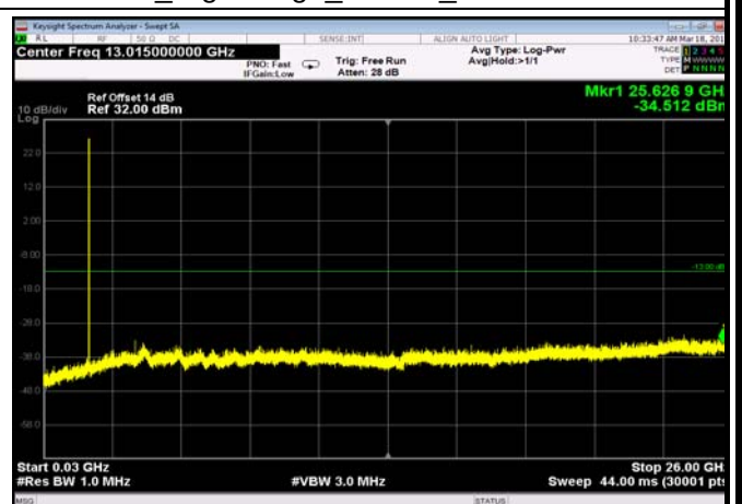
FDD04_HighRange_10MHz_30MHz~26GHz
