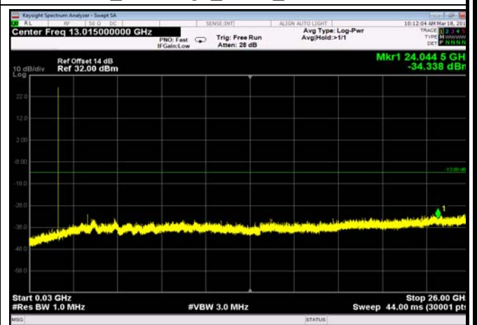
FDD05_HighRange_10MHz_30MHz~26GHz
