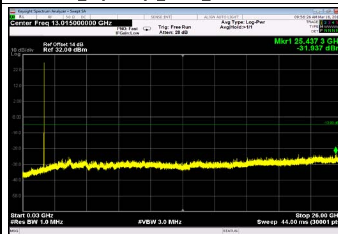
FDD04_LowRange_1.4MHz_30MHz~26GHz
