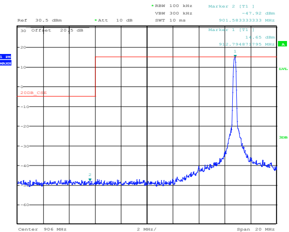
Figure 8.4-2: Conducted spurious emissions at mid channel
