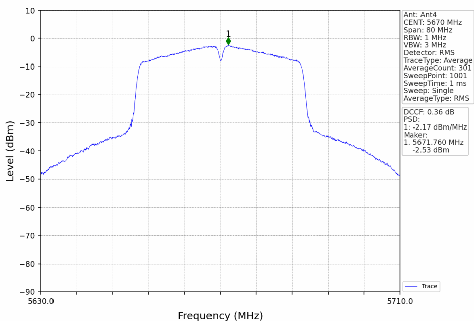
802.11ac(VHT40)_HCH_5670MHz_Ant4_NTNV
