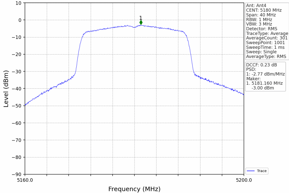
802.11ax(HEW20)_LCH_5180MHz_RU242_Left_MIMO_NTNV
