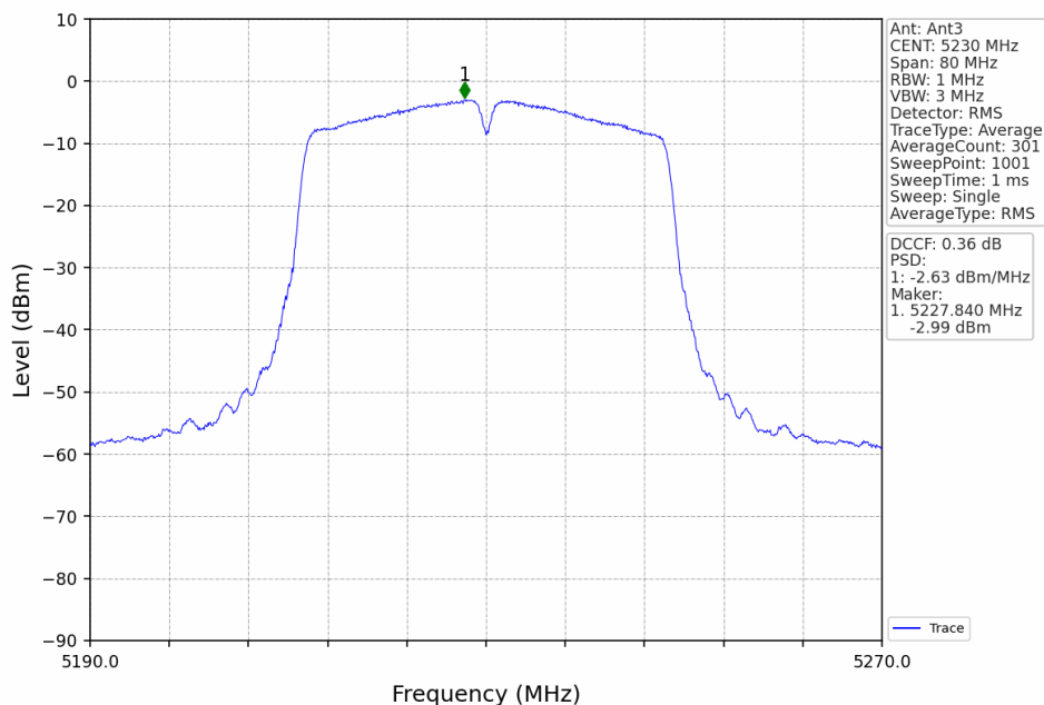
802.11ac(VHT40)_HCH_5230MHz_Ant3_NTNV
