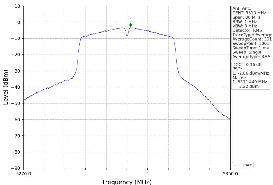
802.11ac(VHT40)_HCH_5310MHz_Ant3_NTNV
