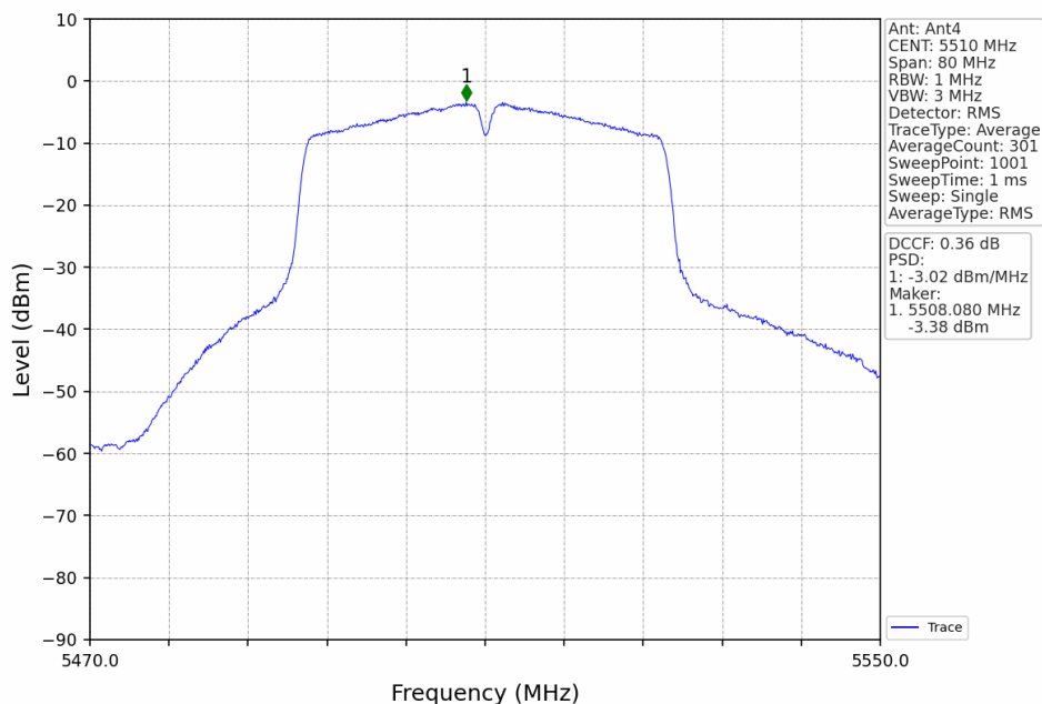
802.11ac(VHT40)_LCH_5510MHz_Ant4_NTNV
