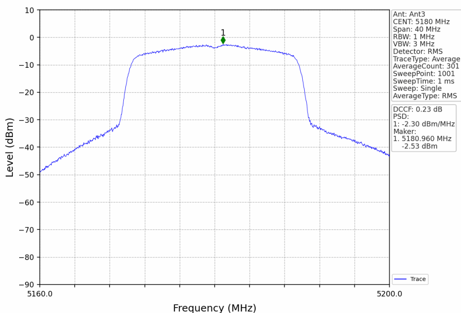
802.11ax(HEW20)_LCH_5180MHz_RU242_Left_Ant3_NTNV
