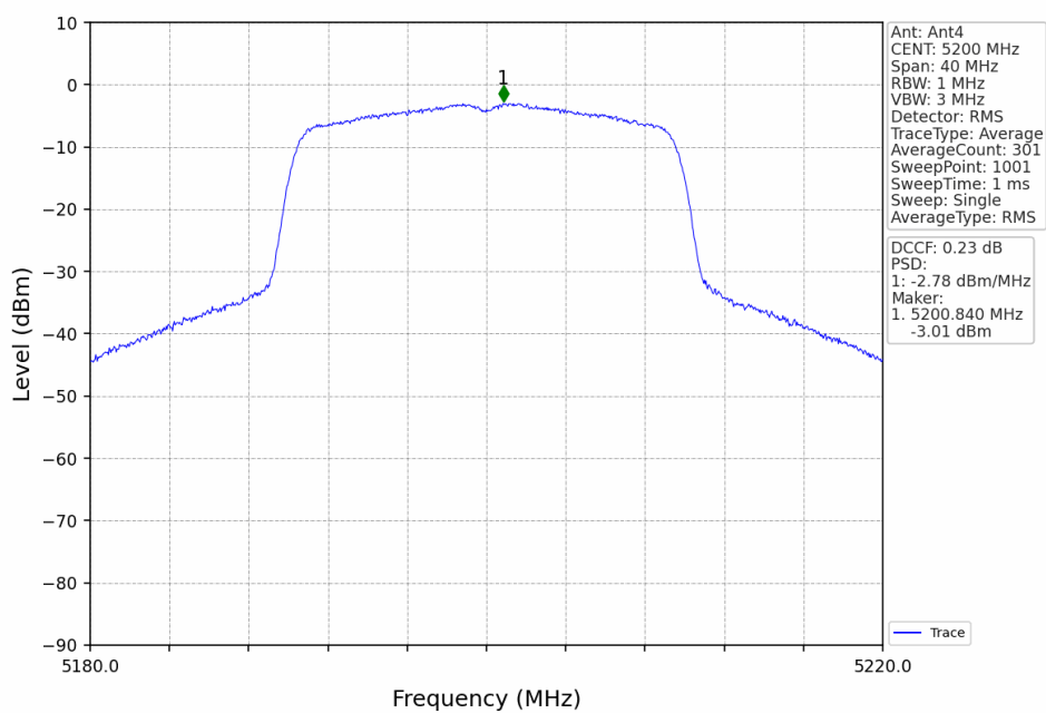
802.11ax(HEW20)_MCH_5200MHz_RU242_Left_Ant4_NTNV
