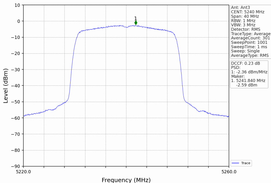
802.11ax(HEW20)_HCH_5240MHz_RU242_Left_Ant3_NTNV
