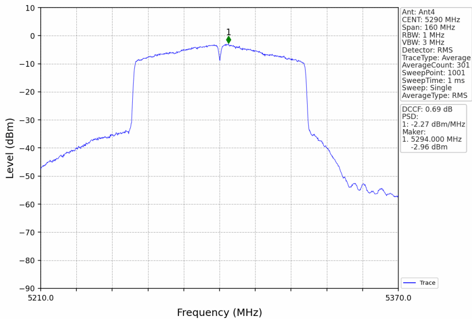
802.11ac(VHT80)_MCH_5290MHz_Ant4_NTNV
