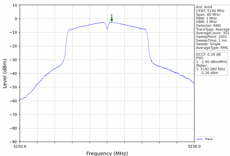
802.11ac(VHT40)_LCH_5190MHz_Ant4_NTNV
