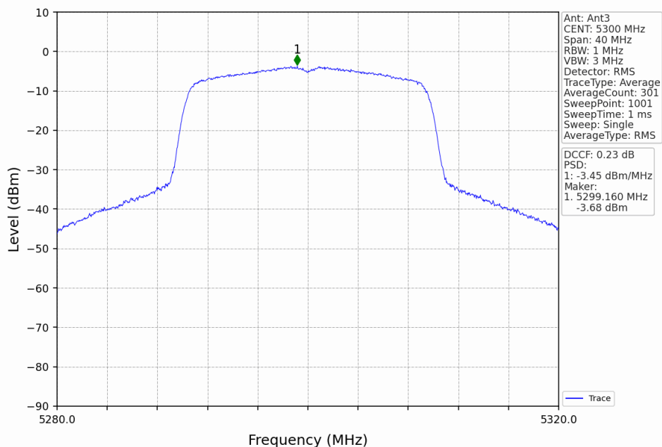
802.11ax(HEW20)_MCH_5300MHz_RU242_Left_Ant3_NTNV
