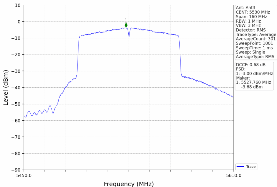
802.11ac(VHT80)_LCH_5530MHz_Ant3_NTNV
