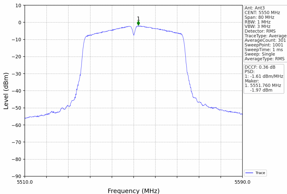
802.11ac(VHT40)_MCH_5550MHz_Ant3_NTNV
