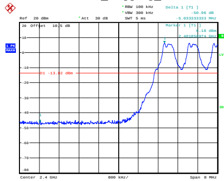
GFSK_Hopping_Lower
