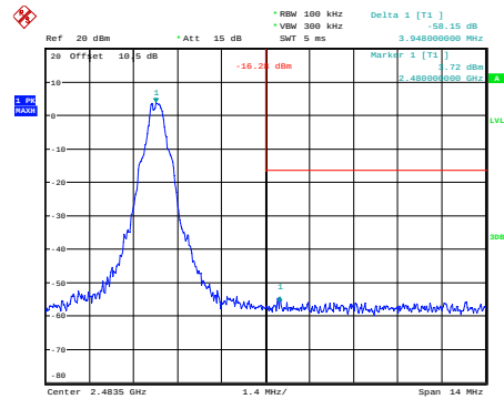
GFSK_High
