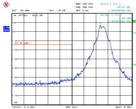
GFSK_Low
