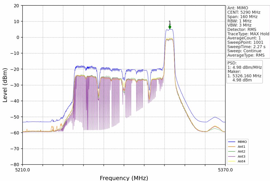
802.11ax(HEW80)_MCH_5290MHz_RU52+26_Right_MIMO_NTNV
