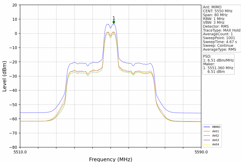
802.11ax(HEW40)_MCH_5550MHz_RU52_Mid_MIMO_NTNV
