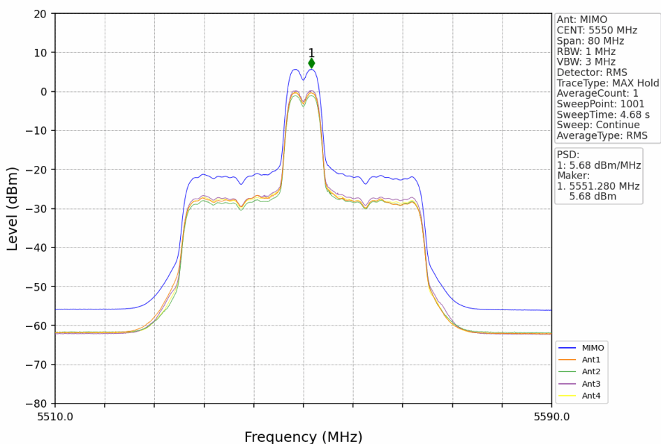
802.11be(EHT40)_MCH_5550MHz_RU52_Mid_MIMO_NTNV
