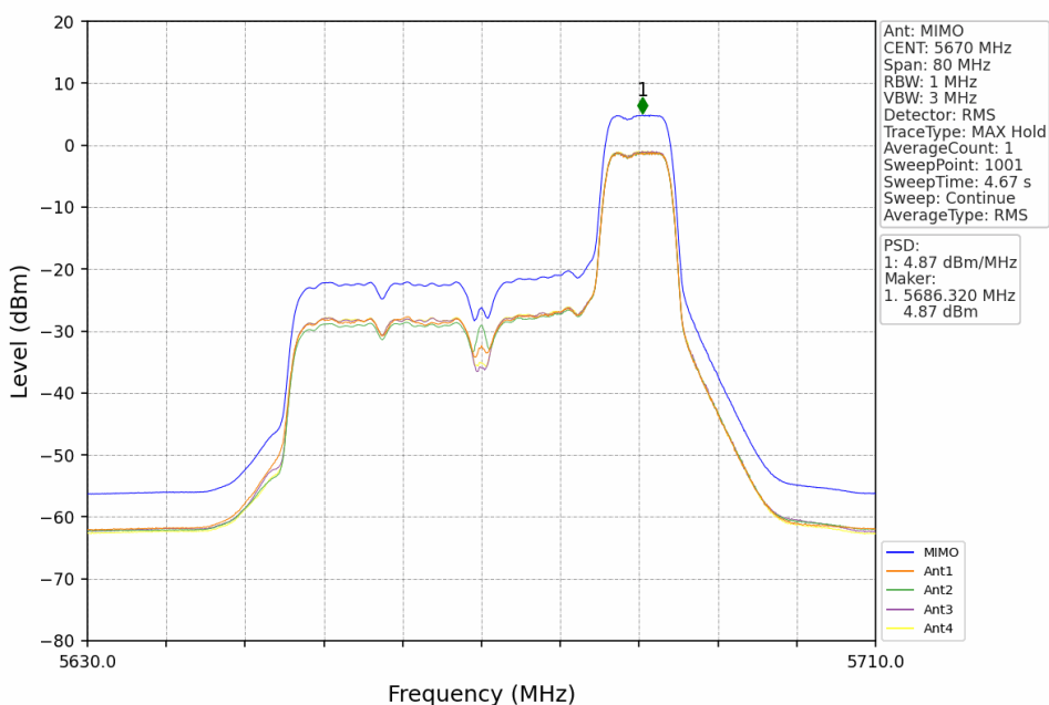
802.11ax(HEW40)_HCH_5670MHz_RU52+26_Right_MIMO_NTNV
