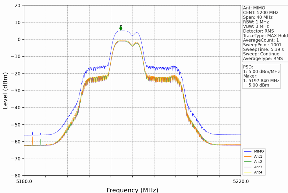
802.11be(EHT20)_MCH_5200MHz_RU52+26_Mid_MIMO_NTNV
