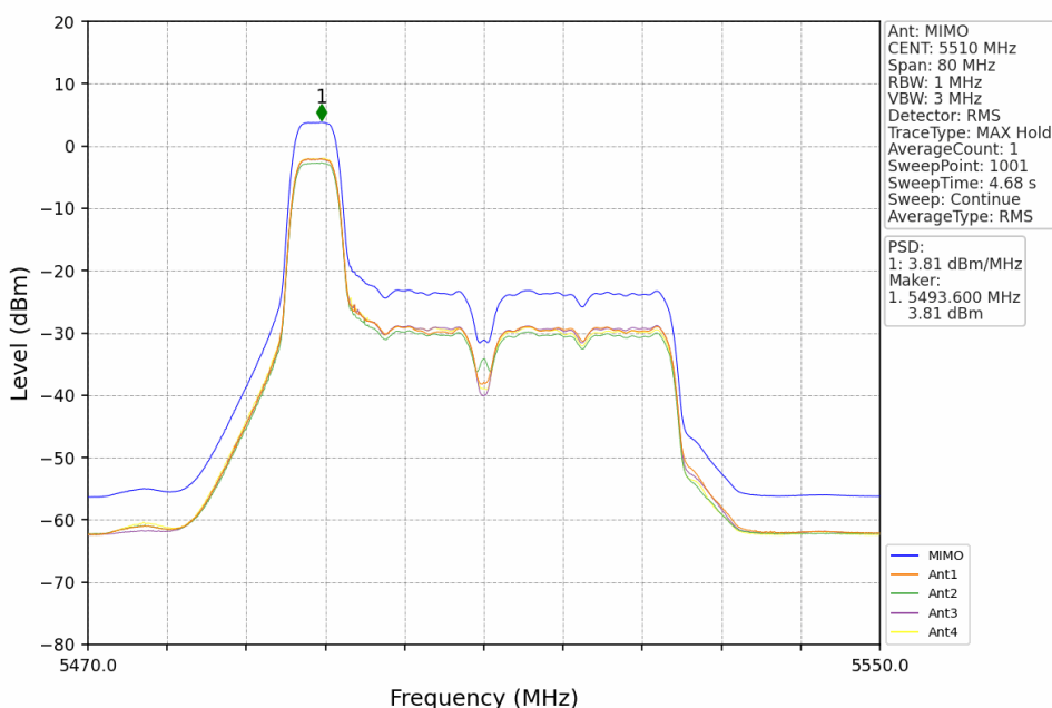
802.11ax(HEW40)_LCH_5510MHz_RU52+26_Left_MIMO_NTNV
