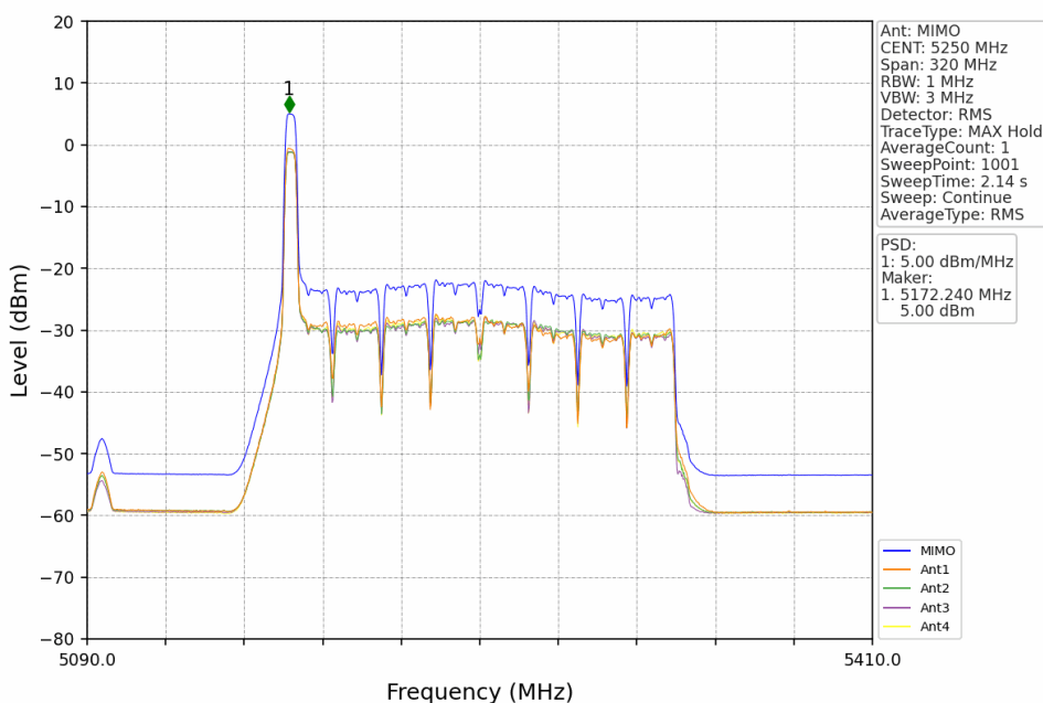
802.11ax(HEW160)_MCH_5250MHz_RU52+26_Left_MIMO_NTNV
