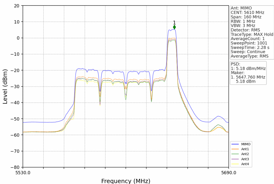
802.11ax(HEW80)_HCH_5610MHz_RU52+26_Right_MIMO_NTNV
