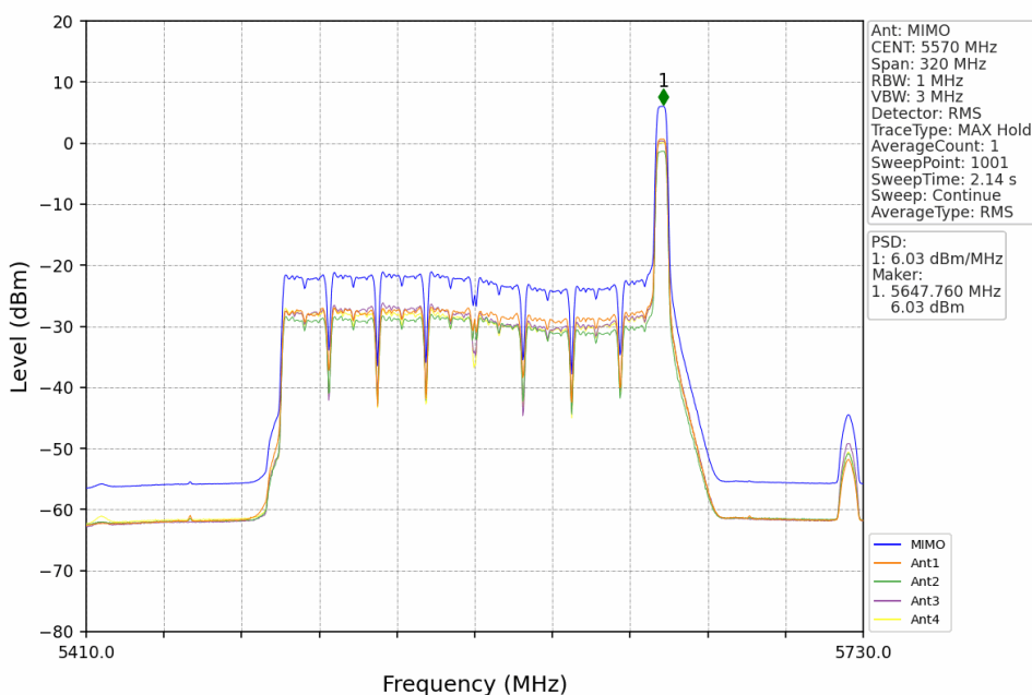
802.11ax(HEW160)_MCH_5570MHz_RU52_Right_MIMO_NTNV
