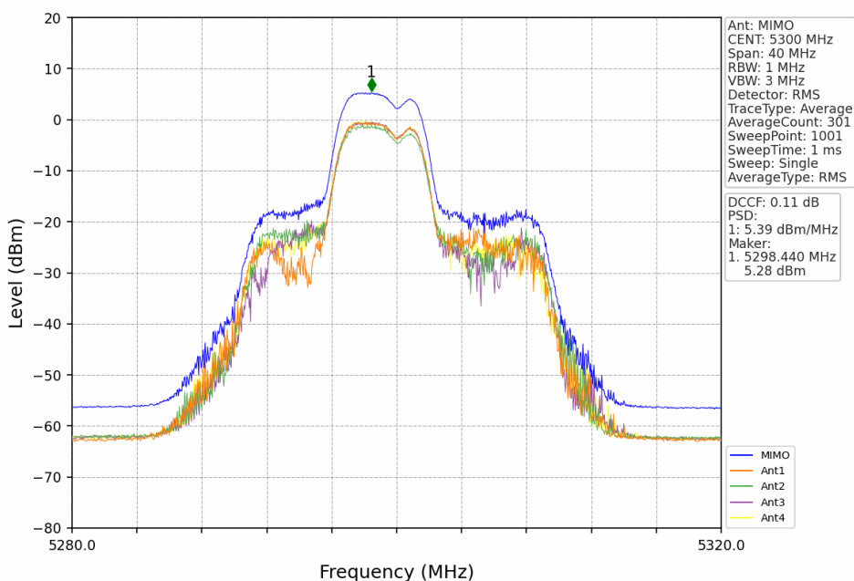
802.11be(EHT20)_MCH_5300MHz_RU52_Mid_MIMO_NTNV
