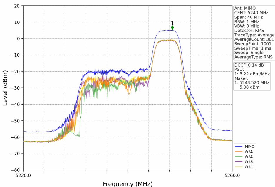
802.11be(EHT20)_HCH_5240MHz_RU52_Right_MIMO_NTNV
