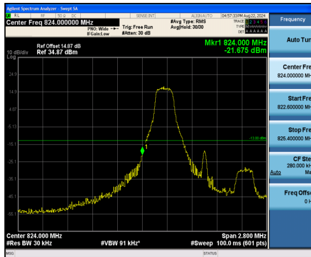
Band26-1.4MHz-QPSK-26797-1RB#5
