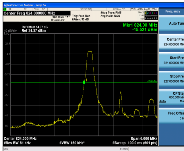
Band26-3MHz-16QAM-26805-1RB#14
