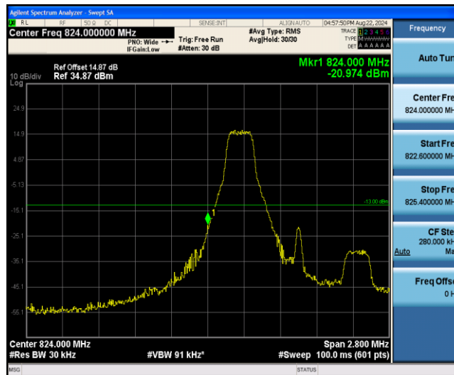
Band26-1.4MHz-16QAM-26797-1RB#5
