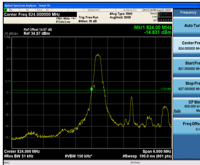
Band26-3MHz-QPSK-26805-1RB#14
