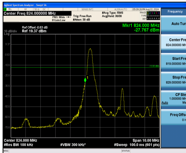
Band26-5MHz-QPSK-26815-1RB#24
