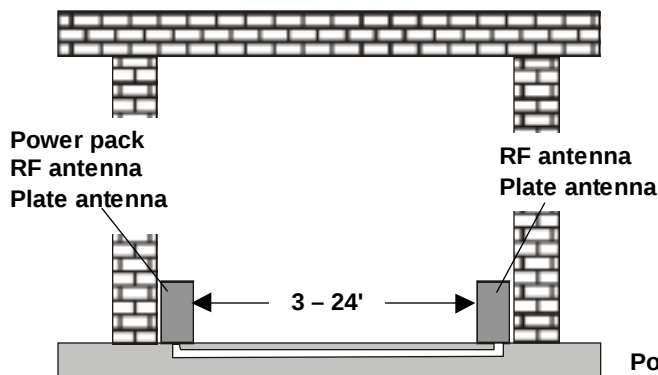
Figure 3. Pedestal with plates
