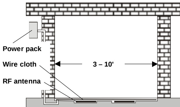
Figure 8. Sensormat II with wire cloth
