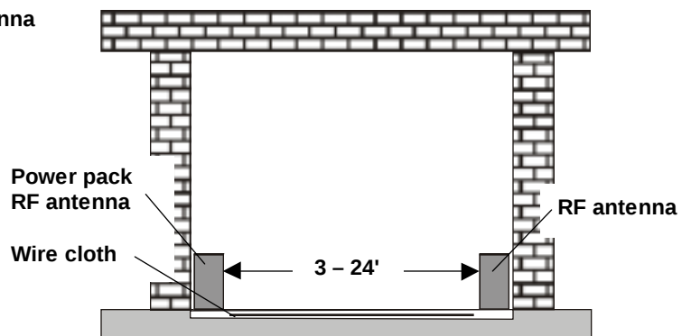
Figure 4. Pedestal with wire cloth
