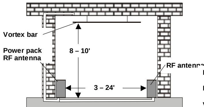
Figure 5. Pedestal with vortex
