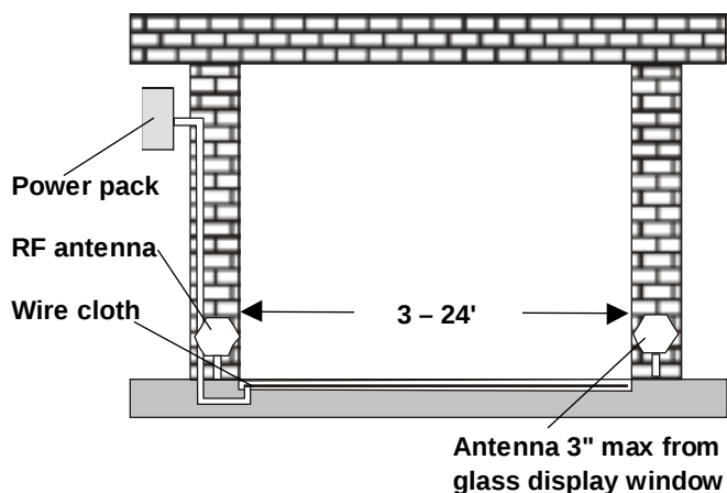
Figure 7. Micromax with wire cloth
