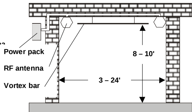
Figure 6. Micromax with vortex
