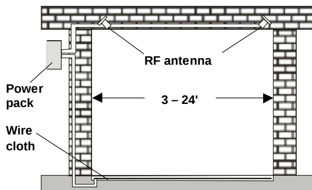
Figure 2. Concealed antennas with wire cloth
