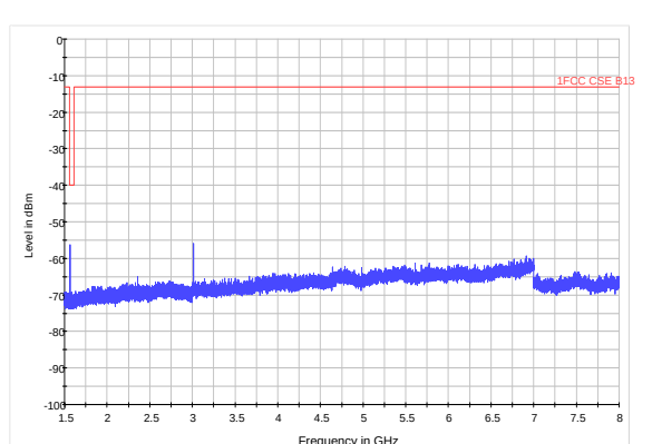
LTE Band 13 5MHz CH-High 1.5GHz~8GHz
