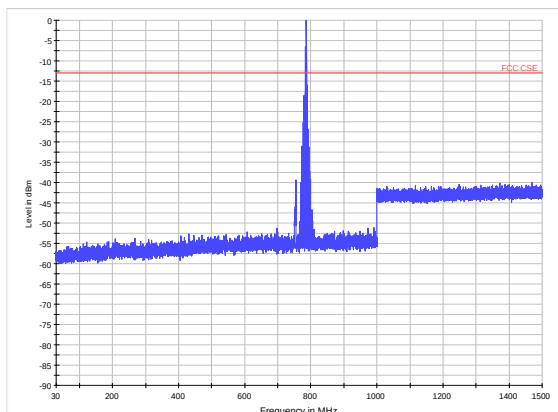
LTE Band 13 5MHz CH-High 30MHz~1.5GHz
