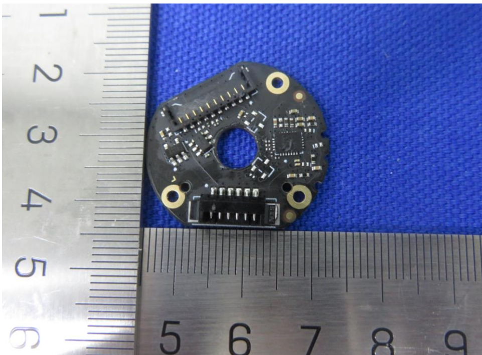
(PCB Photo of Axis-P)
