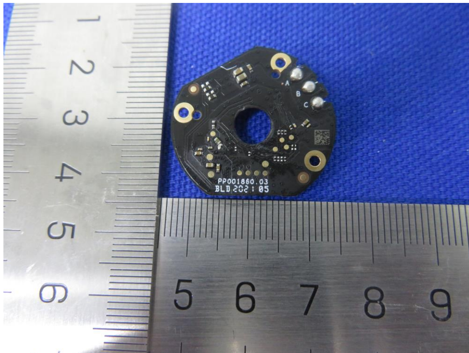
(PCB Photo of Axis-P)
