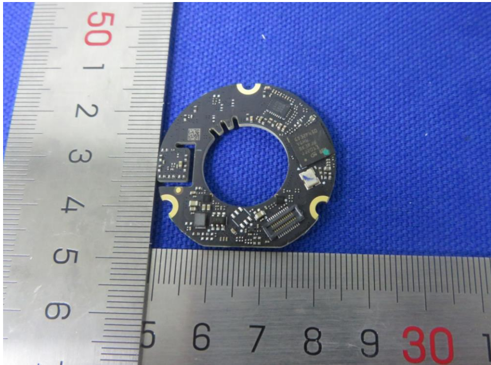
(PCB Photo of Axis-R)
