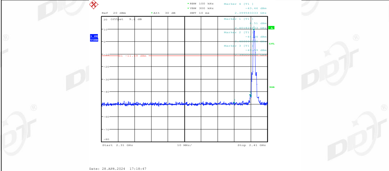
2DH5 Left side Low 2402
