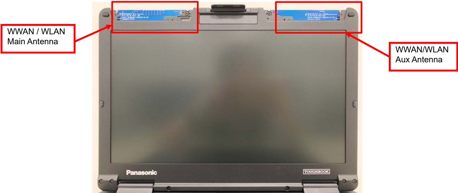
<Front view>
