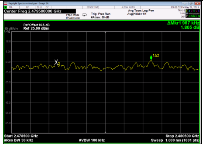
pi/4DQPSK,Hopping2DH5,2478.5~2480.5
