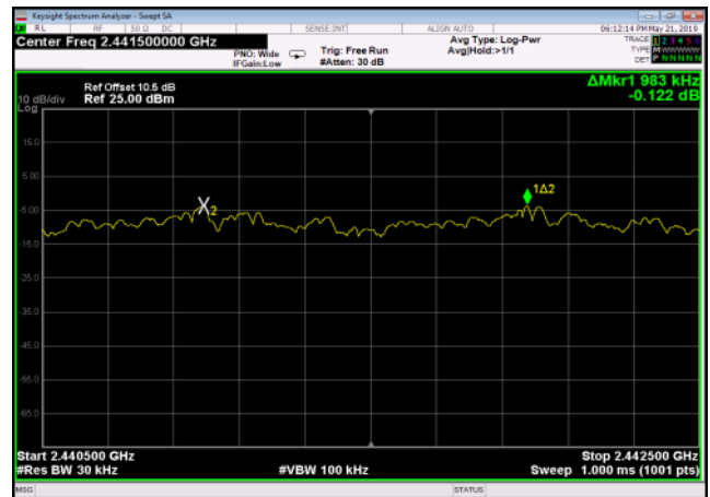
8DPSK,Hopping3DH5,2440.5~2442.5
