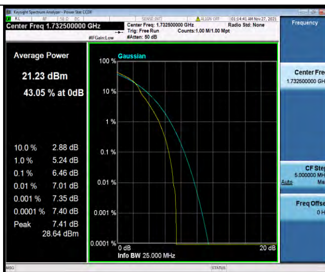
Band4-20MHz-16QAM-20175-27RB#0
