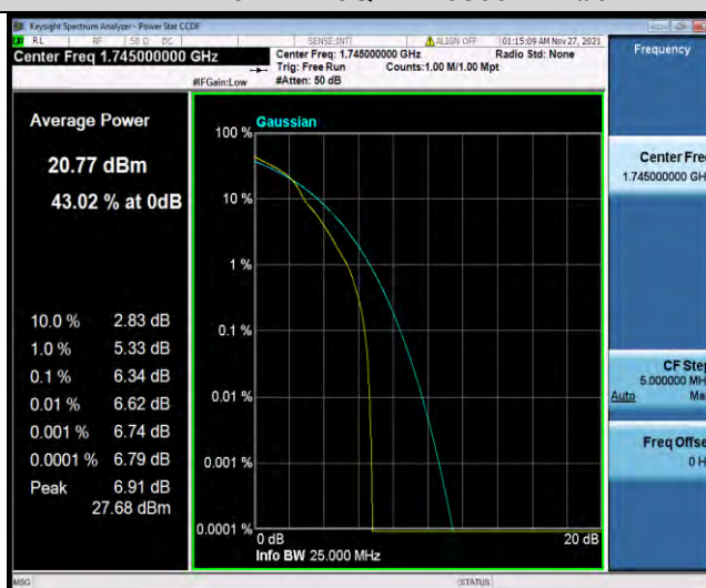
Band4-20MHz-16QAM-20300-27RB#0
