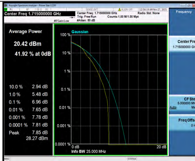
Band4-10MHz-16QAM-20000-27RB#0
