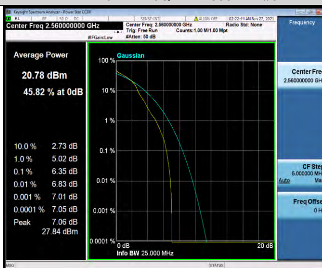
Band7-20MHz-16QAM-21350-27RB#0
