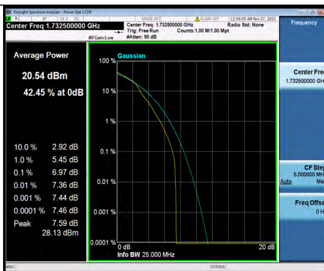
Band4-10MHz-16QAM-20175-27RB#0
