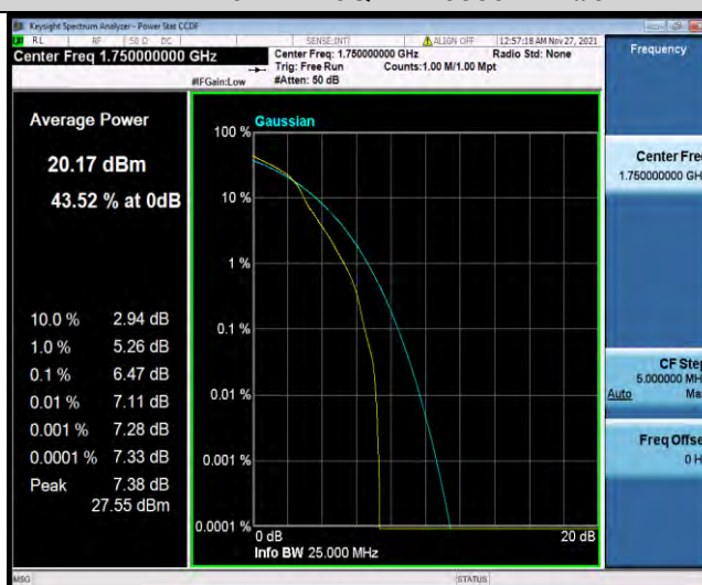
Band4-10MHz-16QAM-20350-27RB#0
