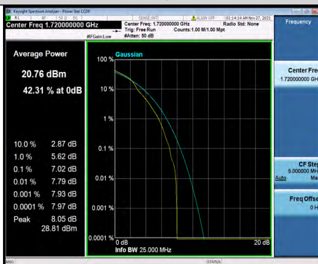
Band4-20MHz-16QAM-20050-27RB#0
