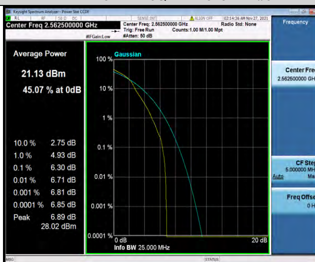
Band7-15MHz-16QAM-21375-27RB#0
