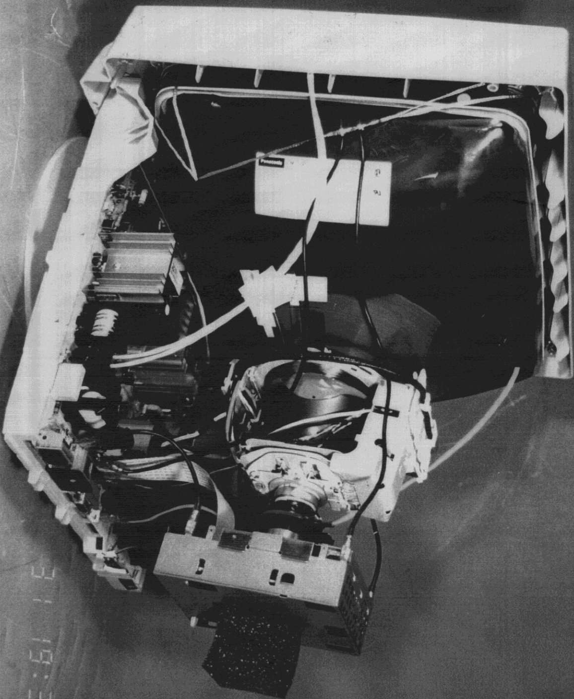
Fig.3. Inside view (without shield case) of VCR model 133 **
