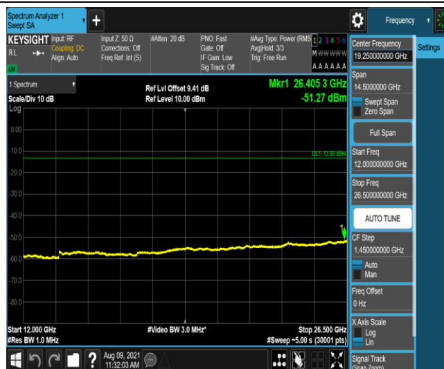
Band25-3MHz-16QAM-26365-1-0-Low-12000-26500--51.27-PASS
