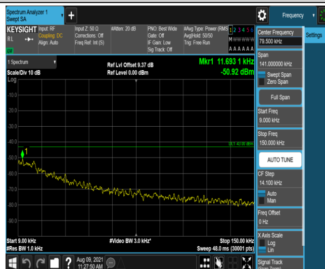
Band25-3MHz-16QAM-26055-1-0-Low-0.009-0.15--50.93-PASS
