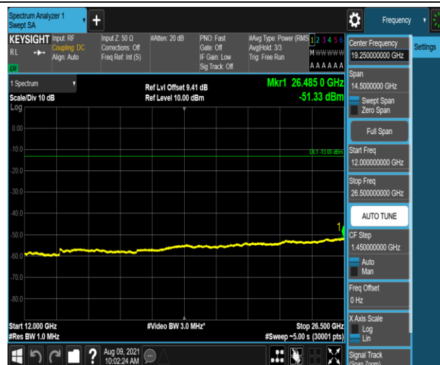
Band25-1.4MHz-16QAM-26365-1-0-Low-12000-26500--51.33-PASS
