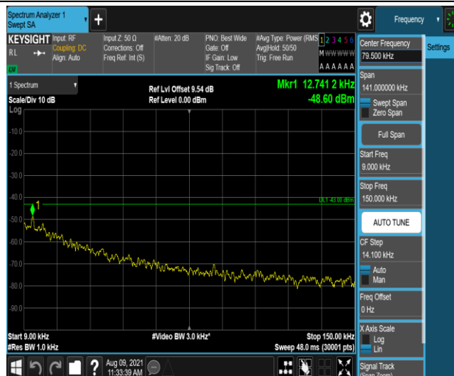
Band25-3MHz-16QAM-26675-1-0-High-0.009-0.15--48.6-PASS
