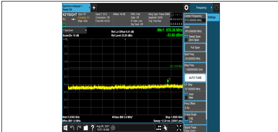
Band25-1.4MHz-16QAM-26365-1-0-Low-30-1000--33.6-PASS
