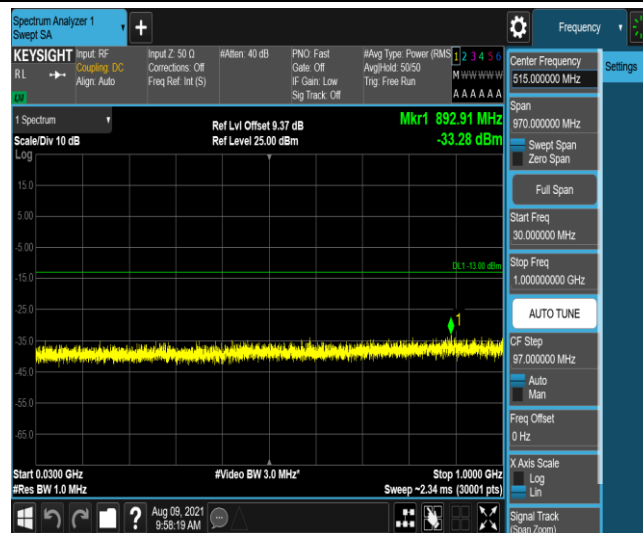
Band25-1.4MHz-16QAM-26047-1-0-Low-30-1000--33.28-PASS
