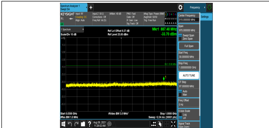
Band25-3MHz-16QAM-26055-1-0-Low-30-1000--33.7-PASS
