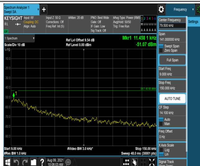
Band25-1.4MHz-16QAM-26683-1-0-High-0.009-0.15--51.07-PASS
