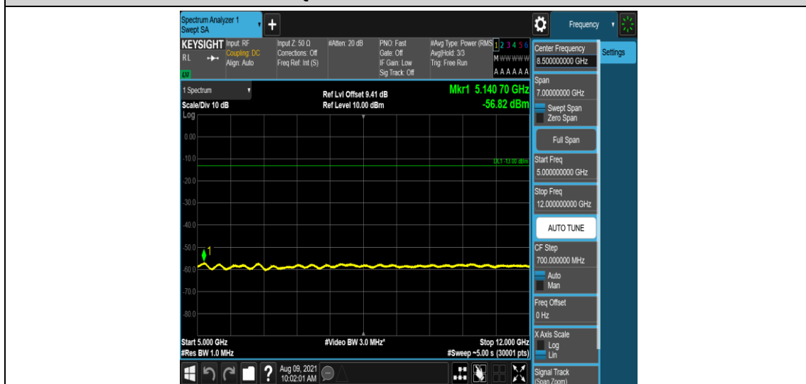
Band25-1.4MHz-16QAM-26365-1-0-Low-5000-12000--56.82-PASS
