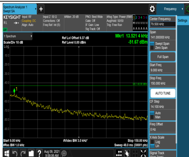
Band25-1.4MHz-16QAM-26047-1-0-Low-0.009-0.15--51.67-PASS
