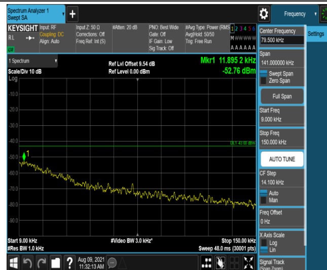
Band25-3MHz-QPSK-26675-1-0-High-0.009-0.15--52.76-PASS
