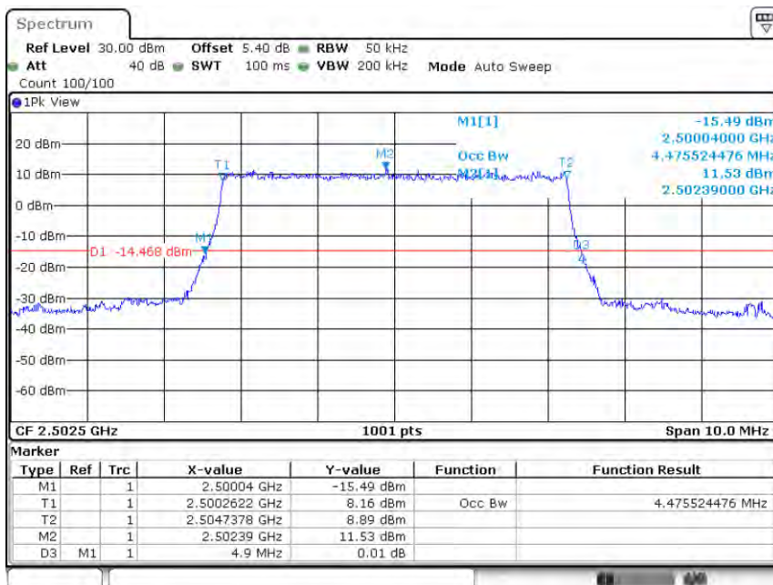
Band7-5MHz-QPSK-20775-25RB#0-4.476
