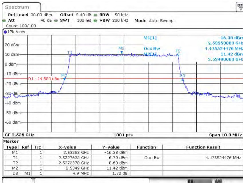
Band7-5MHz-QPSK-21100-25RB#0-4.476
