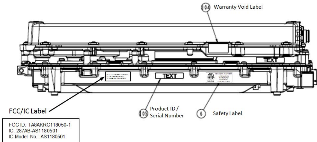
Figure 1: ARUS 32 B4 Label Detail
