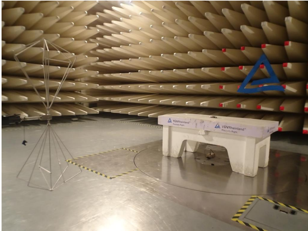
Test Setup:30MHz-200MHz
