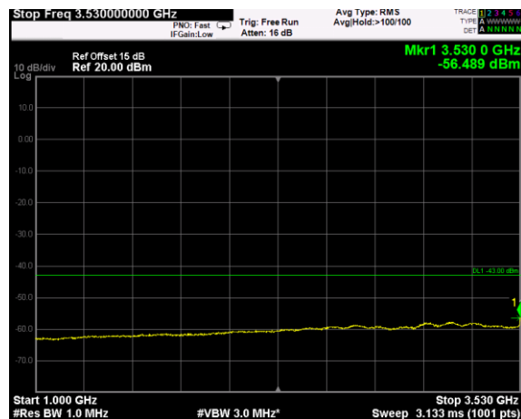
Channel: MIDDLE, Modulation: 16QAM, BW=20MHz, Range: 1GHz - 3530MHz
