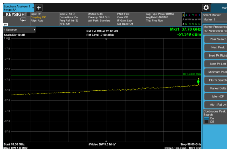
Channel: MIDDLE, Modulation: QPSK, BW=20MHz, Range: 18GHz - 38GHz
