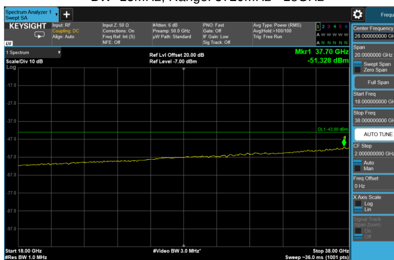
Channel: MIDDLE, Modulation: 16QAM, BW=15MHz, Range: 18GHz - 38GHz
