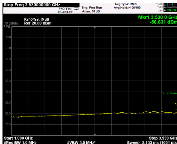
Channel: MIDDLE, Modulation: QPSK, BW=15MHz, Range: 1GHz - 3530MHz
