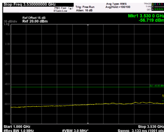
Channel: TOP, Modulation: 16QAM, BW=5 MHz, Range: 1GHz - 3530MHz
