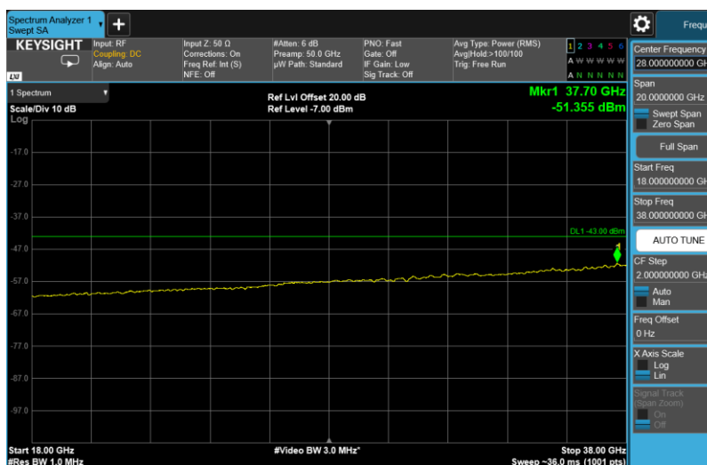
Channel: BOTTOM, Modulation: 16QAM, BW=15MHz, Range: 18GHz - 38GHz
