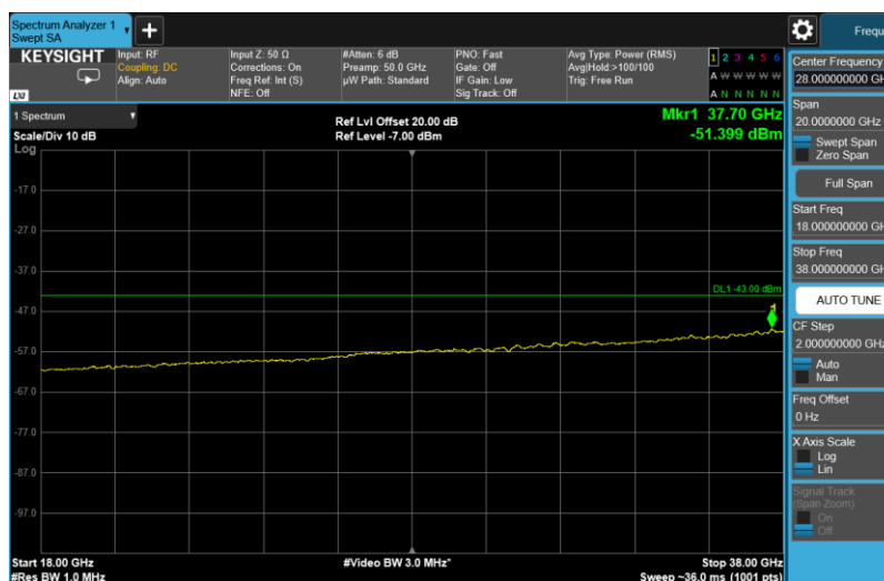
Channel: MIDDLE, Modulation: QPSK, BW=15MHz, Range: 18GHz - 38GHz
