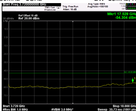
Channel: BOTTOM, Modulation: 16QAM, BW=15MHz, Range: 3720MHz - 18GHz
