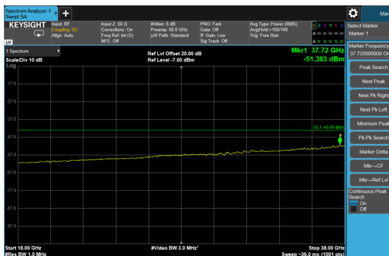
Channel: BOTTOM, Modulation: QPSK, BW=20MHz, Range: 18GHz - 38GHz
