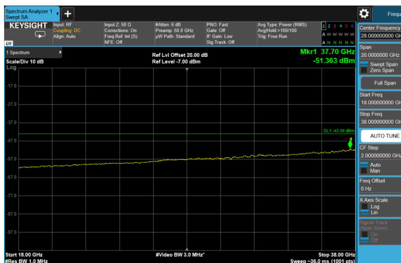
Channel: TOP, Modulation: 256QAM, BW=15MHz, Range: 18GHz - 38GHz
