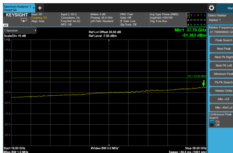
Channel: BOTTOM, Modulation: 256QAM, BW=10MHz, Range: 18GHz - 38GHz
