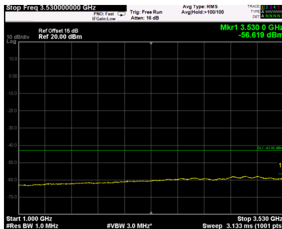
Channel: BOTTOM, Modulation: 16QAM, BW=15MHz, Range: 1GHz - 3530MHz
