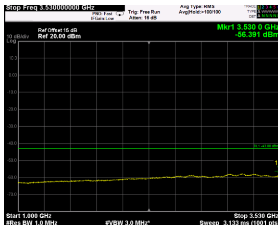
Channel: BOTTOM, Modulation: QPSK, BW=10MHz, Range: 1GHz - 3530MHz
