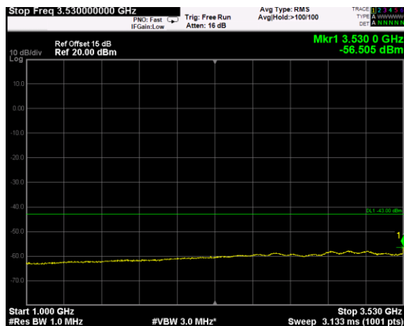
Channel: MIDDLE, Modulation: 16QAM, BW=10MHz, Range: 1GHz - 3530MHz
