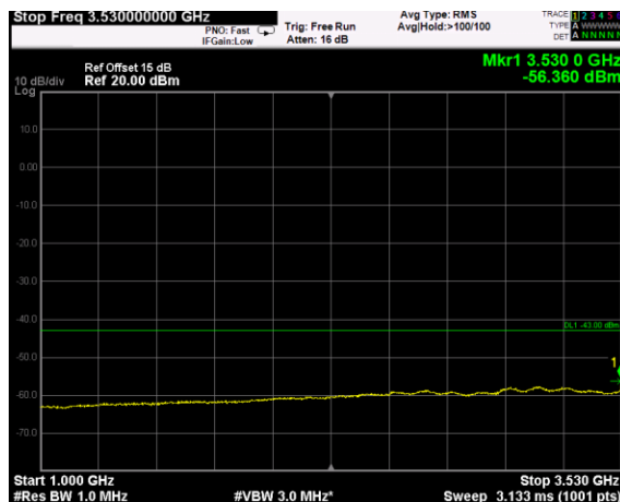
Channel: MIDDLE, Modulation: 64QAM, BW=20MHz, Range: 1GHz - 3530MHz
