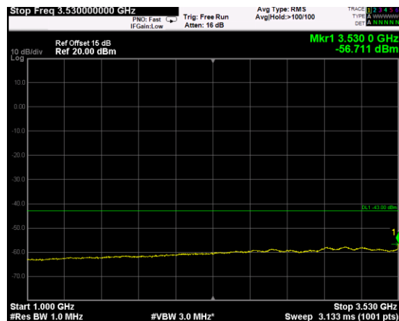
Channel: TOP, Modulation: 256QAM, BW=15MHz, Range: 1GHz - 3530MHz
