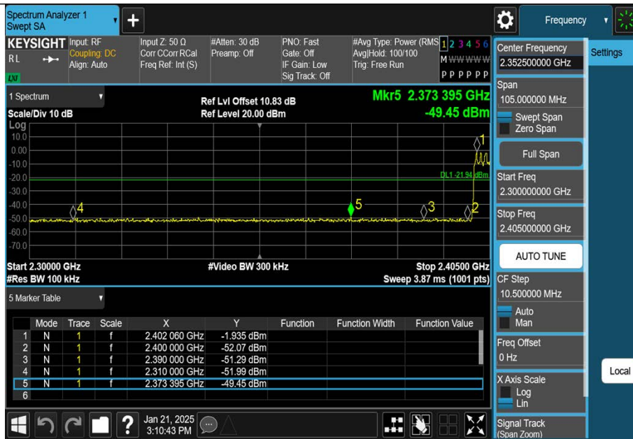
3DH5-Ant1-Hop_2402-PASS
