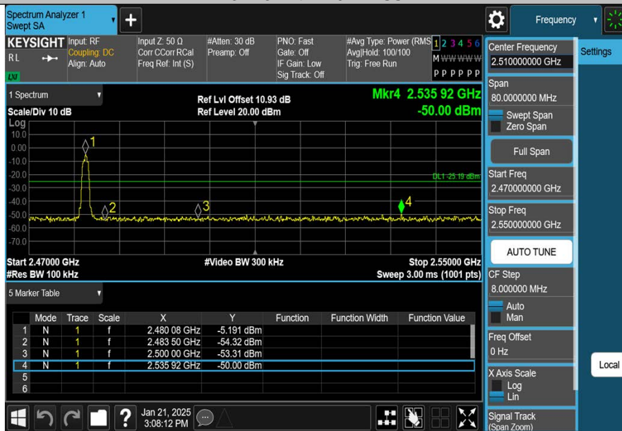
3DH5-Ant1-2480-PASS
