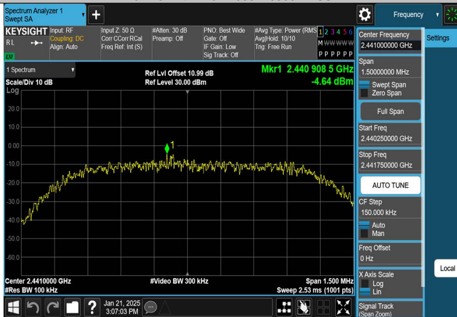
3DH5-Ant1-2441-0~Reference-PASS
