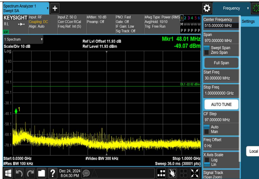
2DH5-Ant1-2480-30~1000-PASS
