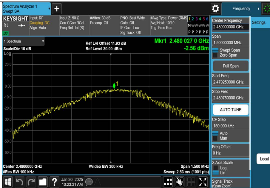
DH5-Ant1-2480-0~Reference-PASS
