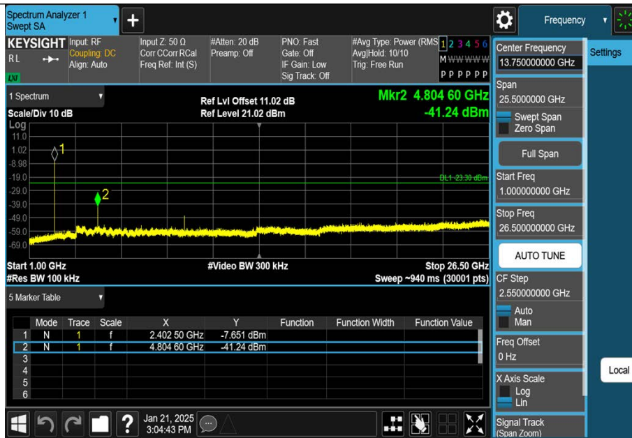
3DH5-Ant1-2402-1000~26500-PASS
