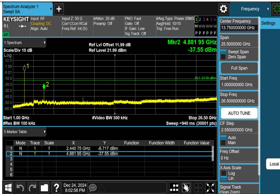
2DH5-Ant1-2441-1000~26500-PASS
