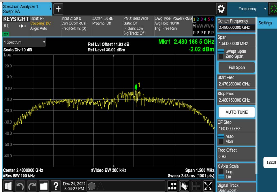
2DH5-Ant1-2480-0~Reference-PASS
