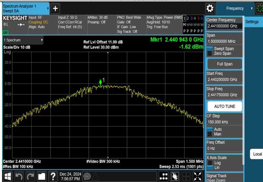
DH5-Ant1-2441-0~Reference-PASS
