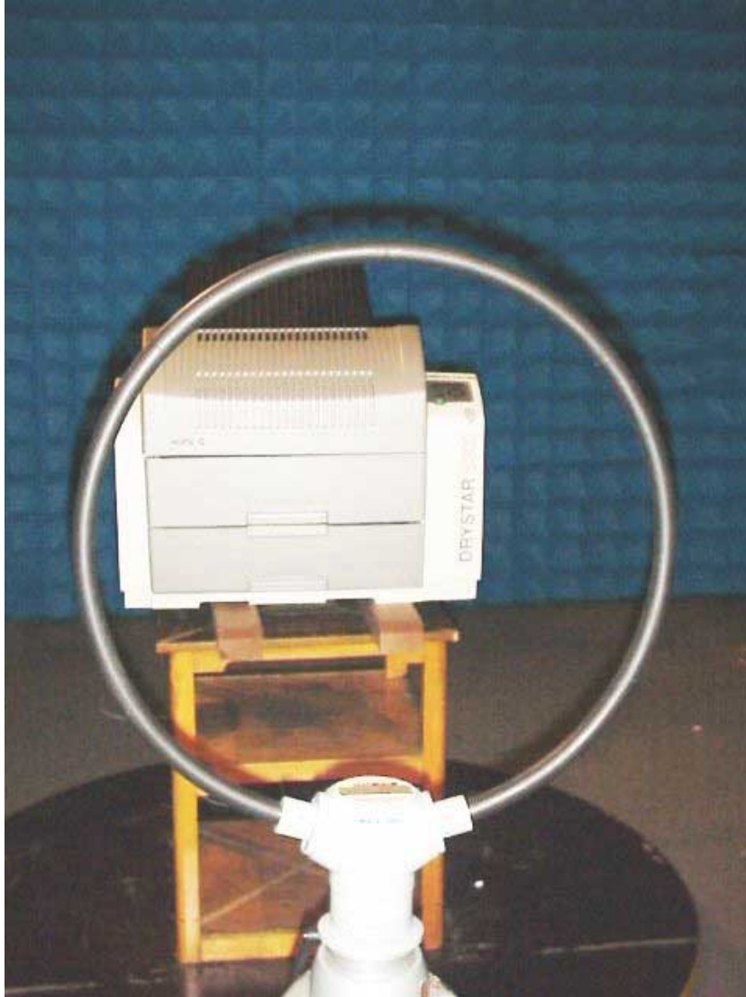
photo 3 : radiated emission set-up (band 13.56MHz)
