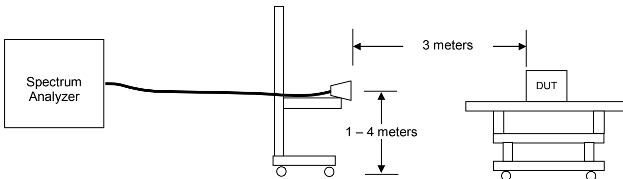
Figure C.6-1 - Setup Drawing
