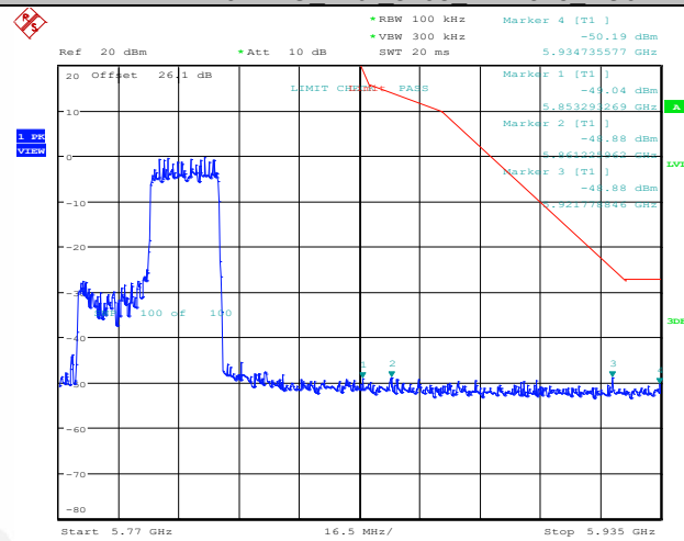
11AX40MIMO Ant2 5795 242Tone RU62
