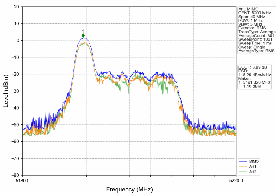
802.11ax(HEW20)_MCH_5200MHz_RU26_Left_MIMO_NTNV
