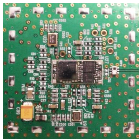
EUT – WLAN Radio without Shielding
