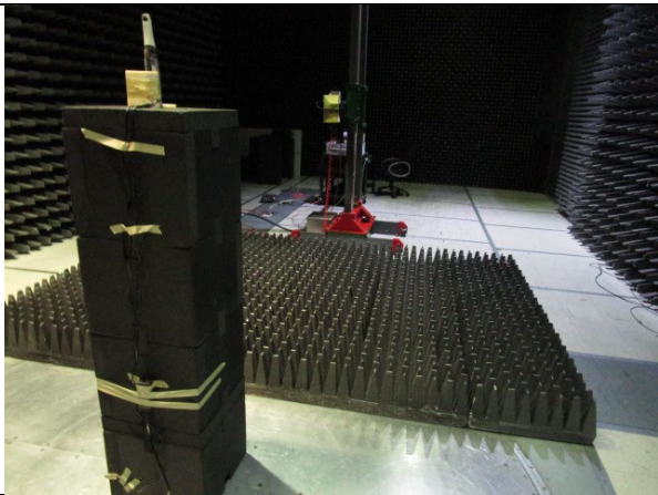
Radiated Emissions above 1 GHz back
