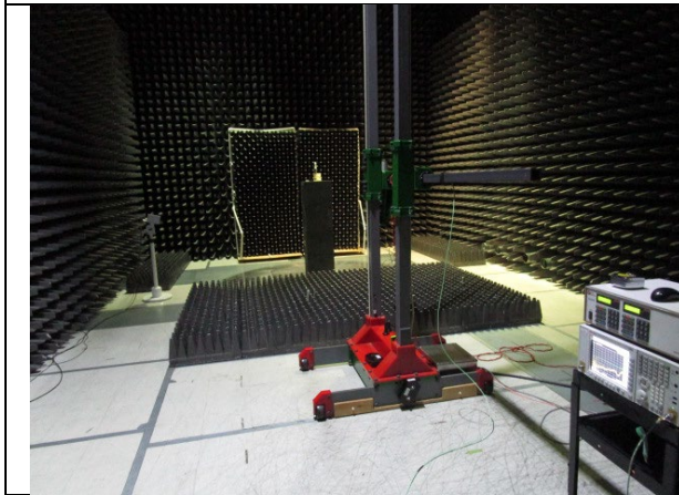
Radiated Emissions above 1 GHz front
