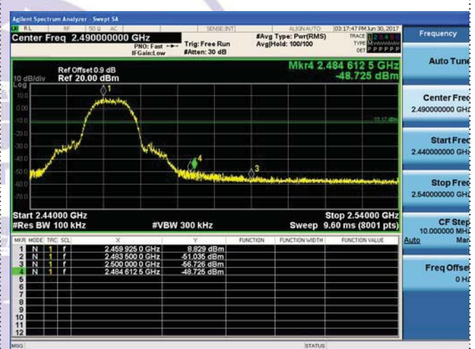
Right bandedge
