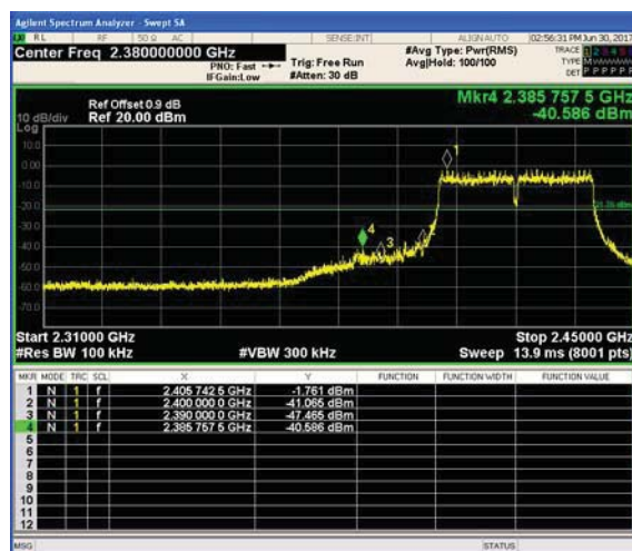
Left bandedge
