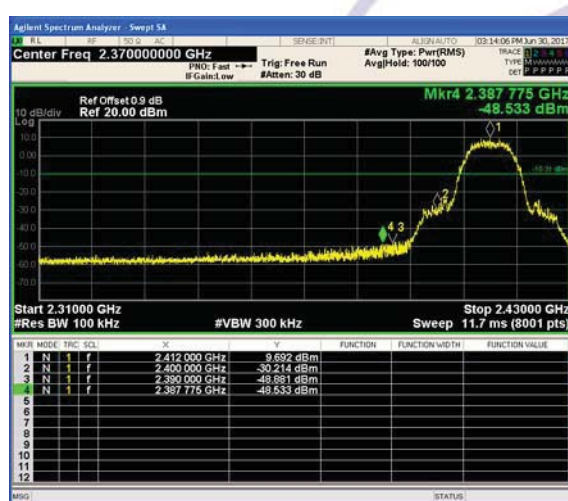
Left bandedge
