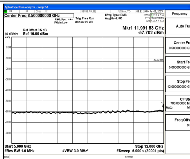
Band25-15MHz-16QAM-26365-1-0-Low-5000-12000--57.7-PASS
