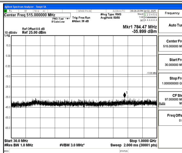
Band25-15MHz-16QAM-26115-1-0-Low-30-1000--35.9-PASS
