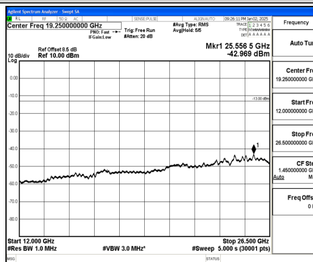
Band25-15MHz-QPSK-26115-1-0-Low-12000-26500--42.97-PASS
