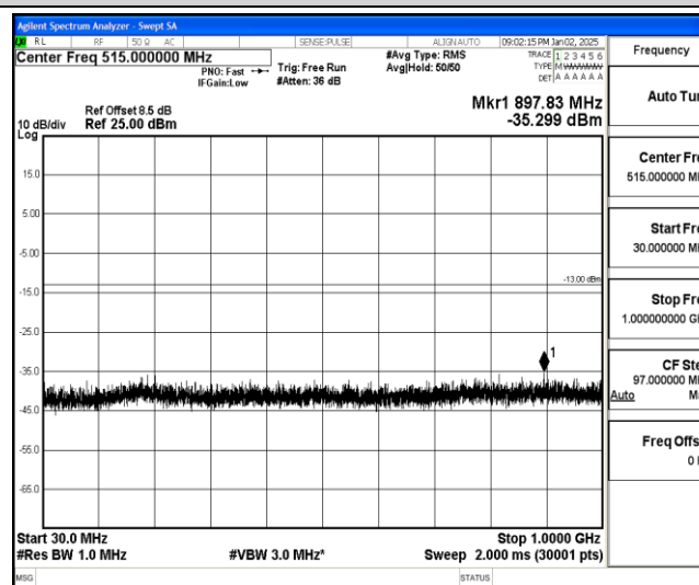
Band25-10MHz-16QAM-26090-1-0-Low-30-1000--35.3-PASS
