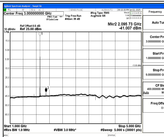
Band25-10MHz-16QAM-26640-1-0-High-1000-5000--41.01-PASS
