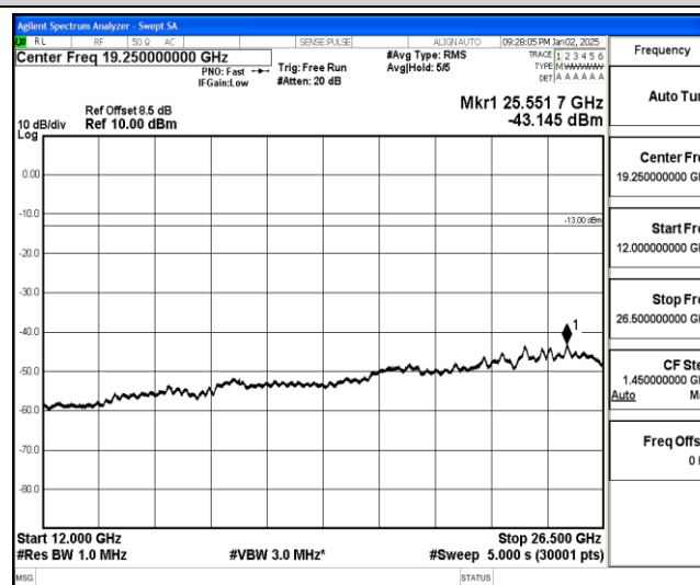
Band25-15MHz-16QAM-26115-1-0-Low-12000-26500--43.15-PASS
