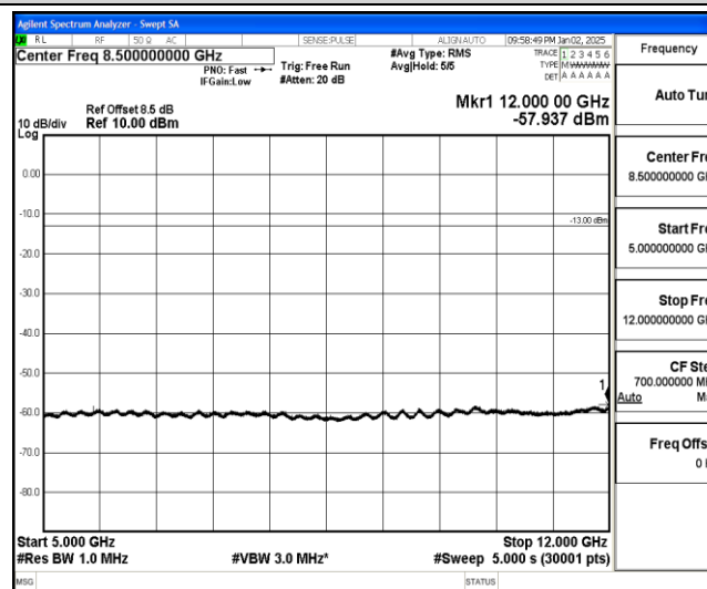
Band25-20MHz-16QAM-26365-1-0-Low-5000-12000--57.94-PASS
