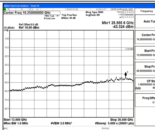
Band25-20MHz-16QAM-26140-1-0-Low-12000-26500--43.32-PASS
