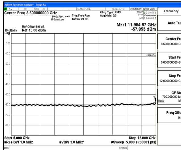
Band25-20MHz-QPSK-26140-1-0-Low-5000-12000--57.85-PASS
