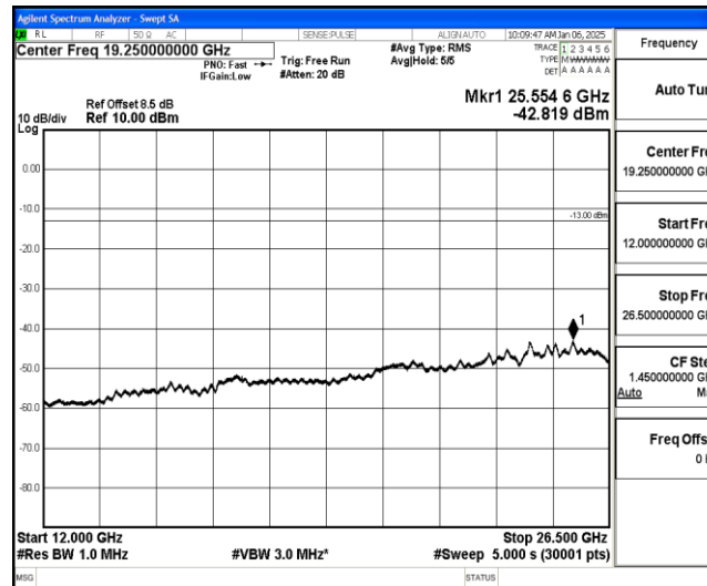
Band25-10MHz-16QAM-26365-1-0-Low-12000-26500--42.82-PASS
