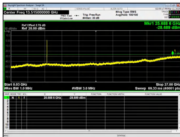
802.11ax40 on channel 151
