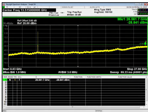
802.11ax20 on channel 149
