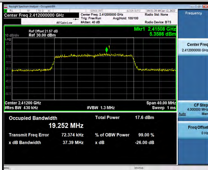
11AX20_RU_Ant2_2412_242Tone_RU61
