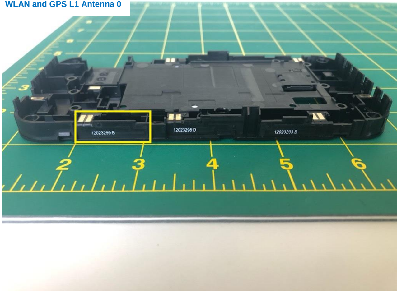
WLAN and GPS L1 Antenna 0
