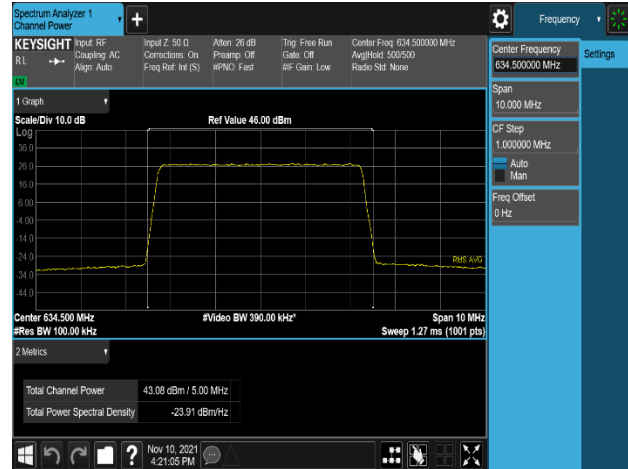
Plot 8-22. Conducted Average Output Power Plot (NR_n71_5M_256QAM - Mid Channel, Port 1)
