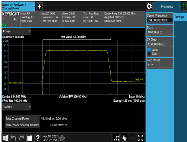
Plot 8-23. Conducted Average Output Power Plot (NR_n71_5M_256QAM - Mid Channel, Port 2)
