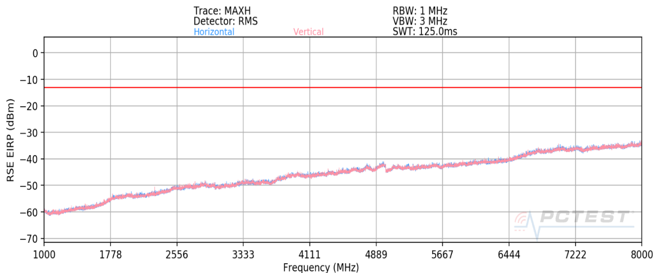
Plot 8-64. Radiated spurious emission Plot_1 GHz to 8 GHz (NR_n71_10M_QPSK - High Channel)
