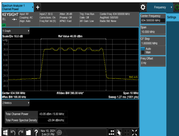
Plot 8-13. Conducted Average Output Power Plot (NR_n71_5M_16QAM - Mid Channel, Port 0)
