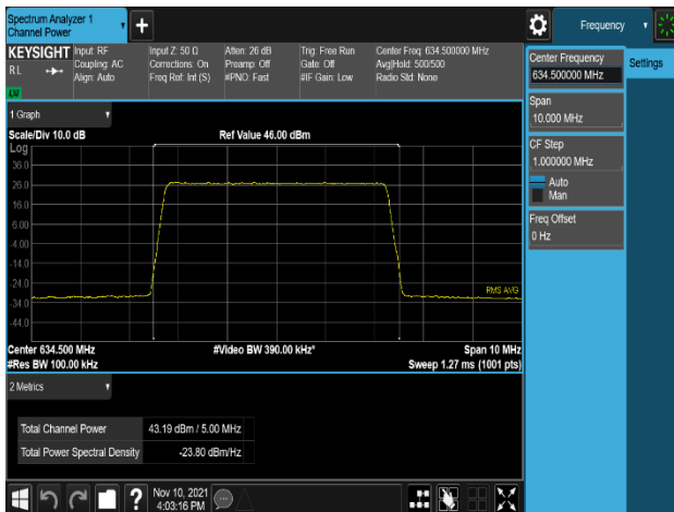
Plot 8-19. Conducted Average Output Power Plot (NR_n71_5M_64QAM - Mid Channel, Port 2)
