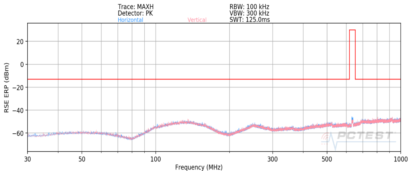
Plot 8-61. Radiated spurious emission Plot_30 MHz to 1000 MHz (NR_n71_10M_QPSK - Mid Channel)
