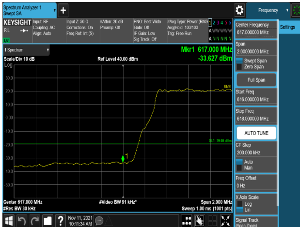
Plot 8-45. Lower Band Edge Emission Plot (NR_n71_10M_QPSK – Low Channel, Port 3)
