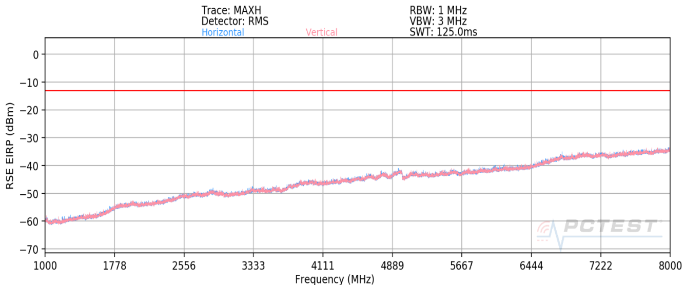
Plot 8-60. Radiated spurious emission Plot_1 GHz to 8 GHz (NR_n71_10M_QPSK - Low Channel)
