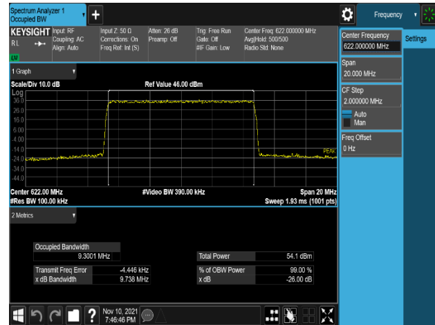
Plot 8-8. Occupied Bandwidth Plot (LTE_n71_10M_256QAM - Low Channel, Port 1)
