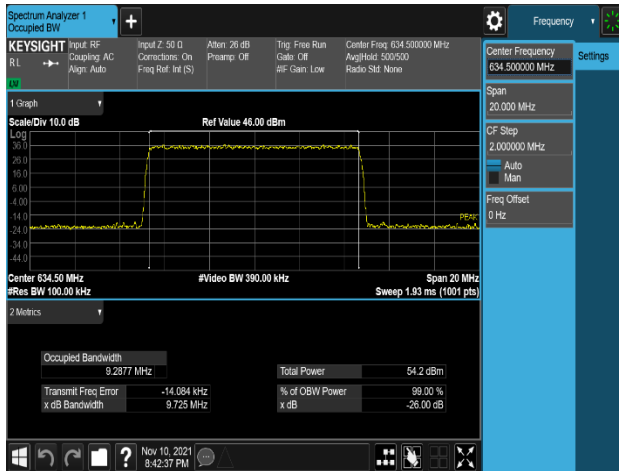
Plot 8-7. Occupied Bandwidth Plot (LTE_n71_10M_64QAM - Mid Channel, Port 1)
