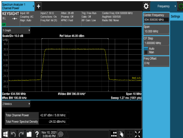
Plot 8-11. Conducted Average Output Power Plot (NR_n71_5M_QPSK - Mid Channel, Port 2)
