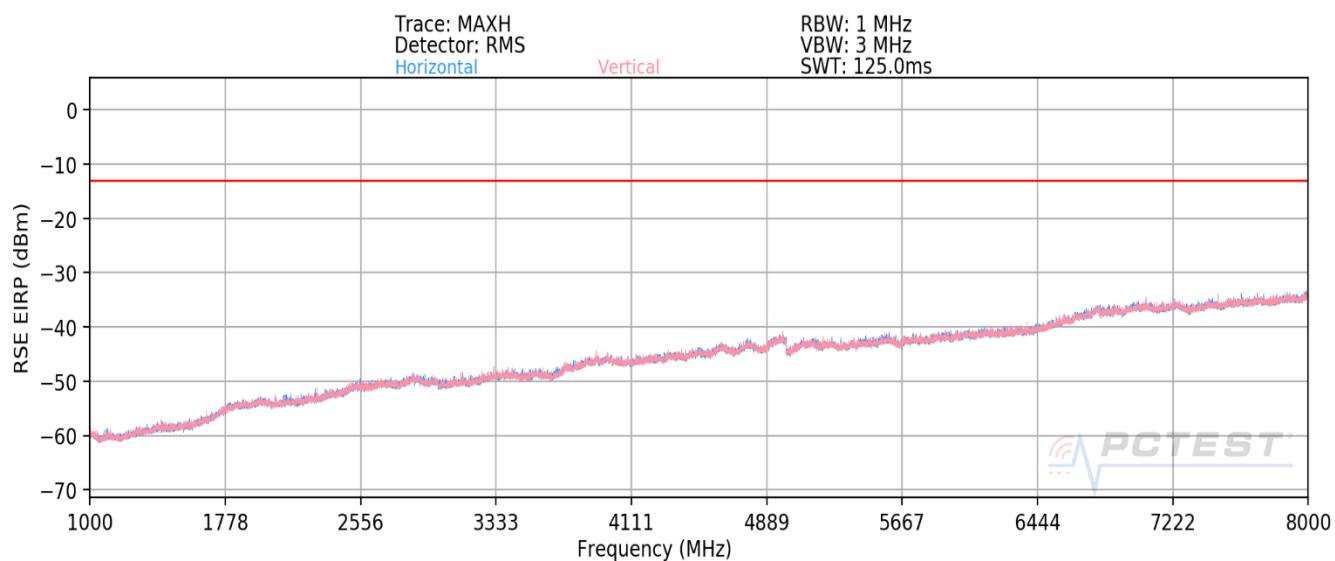
Plot 8-62. Radiated spurious emission Plot_1 GHz to 8 GHz (NR_n71_10M_QPSK - Mid Channel)
