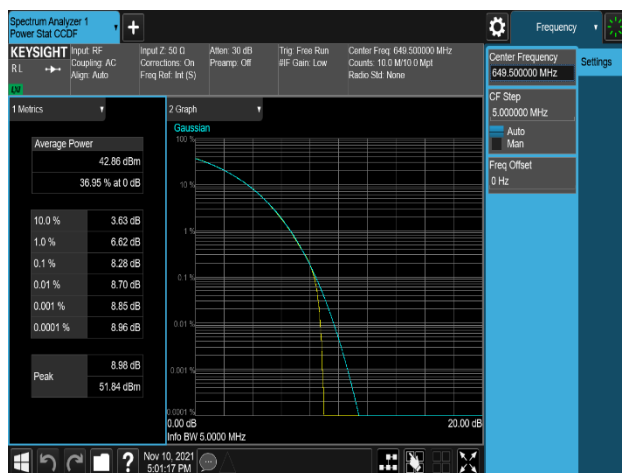
Plot 8-41. Peak To Average Power Ratio Plot (NR_n71_5M_16QAM - High Channel, Port 0)
