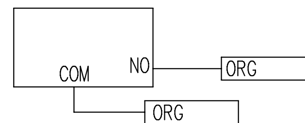
DOOR SENSING SWITCH (SECONDARY INTERLOCK SWITCH)
