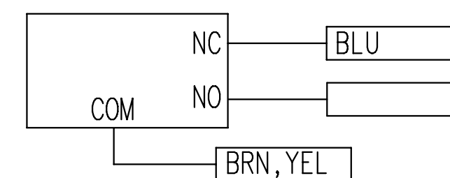
MONITOR INTERLOCK SWITCH
