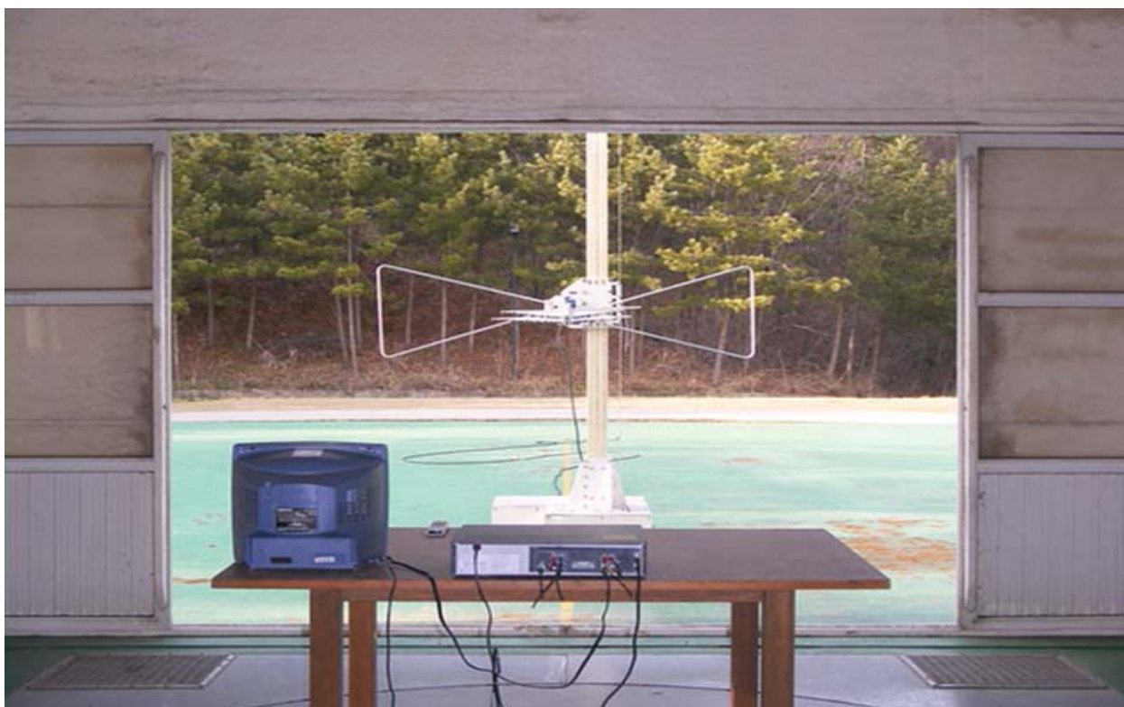
Rear View
