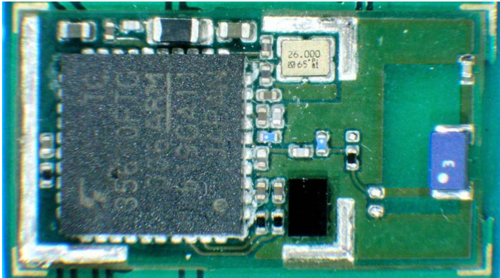
Module without cover, front view
