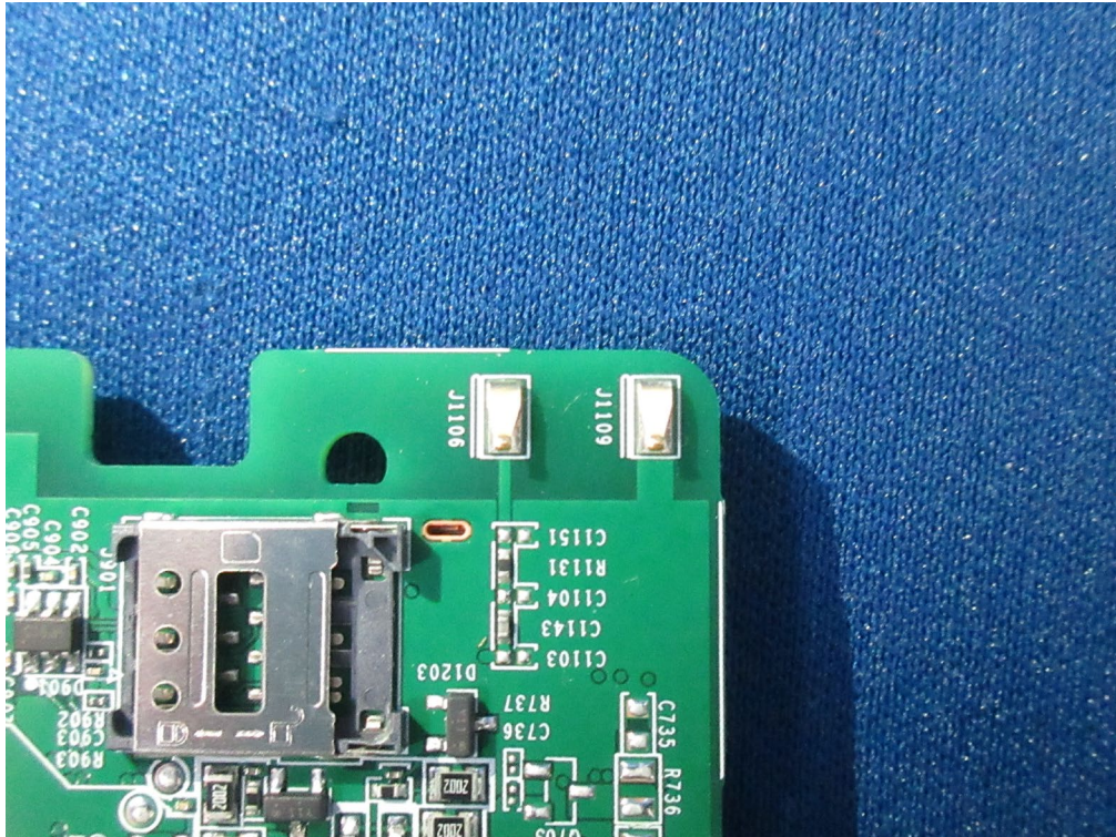
(34) EUT Photo (BT LE+WiFi Antenna)
